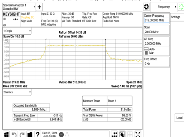
Band26-Part90s 10MHz QPSK RB50 0 CH26740
