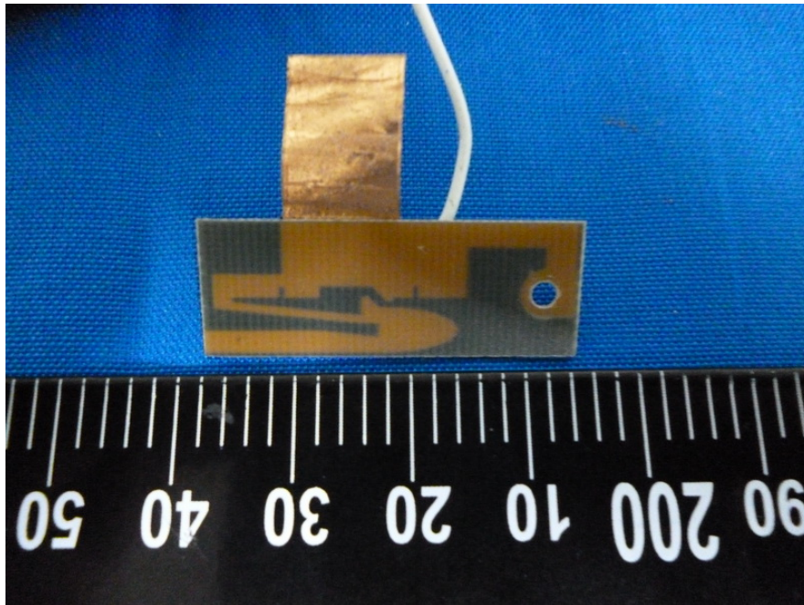
EUT – WIFI AUX Antenna Top View
