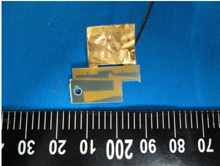
EUT – WIFI Main Antenna Top View
