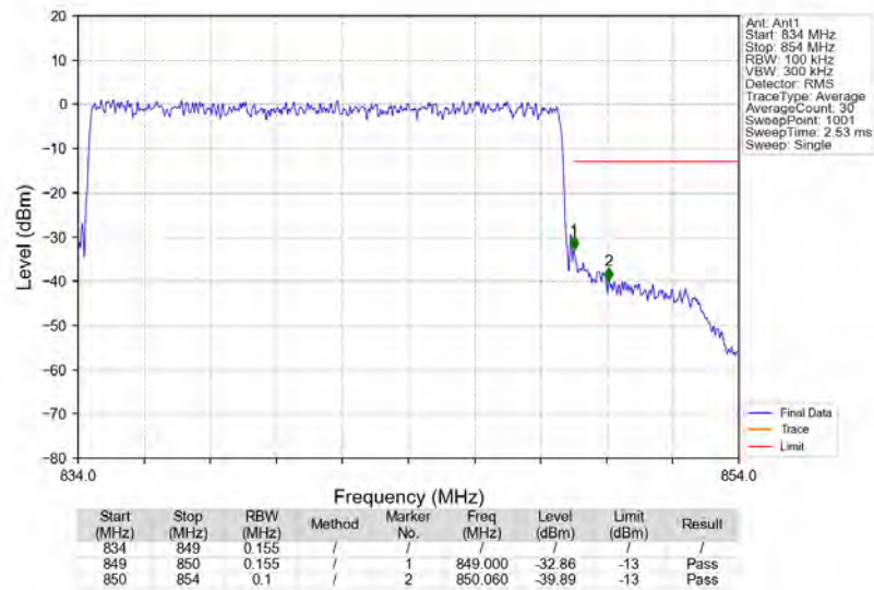
n5_15kHz_SISO_NTNV_15MHz_CP-OFDM_QPSK_841.5MHz_Outer_Full
