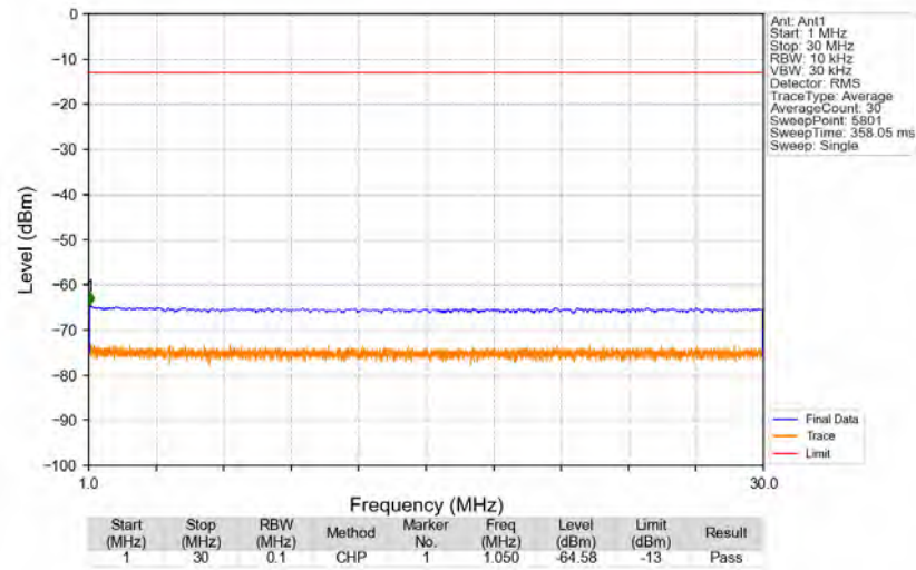
n5_15kHz_SISO_NTNV_10MHz_DFT-s-OFDM PI/2 BPSK 836.5MHz_Edge_1RB_Left
