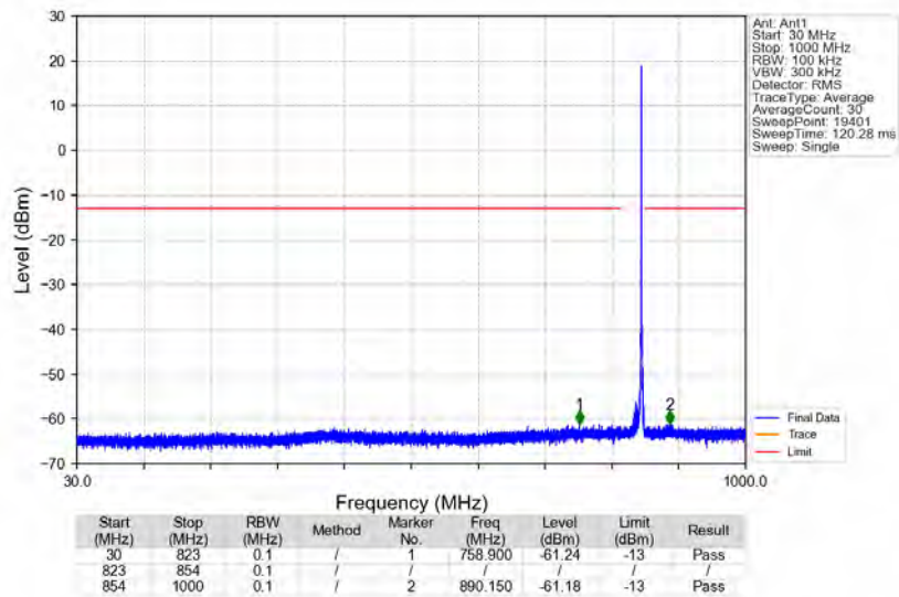
n5_15kHz_SISO_NTNV_10MHz_DFT-s-OFDM_QPSK_844MHz_Edge_1RB_Right
