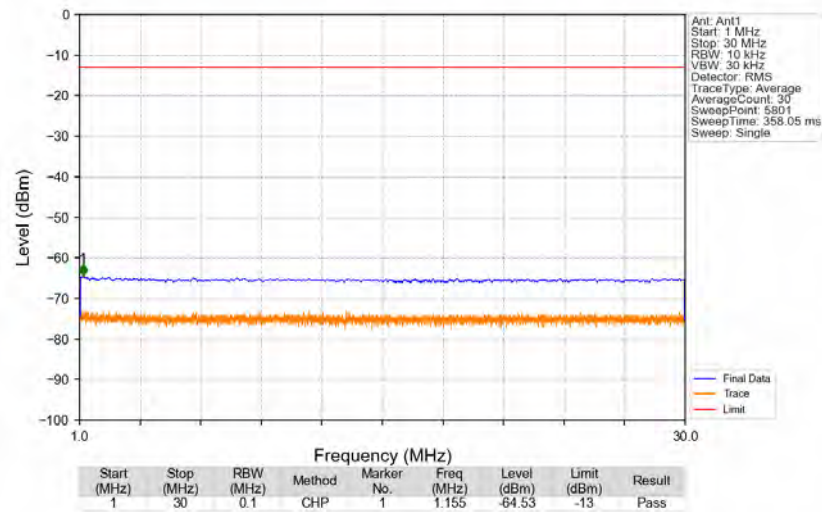
n5_15kHz_SISO_NTNV_10MHz_DFT-s-OFDM_QPSK_836.5MHz_Edge_1RB_Left
