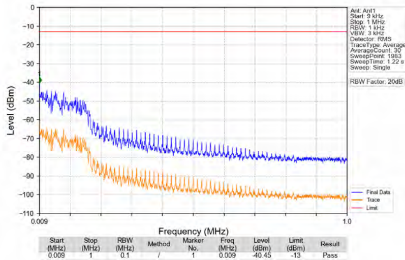
n5_15kHz_SISO_NTNV_15MHz_CP-OFDM_QPSK_831.5MHz_Edge_1RB_Left
