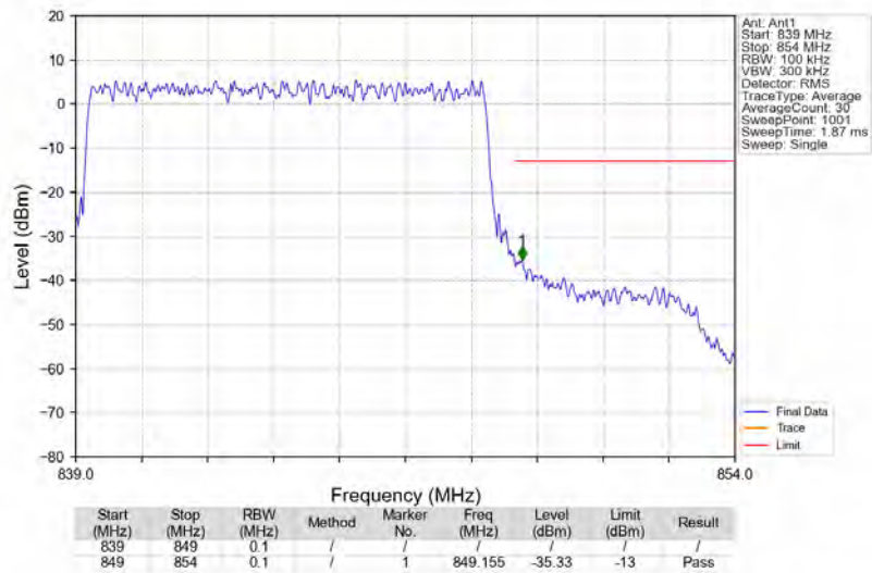
n5_15kHz_SISO_NTNV_10MHz_DFT-s-OFDM_QPSK_844MHz_Outer_Full
