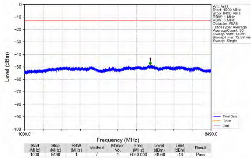
n5_15kHz_SISO_NTNV_10MHz_DFT-s-OFDM_QPSK_844MHz_Edge_1RB_Right
