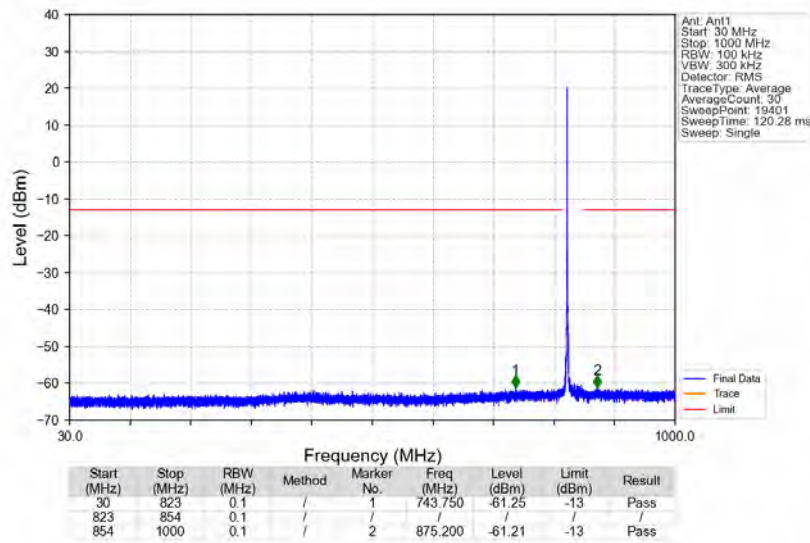
n5_15kHz_SISO_NTNV_20MHz_DFT-s-OFDM_PI/2_BPSK_836.5MHz_Edge_1RB_Left
