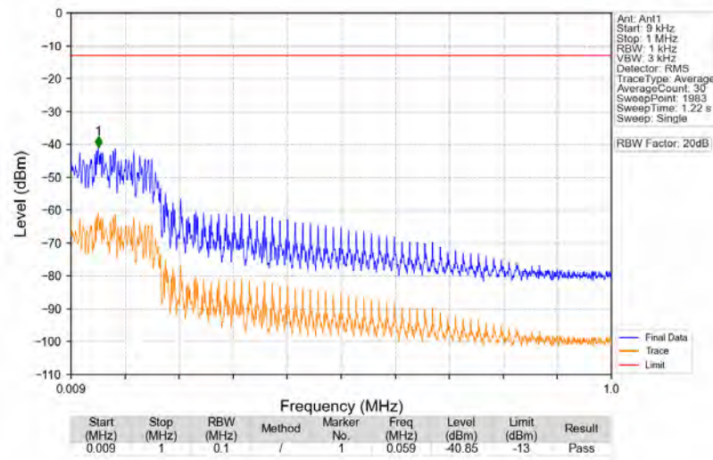
n5_15kHz_SISO_NTNV_20MHz_DFT-s-OFDM_QPSK_836.5MHz_Edge_1RB_Left
