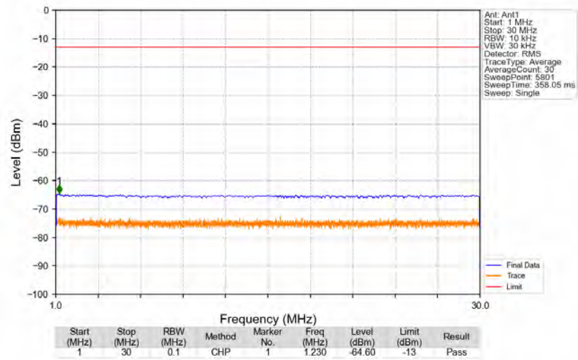
n5_15kHz_SISO_NTNV_10MHz_DFT-s-OFDM PI/2 BPSK_829MHz_Edge_1RB_Left
