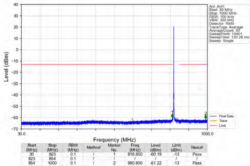
n5_15kHz_SISO_NTNV_15MHz_DFT-s-OFDM_PI/2_BPSK_831.5MHz_Edge_1RB_Left
