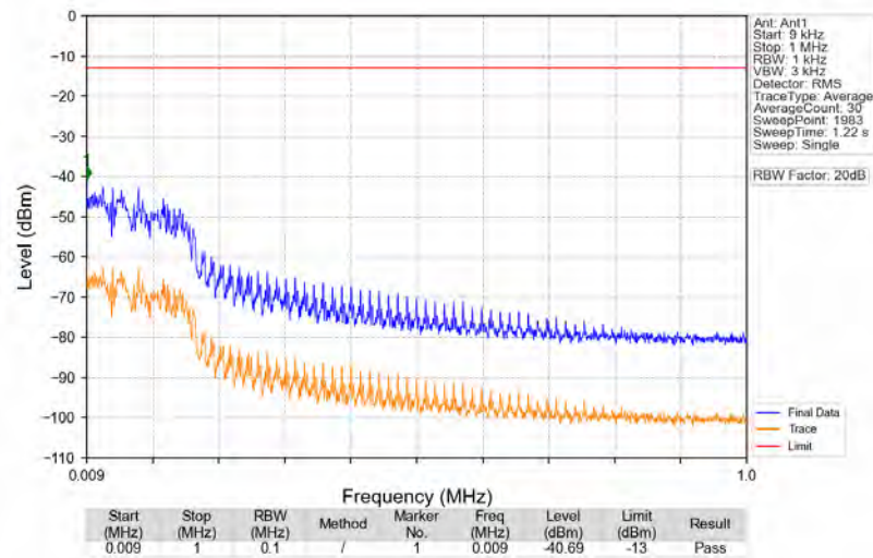
n5_15kHz_SISO_NTNV_15MHz_CP-OFDM_QPSK_841.5MHz_Edge_1RB_Right
