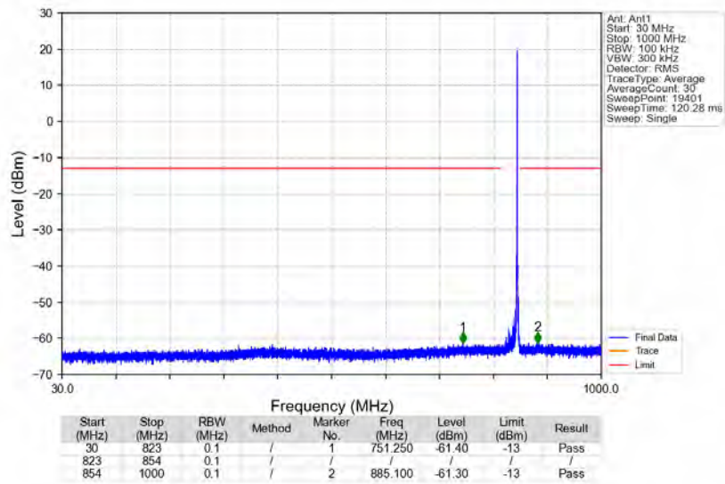
n5_15kHz_SISO_NTNV_15MHz_DFT-s-OFDM_QPSK_841.5MHz_Edge_1RB_Right
