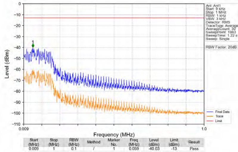
n5_15kHz_SISO_NTNV_15MHz_DFT-s-OFDM_QPSK_836.5MHz_Edge_1RB_Left
