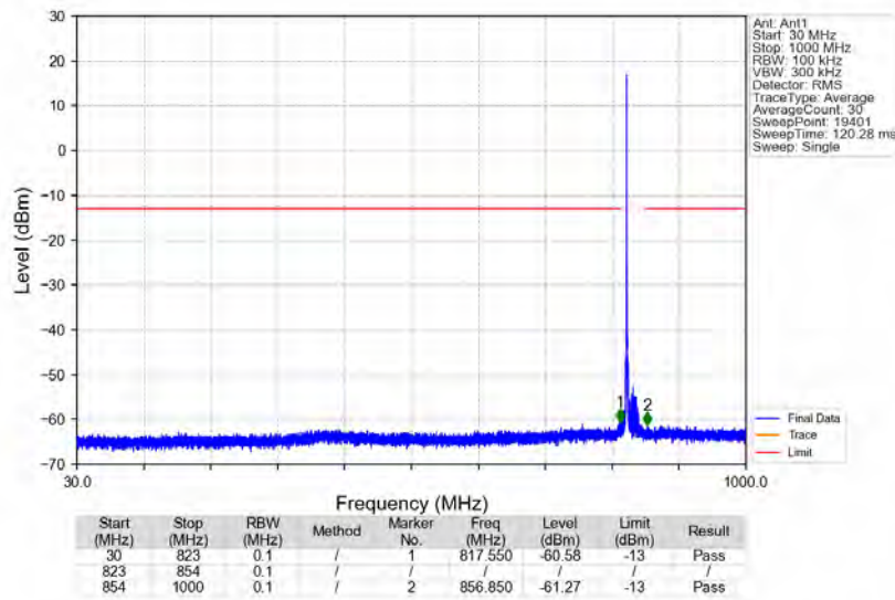
n5_15kHz_SISO_NTNV_20MHz_CP-OFDM_QPSK_836.5MHz_Edge_1RB_Left
