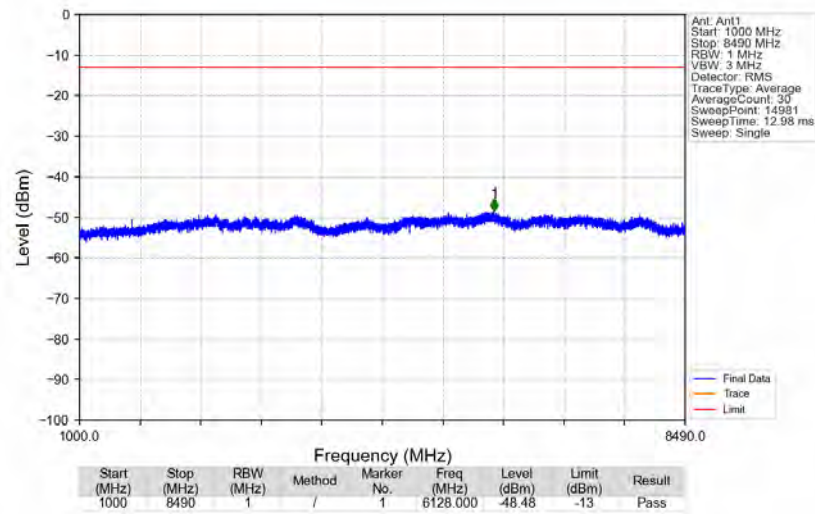
n5_15kHz_SISO_NTNV_15MHz_DFT-s-OFDM_QPSK_831.5MHz_Edge_1RB_Left
