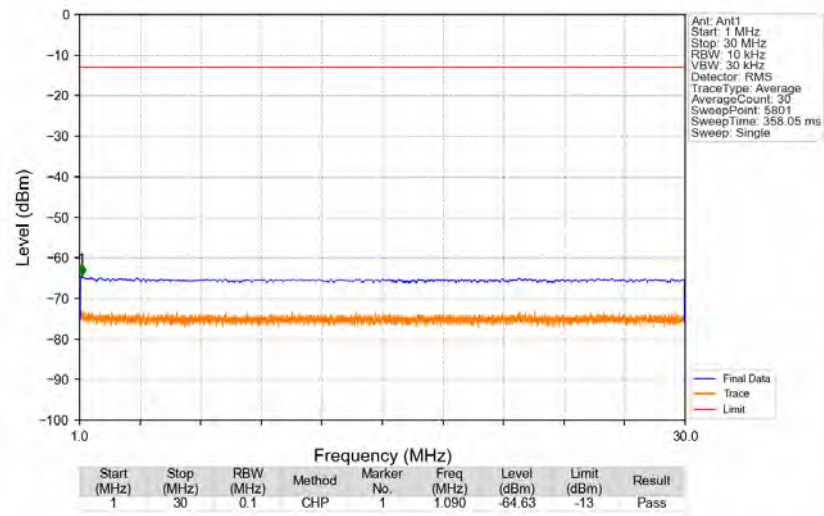
n5_15kHz_SISO_NTNV_15MHz_DFT-s-OFDM PI/2 BPSK_841.5MHz_Edge_1RB_Right
