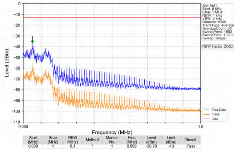
n5_15kHz_SISO_NTNV_20MHz_DFT-s-OFDM PI/2 BPSK 836.5MHz_Edge_1RB_Left
