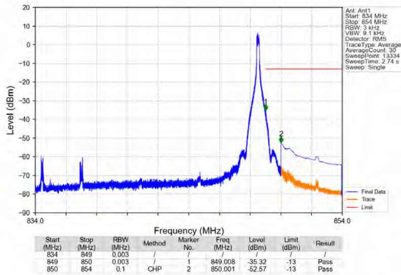
n5_15kHz_SISO_NTNV_15MHz_CP-OFDM_QPSK_841.5MHz_Edge_1RB_Right
