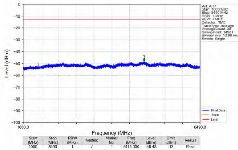
n5_15kHz_SISO_NTNV_10MHz_DFT-s-OFDM_PI/2_BPSK_829MHz_Edge_1RB_Left
