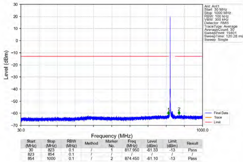
n5_15kHz_SISO_NTNV_20MHz_DFT-s-OFDM_QPSK_836.5MHz_Edge_1RB_Left
