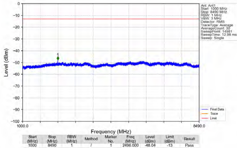
n5_15kHz_SISO_NTNV_10MHz_DFT-s-OFDM_QPSK_836.5MHz_Edge_1RB_Left
