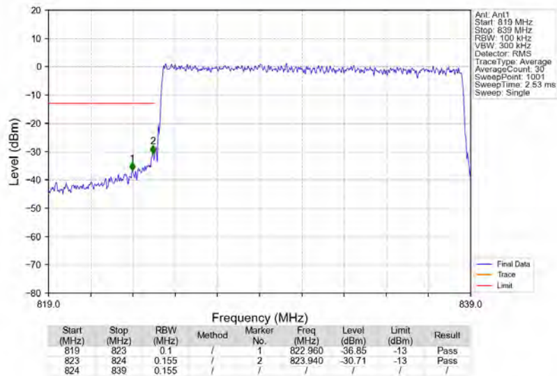
n5_15kHz_SISO_NTNV_15MHz_CP-OFDM_QPSK_831.5MHz_Outer_Full
