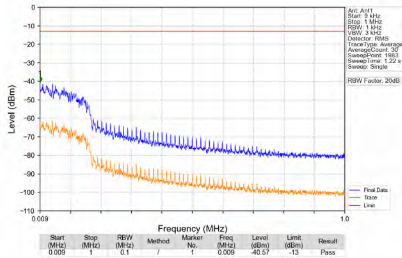
n5_15kHz_SISO_NTNV_15MHz_CP-OFDM_QPSK_836.5MHz_Edge_1RB_Left
