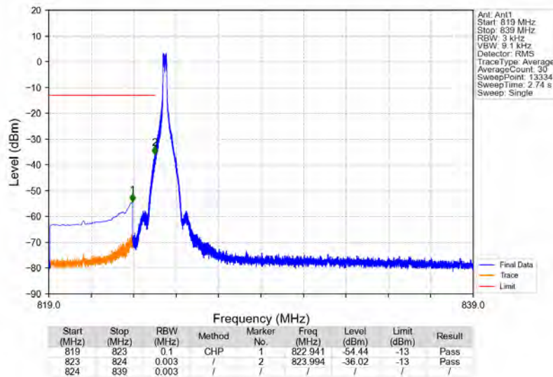
n5_15kHz_SISO_NTNV_15MHz_CP-OFDM_QPSK_831.5MHz_Edge_1RB_Left
