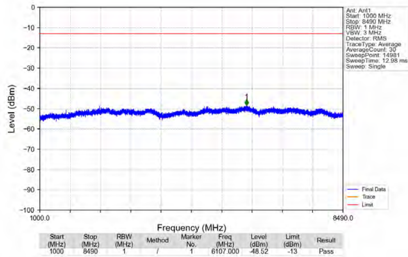
n5_15kHz_SISO_NTNV_15MHz_DFT-s-OFDM_PI/2_BPSK_831.5MHz_Edge_1RB_Left
