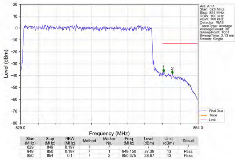
n5_15kHz_SISO_NTNV_20MHz_DFT-s-OFDM_QPSK_839MHz_Outer_Full
