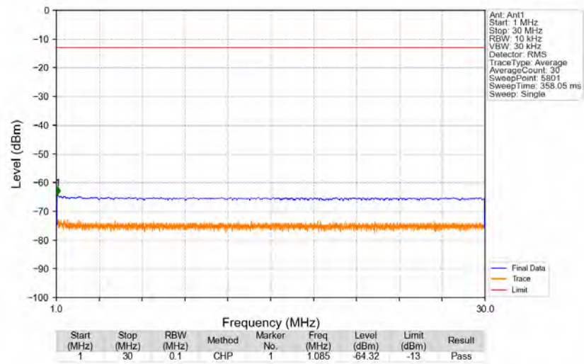
n5_15kHz_SISO_NTNV_5MHz_CP-OFDM_QPSK_846.5MHz_Edge_1RB_Right
