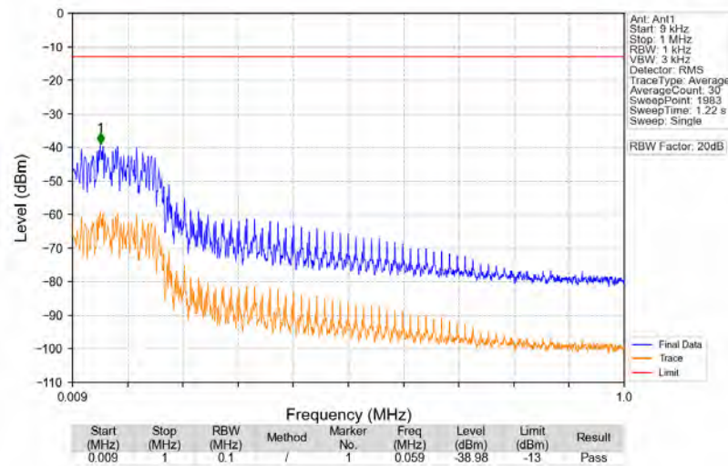
n5_15kHz_SISO_NTNV_15MHz_DFT-s-OFDM_QPSK_831.5MHz_Edge_1RB_Left
