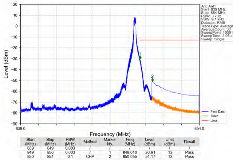
n5_15kHz_SISO_NTNV_10MHz_DFT-s-OFDM_QPSK_844MHz_Edge_1RB_Right
