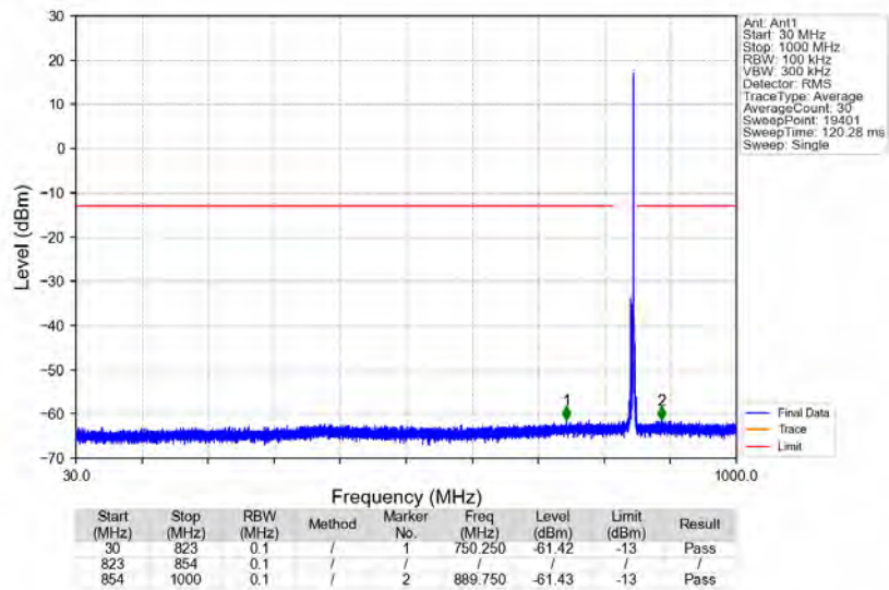
n5_15kHz_SISO_NTNV_5MHz_CP-OFDM_QPSK_846.5MHz_Edge_1RB_Right
