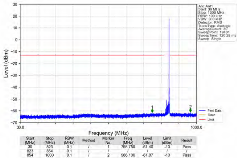
n5_15kHz_SISO_NTNV_15MHz_CP-OFDM_QPSK_841.5MHz_Edge_1RB_Right
