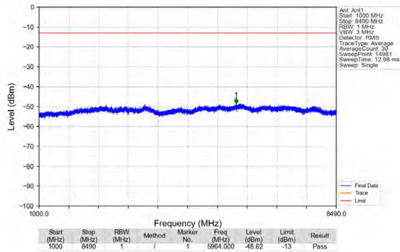
n5_15kHz_SISO_NTNV_15MHz_DFT-s-OFDM_PI/2_BPSK_841.5MHz_Edge_1RB_Right
