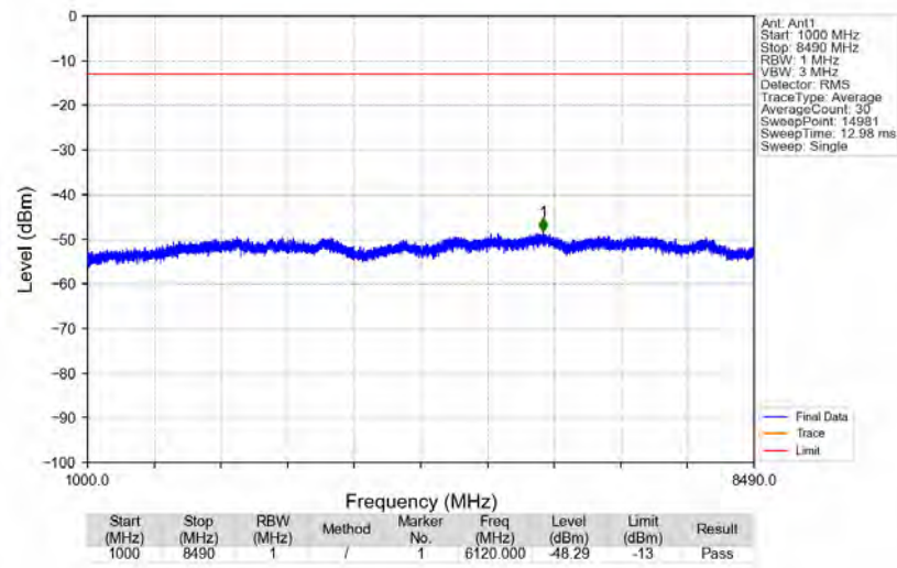
n5_15kHz_SISO_NTNV_20MHz_CP-OFDM_QPSK_834MHz_Edge_1RB_Left
