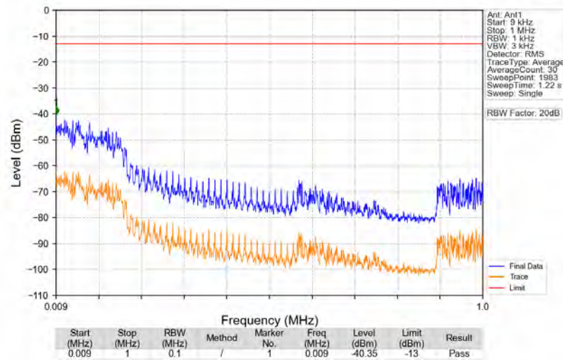
n5_15kHz_SISO_NTNV_10MHz_CP-OFDM_QPSK_829MHz_Edge_1RB_Left
