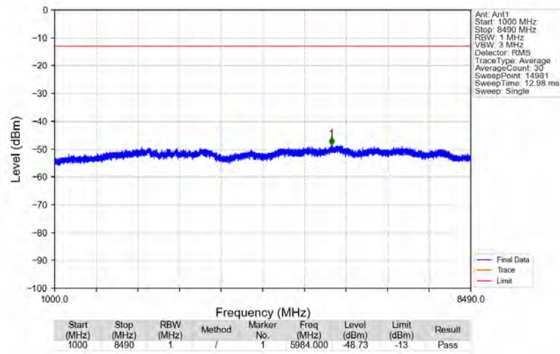
n5_15kHz_SISO_NTNV_15MHz_CP-OFDM_QPSK_831.5MHz_Edge_1RB_Left
