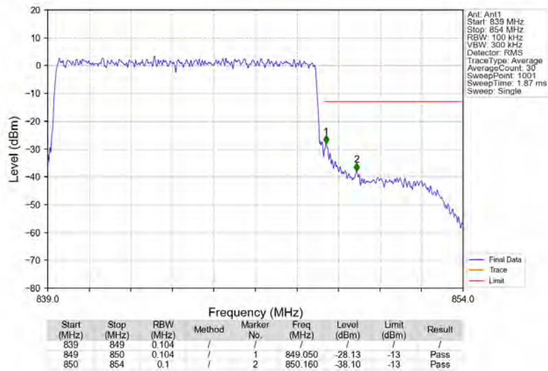
n5_15kHz_SISO_NTNV_10MHz_CP-OFDM_QPSK_844MHz_Outer_Full
