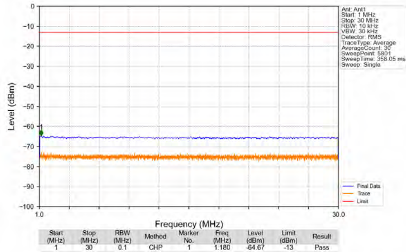
n5_15kHz_SISO_NTNV_15MHz_DFT-s-OFDM_QPSK_836.5MHz_Edge_1RB_Left
