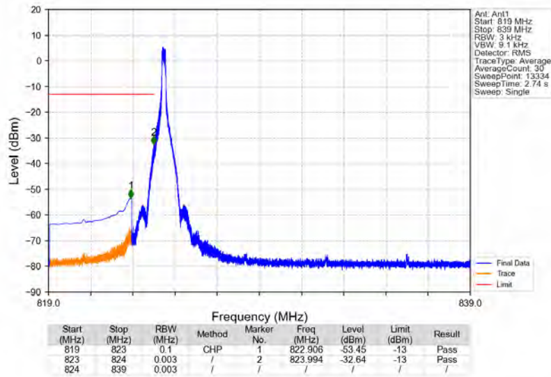
n5_15kHz_SISO_NTNV_15MHz_DFT-s-OFDM PI/2 BPSK_831.5MHz_Edge_1RB_Left
