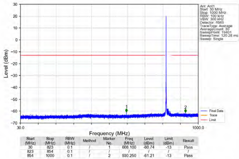
n5_15kHz_SISO_NTNV_20MHz_DFT-s-OFDM_QPSK_834MHz_Edge_1RB_Left
