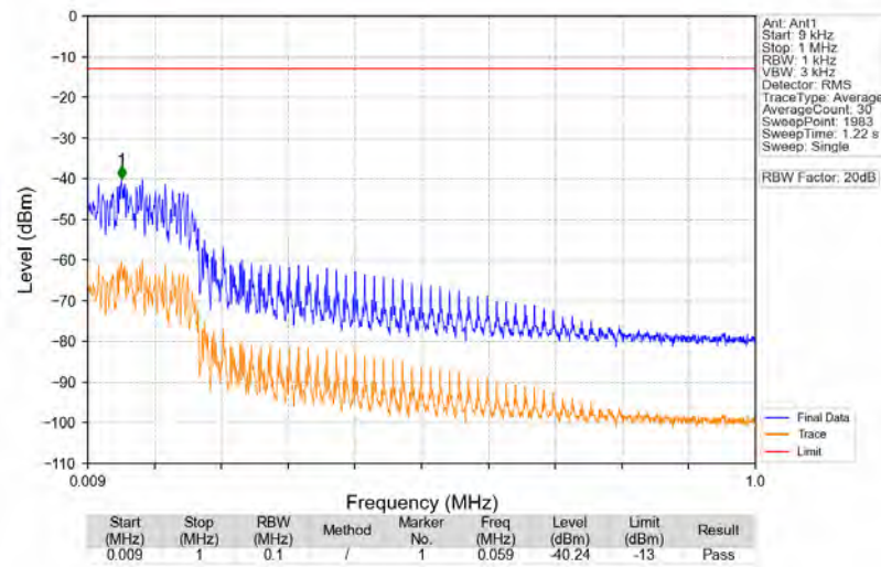
n5_15kHz_SISO_NTNV_10MHz_DFT-s-OFDM_QPSK_836.5MHz_Edge_1RB_Left
