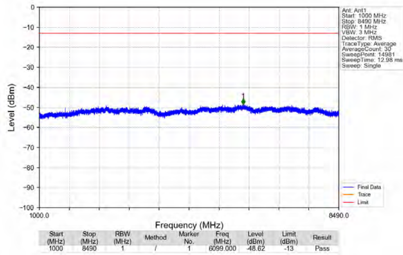
n5_15kHz_SISO_NTNV_20MHz_DFT-s-OFDM_PI/2_BPSK_834MHz_Edge_1RB_Left
