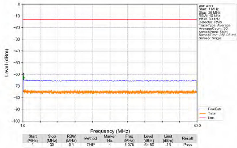
n5_15kHz_SISO_NTNV_20MHz_CP-OFDM_QPSK_839MHz_Edge_1RB_Right
