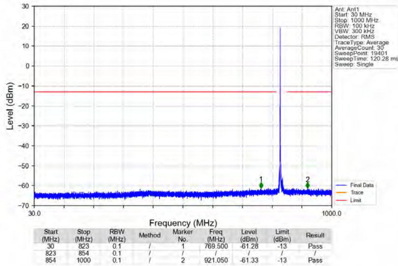
n5_15kHz_SISO_NTNV_10MHz_DFT-s-OFDM_QPSK_836.5MHz_Edge_1RB_Left
