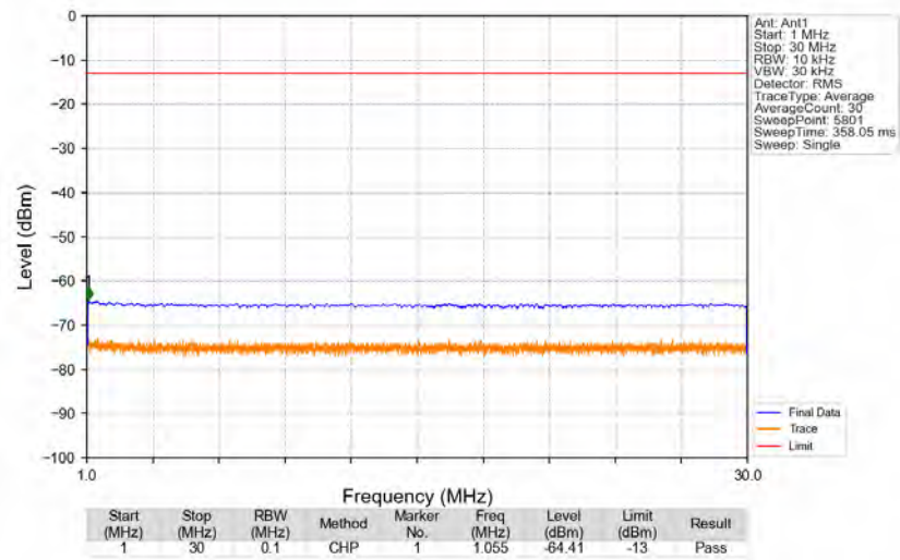
n5_15kHz_SISO_NTNV_10MHz_CP-OFDM_QPSK_829MHz_Edge_1RB_Left
