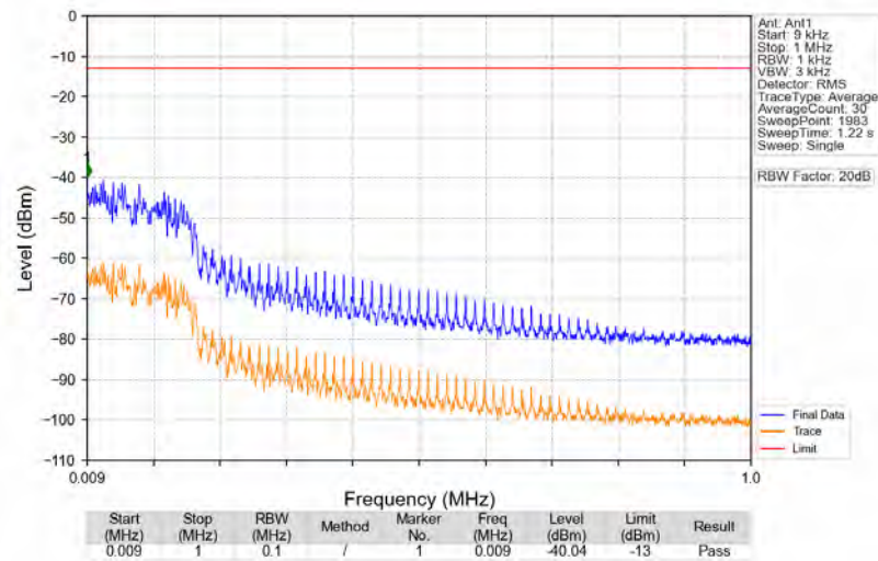
n5_15kHz_SISO_NTNV_20MHz_CP-OFDM_QPSK_834MHz_Edge_1RB_Left
