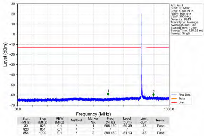
n5 15kHz_SISO_NTNV_20MHz_DFT-s-OFDM PI/2 BPSK_834MHz_Edge_1RB_Left
