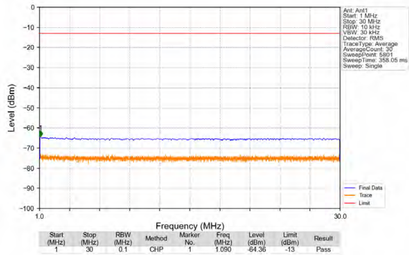
n5_15kHz_SISO_NTNV_10MHz_DFT-s-OFDM_QPSK_829MHz_Edge_1RB_Left
