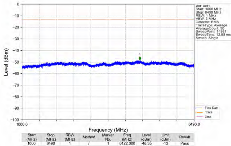
n5_15kHz_SISO_NTNV_20MHz_CP-OFDM_QPSK_836.5MHz_Edge_1RB_Left
