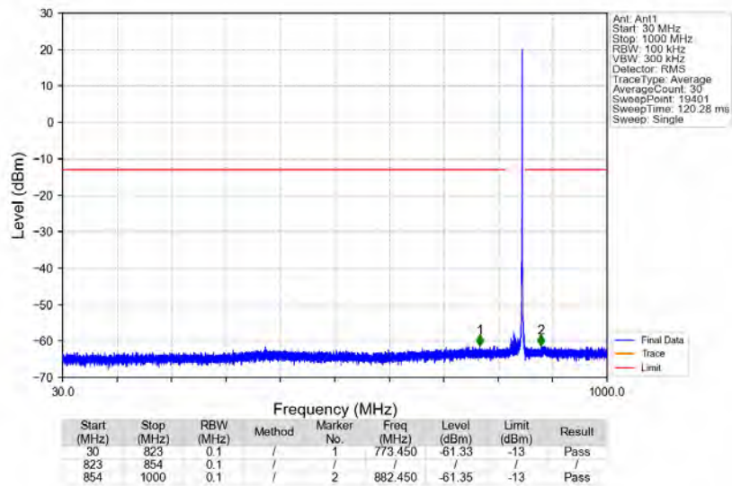
n5_15kHz_SISO_NTNV_15MHz_DFT-s-OFDM PI/2 BPSK_841.5MHz_Edge_1RB_Right
