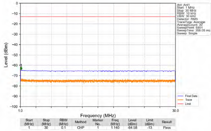
n5_15kHz_SISO_NTNV_20MHz_DFT-s-OFDM_QPSK_834MHz_Edge_1RB_Left
