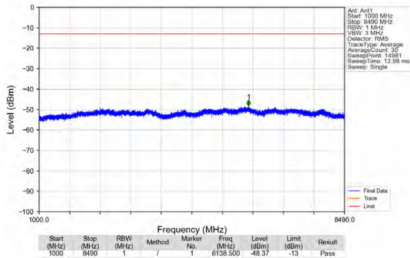
n5_15kHz_SISO_NTNV_10MHz_CP-OFDM_QPSK_836.5MHz_Edge_1RB_Left
