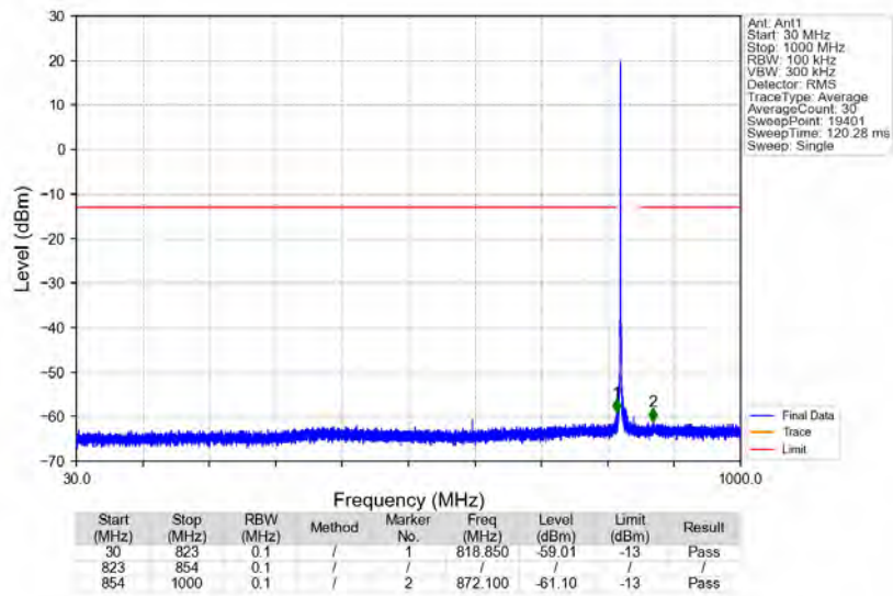
n5_15kHz_SISO_NTNV_15MHz_DFT-s-OFDM_QPSK_831.5MHz_Edge_1RB_Left
