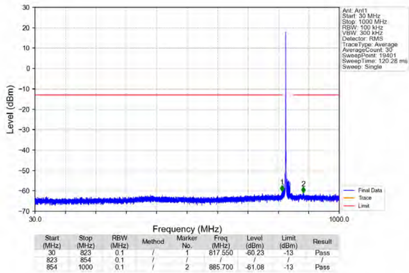
n5_15kHz_SISO_NTNV_15MHz_CP-OFDM_QPSK_836.5MHz_Edge_1RB_Left
