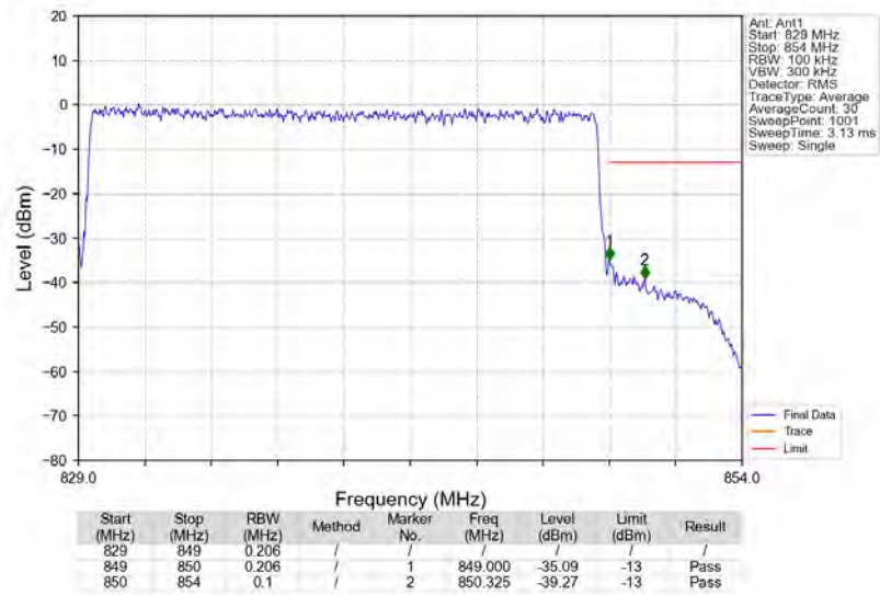
n5_15kHz_SISO_NTNV_20MHz_CP-OFDM_QPSK_839MHz_Outer_Full
