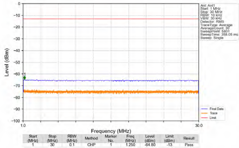
n5_15kHz_SISO_NTNV_15MHz_CP-OFDM_QPSK_841.5MHz_Edge_1RB_Right
