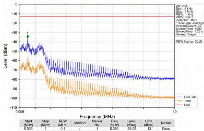
n5_15kHz_SISO_NTNV_15MHz_DFT-s-OFDM PI/2 BPSK_831.5MHz_Edge_1RB_Left
