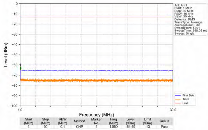
n5_15kHz_SISO_NTNV_15MHz_DFT-s-OFDM_PI/2_BPSK_831.5MHz_Edge_1RB_Left
