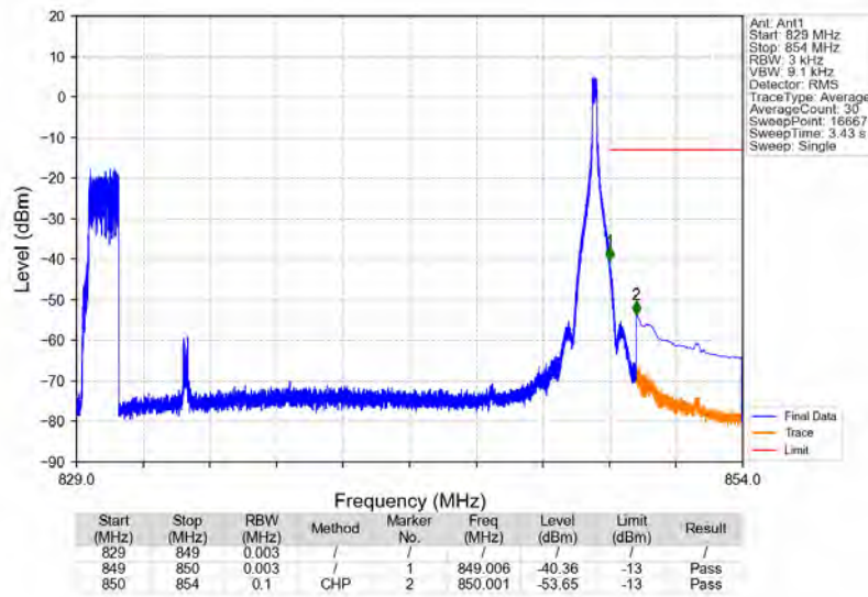
n5_15kHz_SISO_NTNV_20MHz_CP-OFDM_QPSK_839MHz_Edge_1RB_Right
