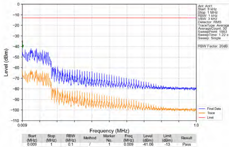
n5_15kHz_SISO_NTNV_10MHz_DFT-s-OFDM_QPSK_844MHz_Edge_1RB_Right
