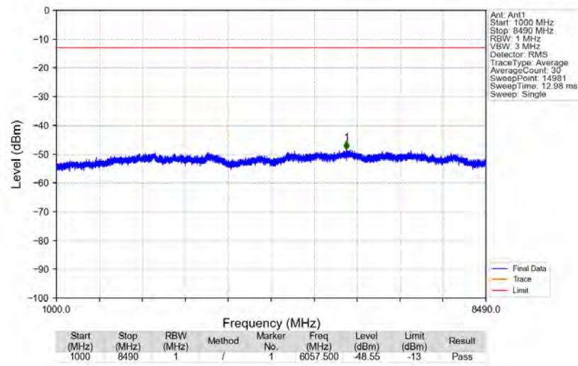
n5_15kHz_SISO_NTNV_20MHz_DFT-s-OFDM_QPSK_839MHz_Edge_1RB_Right
