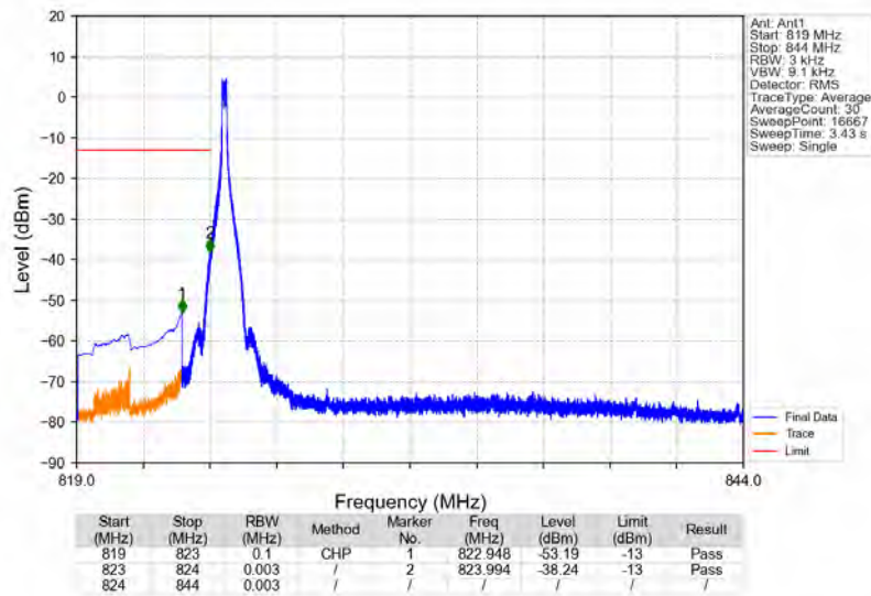
n5_15kHz_SISO_NTNV_20MHz_CP-OFDM_QPSK_834MHz_Edge_1RB_Left
