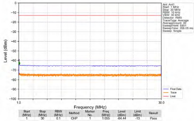
n5_15kHz_SISO_NTNV_10MHz_DFT-s-OFDM_QPSK_844MHz_Edge_1RB_Right
