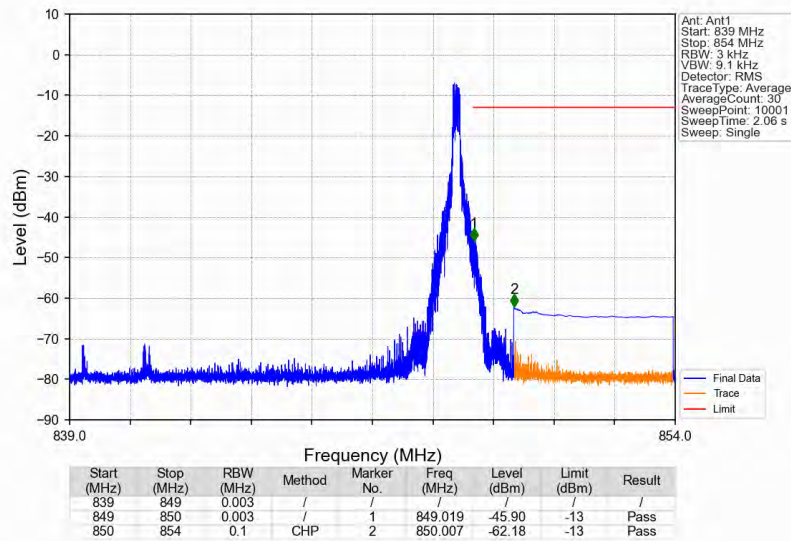
n5_15kHz_SISO_NTNV_10MHz_CP-OFDM_QPSK_844MHz_Edge_1RB_Right
