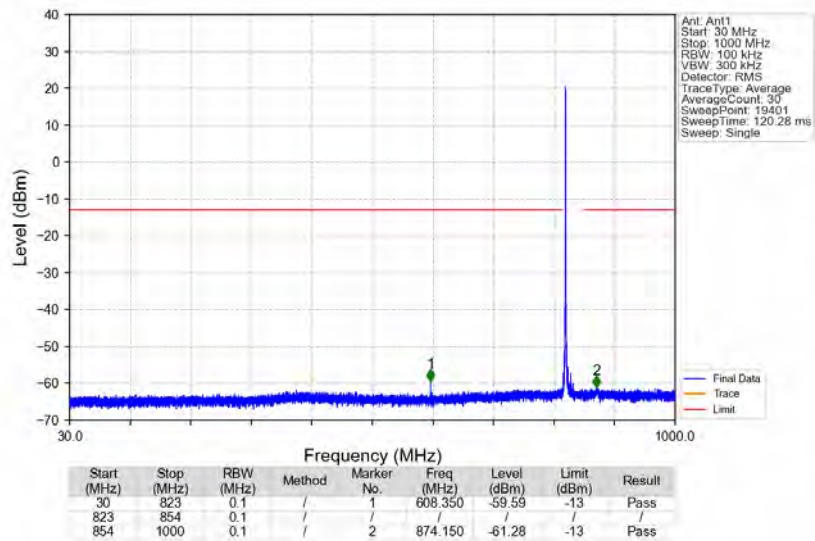
n5_15kHz_SISO_NTNV_10MHz_DFT-s-OFDM PI/2 BPSK_829MHz_Edge_1RB_Left
