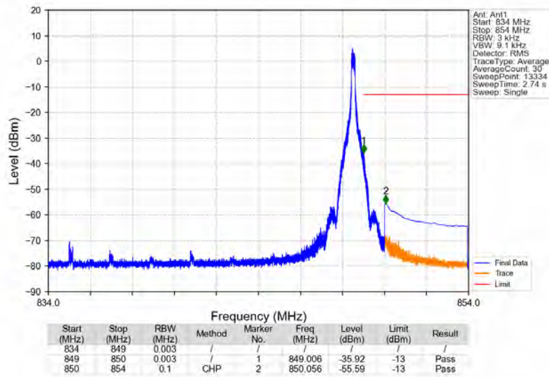
n5_15kHz_SISO_NTNV_15MHz_DFT-s-OFDM PI/2 BPSK_841.5MHz_Edge_1RB_Right
