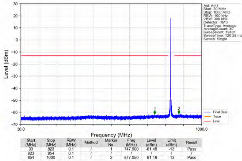
n5_15kHz_SISO_NTNV_10MHz_CP-OFDM_QPSK_836.5MHz_Edge_1RB_Left
