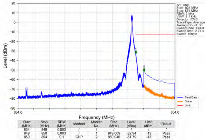
n5_15kHz_SISO_NTNV_15MHz_DFT-s-OFDM QPSK 841.5MHz_Edge_1RB_Right
