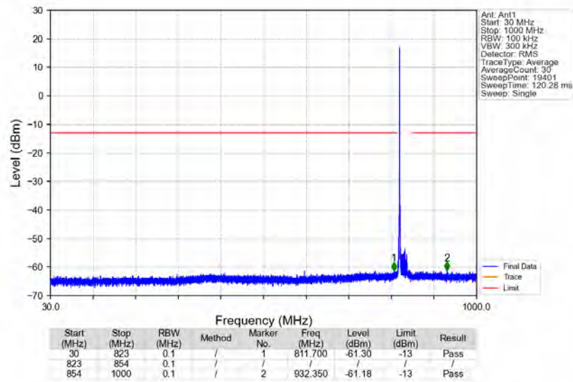
n5_15kHz_SISO_NTNV_20MHz_CP-OFDM_QPSK_834MHz_Edge_1RB_Left
