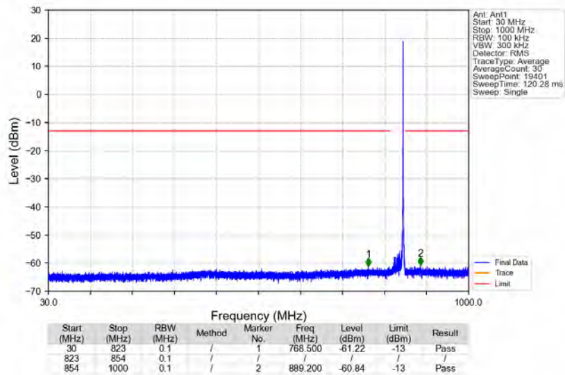
n5_15kHz_SISO_NTNV_20MHz_DFT-s-OFDM_QPSK_839MHz_Edge_1RB_Right
