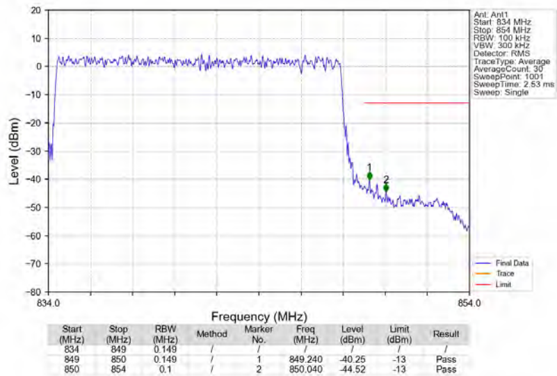
n5_15kHz_SISO_NTNV_15MHz_DFT-s-OFDM_PI/2_BPSK_841.5MHz_Outer_Full
