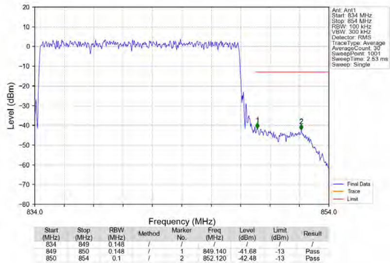
n5_15kHz_SISO_NTNV_15MHz_DFT-s-OFDM_QPSK_841.5MHz_Outer_Full
