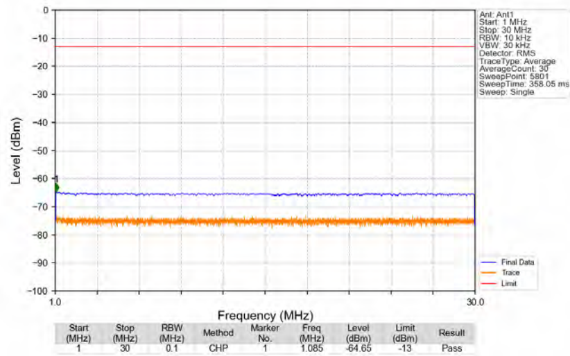
n5_15kHz_SISO_NTNV_15MHz_DFT-s-OFDM PI/2 BPSK 836.5MHz_Edge_1RB_Left
