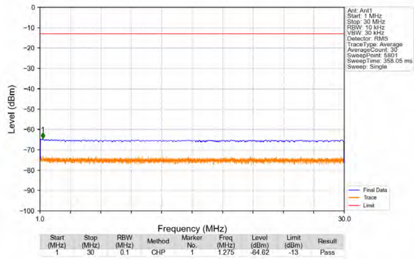
n5_15kHz_SISO_NTNV_15MHz_CP-OFDM_QPSK_831.5MHz_Edge_1RB_Left
