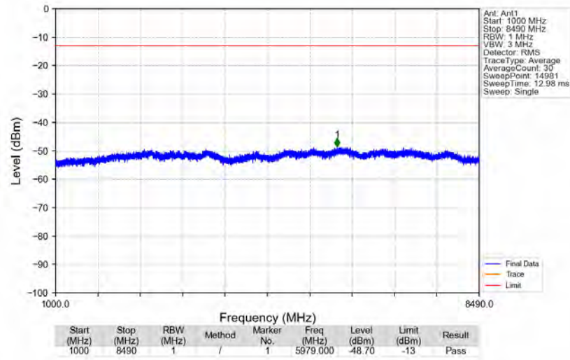
n5_15kHz_SISO_NTNV_20MHz_CP-OFDM_QPSK_839MHz_Edge_1RB_Right
