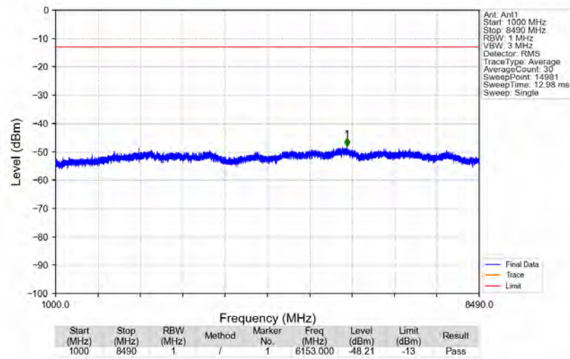
n5_15kHz_SISO_NTNV_10MHz_DFT-s-OFDM_QPSK_829MHz_Edge_1RB_Left
