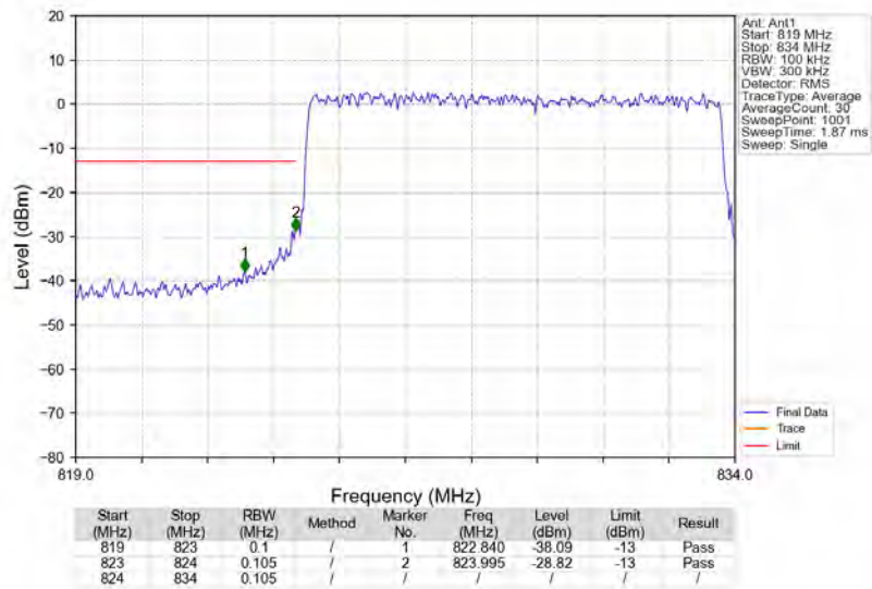
n5_15kHz_SISO_NTNV_10MHz_CP-OFDM_QPSK_829MHz_Outer_Full
