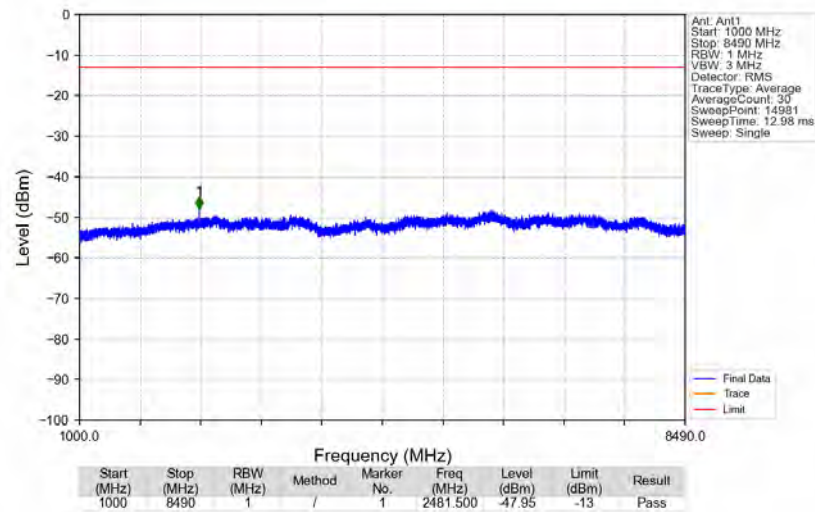
n5_15kHz_SISO_NTNV_20MHz_DFT-s-OFDM_PI/2_BPSK_836.5MHz_Edge_1RB_Left
