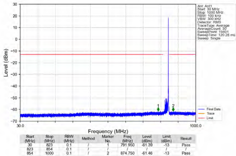
n5_15kHz_SISO_NTNV_20MHz_CP-OFDM_QPSK_839MHz_Edge_1RB_Right
