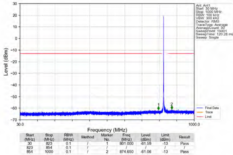
n5_15kHz_SISO_NTNV_15MHz_DFT-s-OFDM_QPSK_836.5MHz_Edge_1RB_Left
