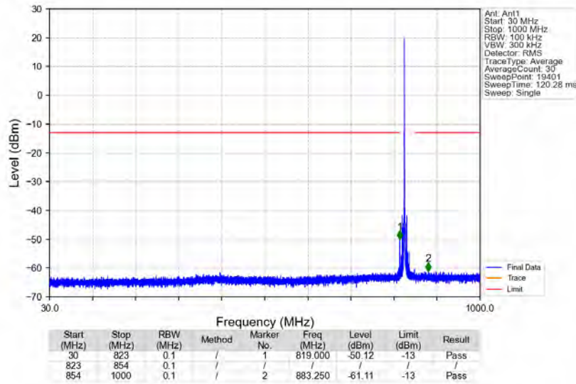
n5_15kHz_SISO_NTNV_15MHz_DFT-s-OFDM_PI/2_BPSK_836.5MHz_Edge_1RB_Left
