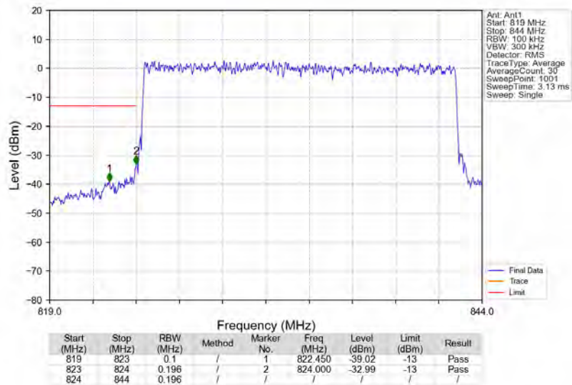
n5_15kHz_SISO_NTNV_20MHz_DFT-s-OFDM_QPSK_834MHz_Outer_Full
