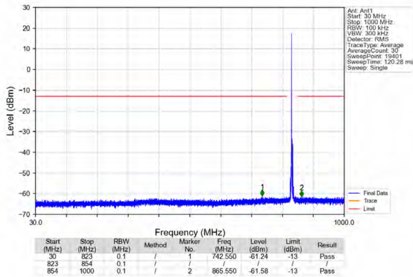
n5_15kHz_SISO_NTNV_5MHz_CP-OFDM_QPSK_836.5MHz_Edge_1RB_Left
