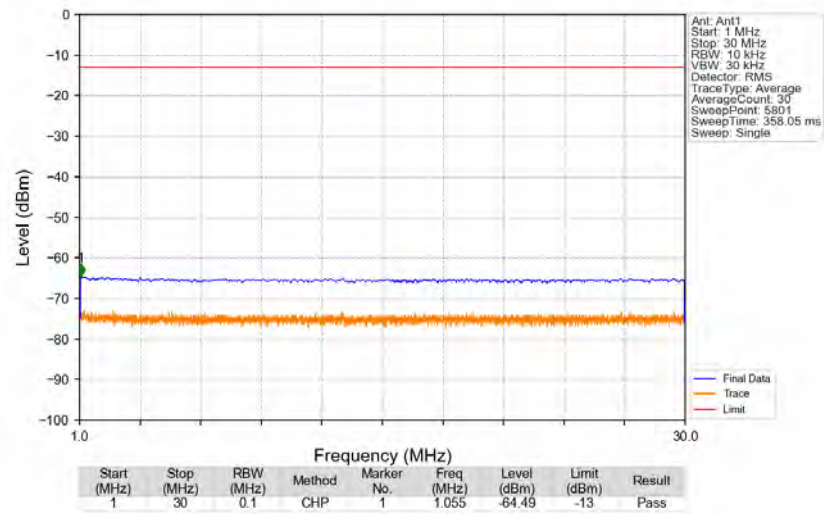
n5_15kHz_SISO_NTNV_15MHz_DFT-s-OFDM_QPSK_831.5MHz_Edge_1RB_Left
