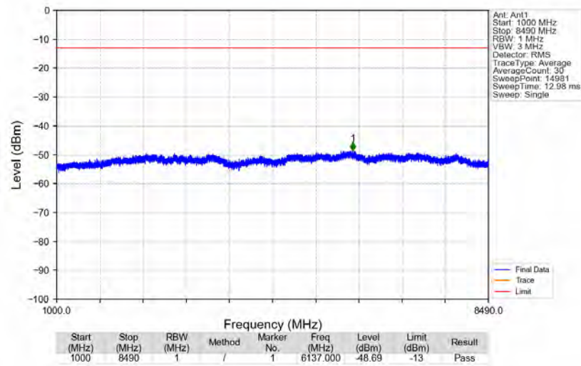
n5_15kHz_SISO_NTNV_10MHz_DFT-s-OFDM_PI/2_BPSK_844MHz_Edge_1RB_Right
