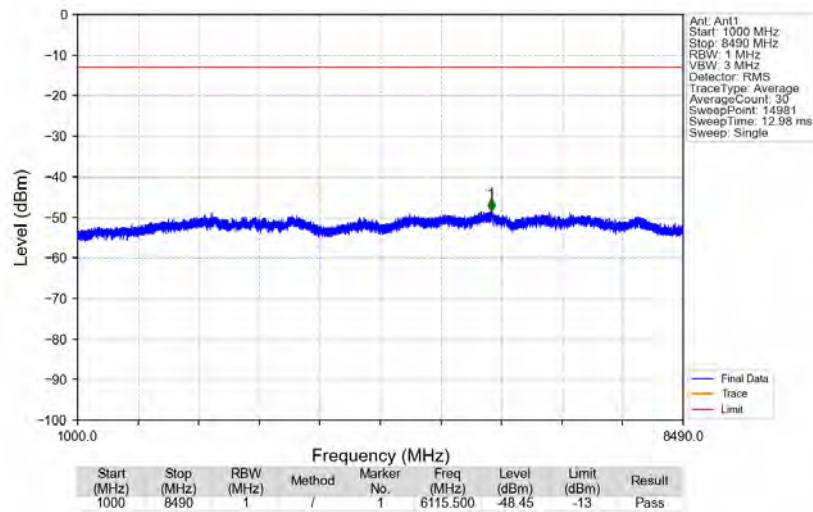
n5_15kHz_SISO_NTNV_5MHz_CP-OFDM_QPSK_836.5MHz_Edge_1RB_Left
