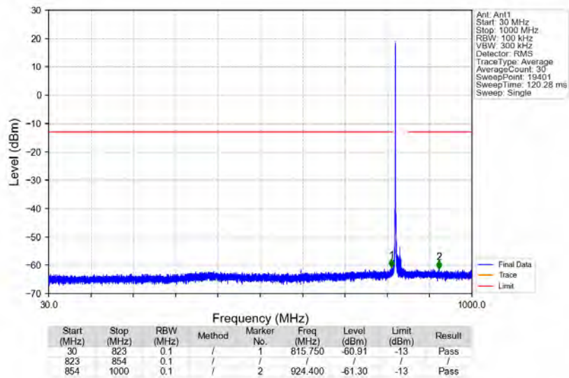
n5_15kHz_SISO_NTNV_15MHz_CP-OFDM_QPSK_831.5MHz_Edge_1RB_Left
