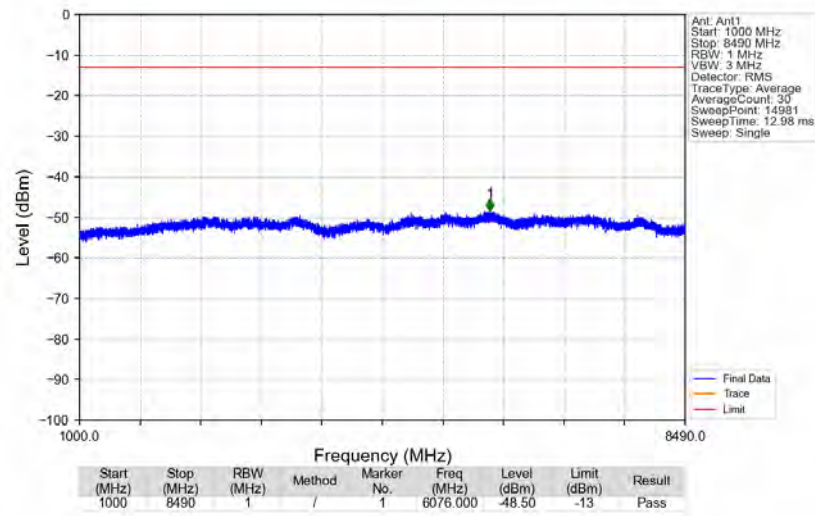
n5_15kHz_SISO_NTNV_15MHz_CP-OFDM_QPSK_841.5MHz_Edge_1RB_Right
