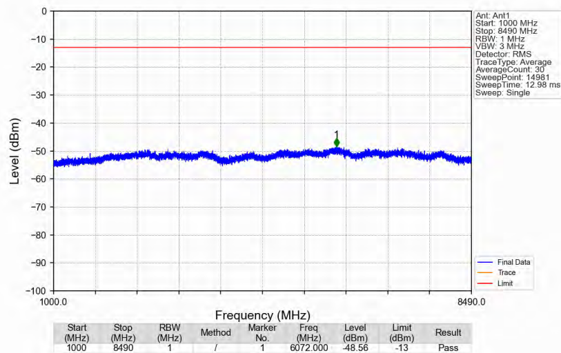
n5_15kHz_SISO_NTNV_20MHz_DFT-s-OFDM_QPSK_836.5MHz_Edge_1RB_Left
