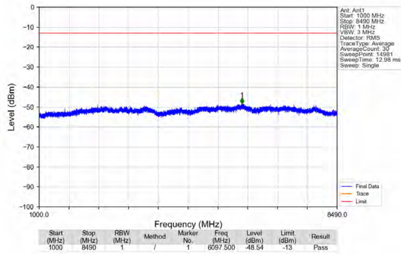
n5_15kHz_SISO_NTNV_20MHz_DFT-s-OFDM_QPSK_834MHz_Edge_1RB_Left
