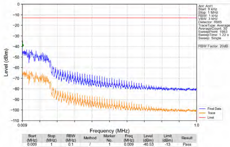
n5_15kHz_SISO_NTNV_10MHz_CP-OFDM_QPSK_844MHz_Edge_1RB_Right
