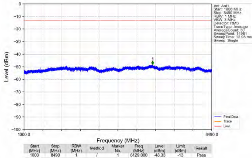
n5_15kHz_SISO_NTNV_15MHz_DFT-s-OFDM_PI/2_BPSK_836.5MHz_Edge_1RB_Left
