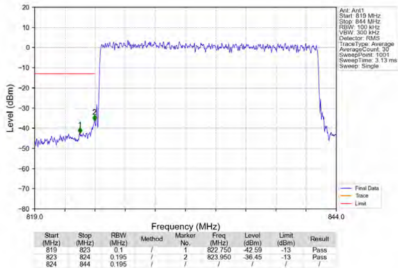
n5_15kHz_SISO_NTNV_20MHz_DFT-s-OFDM_PI/2_BPSK_834MHz_Outer_Full
