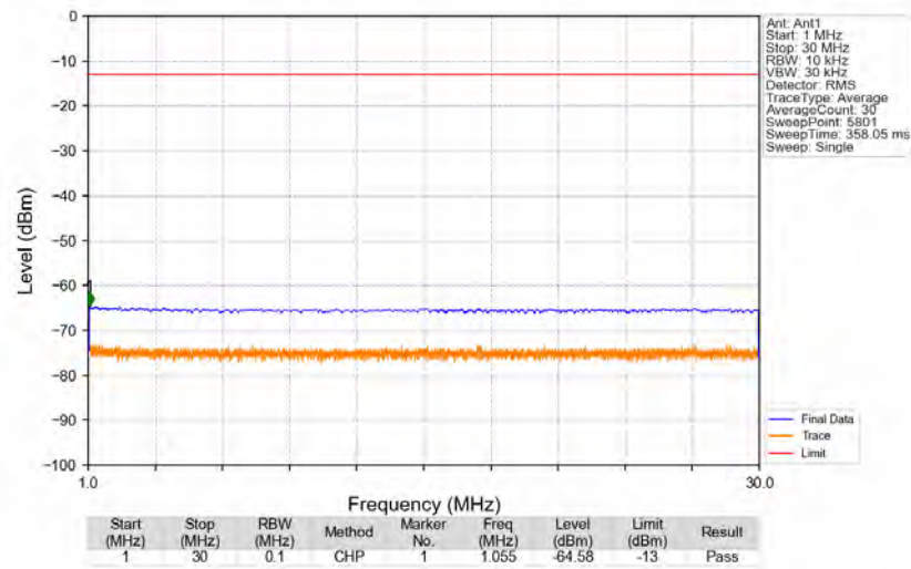
n5_15kHz_SISO_NTNV_20MHz_DFT-s-OFDM_QPSK_836.5MHz_Edge_1RB_Left
