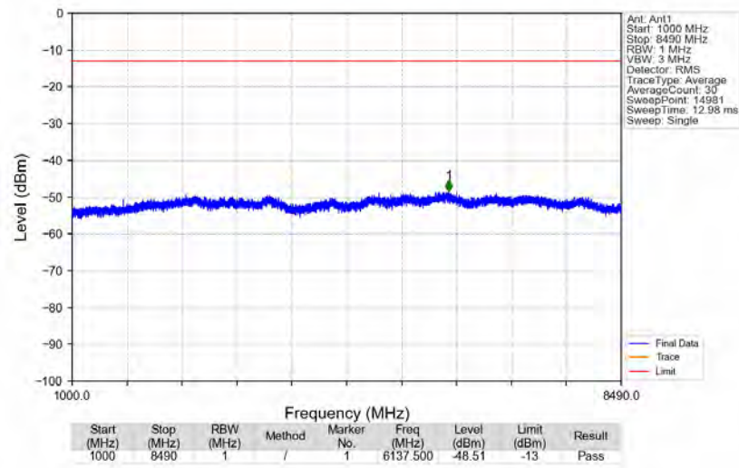
n5_15kHz_SISO_NTNV_15MHz_DFT-s-OFDM_QPSK_841.5MHz_Edge_1RB_Right
