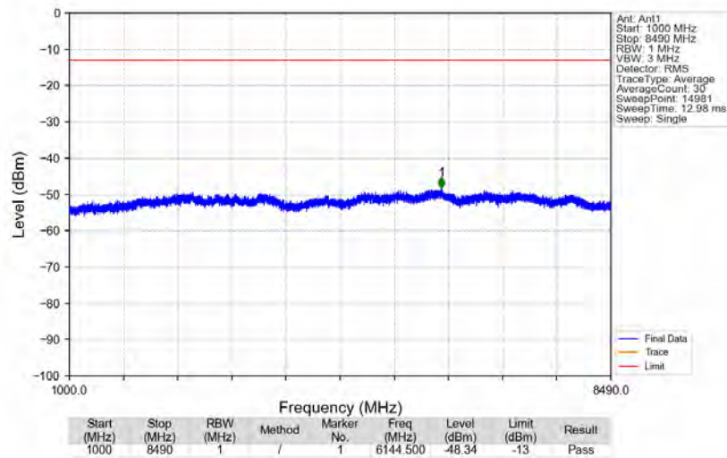
n5_15kHz_SISO_NTNV_15MHz_CP-OFDM_QPSK_836.5MHz_Edge_1RB_Left
