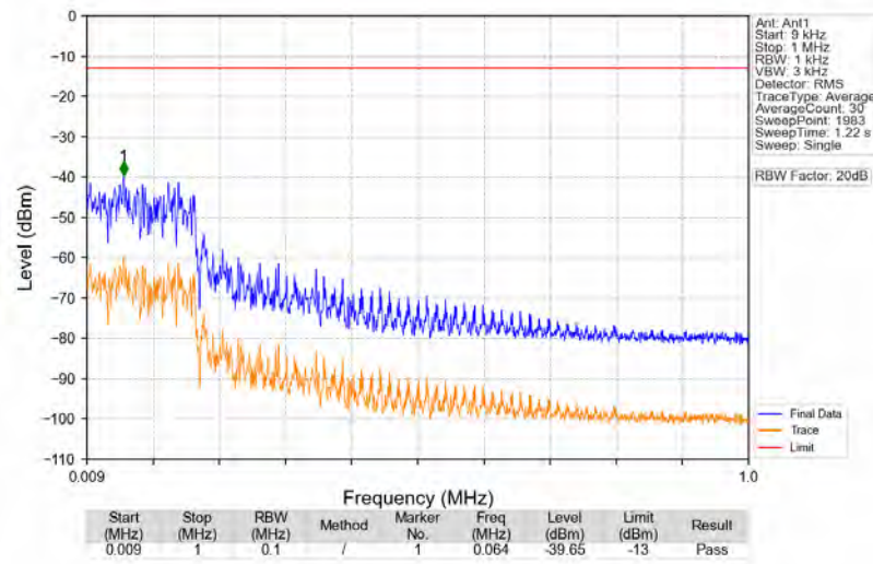
n5_15kHz_SISO_NTNV_15MHz_DFT-s-OFDM PI/2 BPSK 836.5MHz_Edge_1RB_Left
