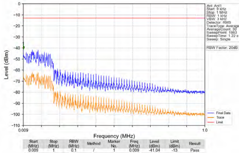
n5_15kHz_SISO_NTNV_20MHz_DFT-s-OFDM_QPSK_839MHz_Edge_1RB_Right
