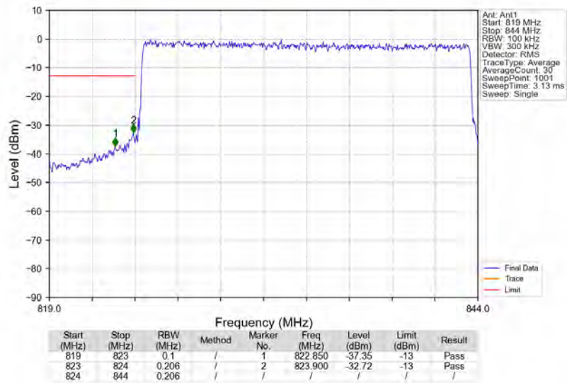
n5_15kHz_SISO_NTNV_20MHz_CP-OFDM_QPSK_834MHz_Outer_Full
