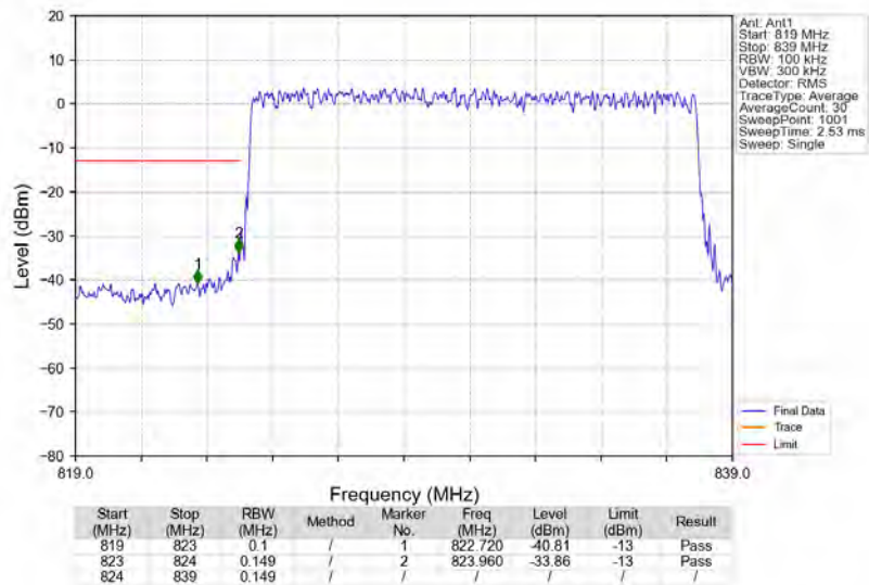
n5_15kHz_SISO_NTNV_15MHz_DFT-s-OFDM_QPSK_831.5MHz_Outer_Full
