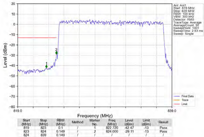
n5_15kHz_SISO_NTNV_15MHz_DFT-s-OFDM_PI/2_BPSK_831.5MHz_Outer_Full
