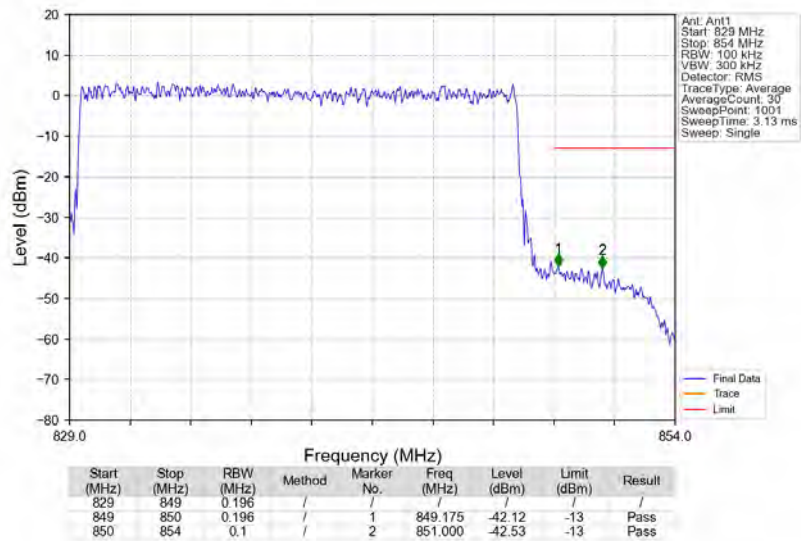
n5_15kHz_SISO_NTNV_20MHz_DFT-s-OFDM_PI/2_BPSK_839MHz_Outer_Full
