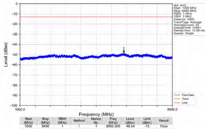
n5_15kHz_SISO_NTNV_10MHz_CP-OFDM_QPSK_829MHz_Edge_1RB_Left
