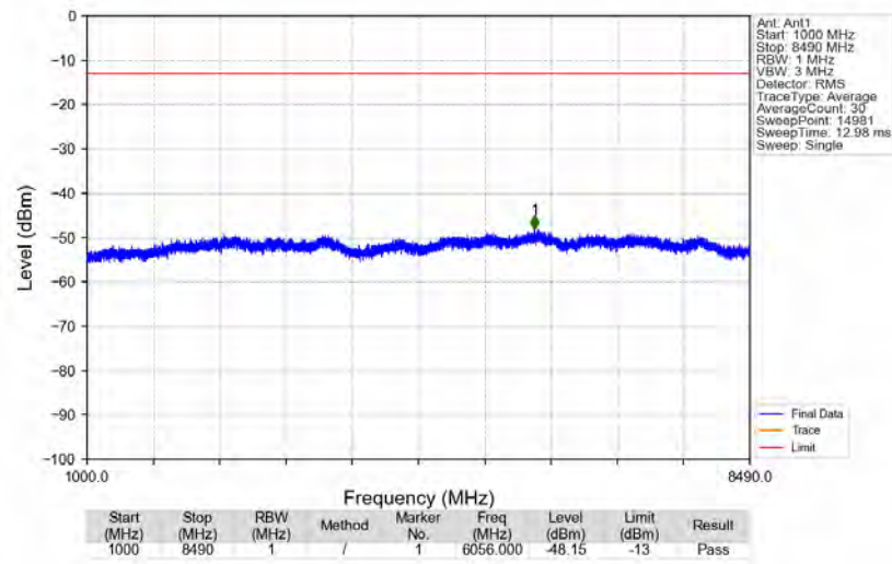
n5_15kHz_SISO_NTNV_20MHz_DFT-s-OFDM_PI/2_BPSK_839MHz_Edge_1RB_Right
