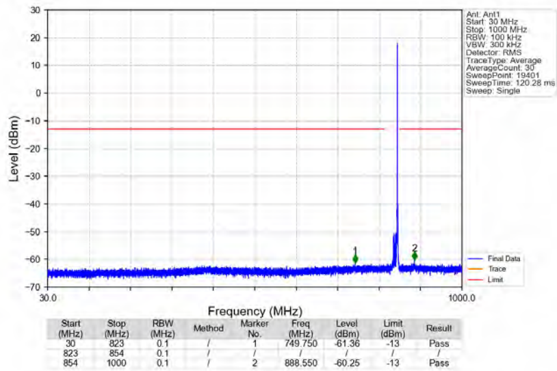
n5_15kHz_SISO_NTNV_10MHz_CP-OFDM_QPSK_844MHz_Edge_1RB_Right
