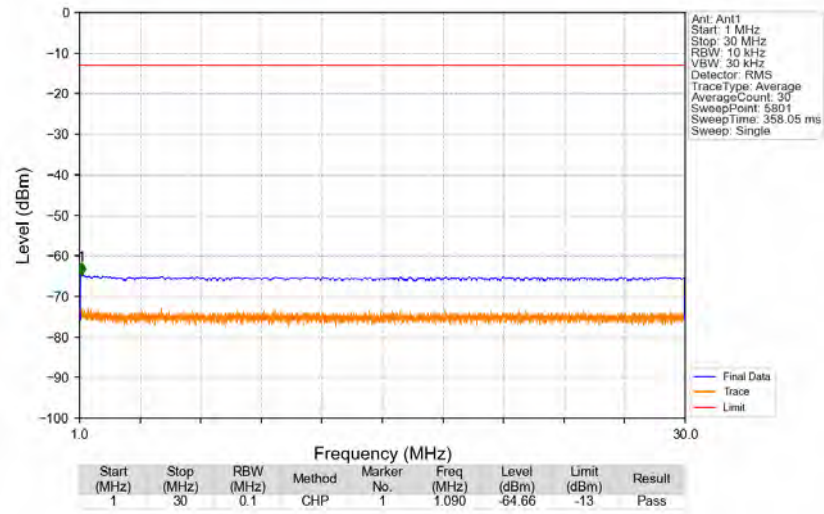
n5_15kHz_SISO_NTNV_15MHz_DFT-s-OFDM_QPSK_841.5MHz_Edge_1RB_Right
