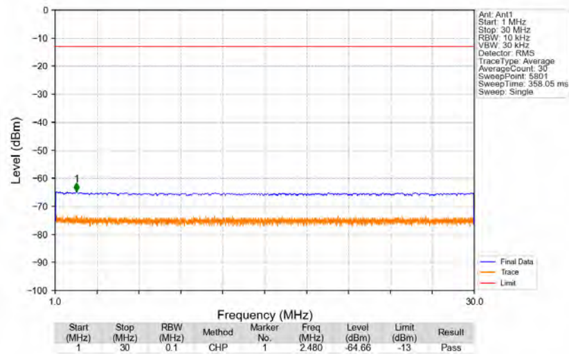
n5_15kHz_SISO_NTNV_15MHz_CP-OFDM_QPSK_836.5MHz_Edge_1RB_Left
