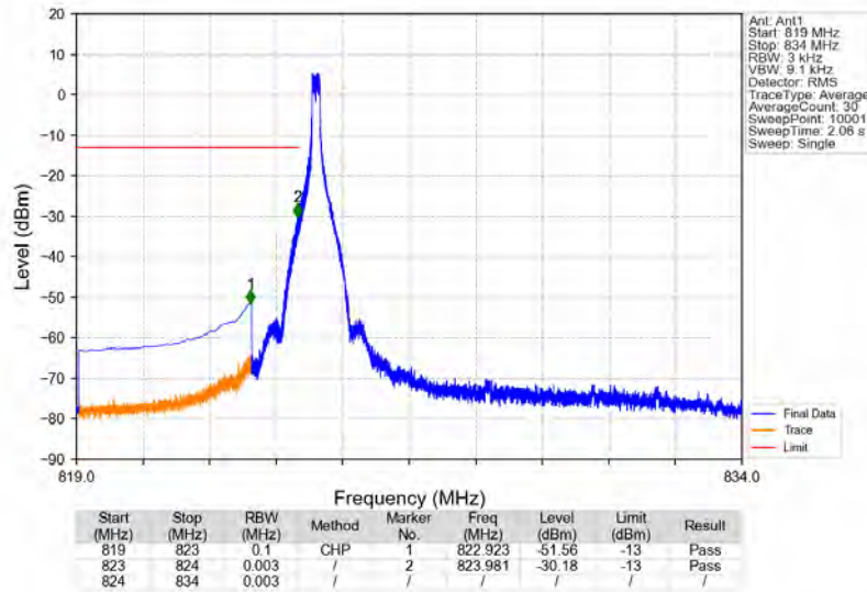
n5_15kHz_SISO_NTNV_10MHz_CP-OFDM_QPSK_829MHz_Edge_1RB_Left
