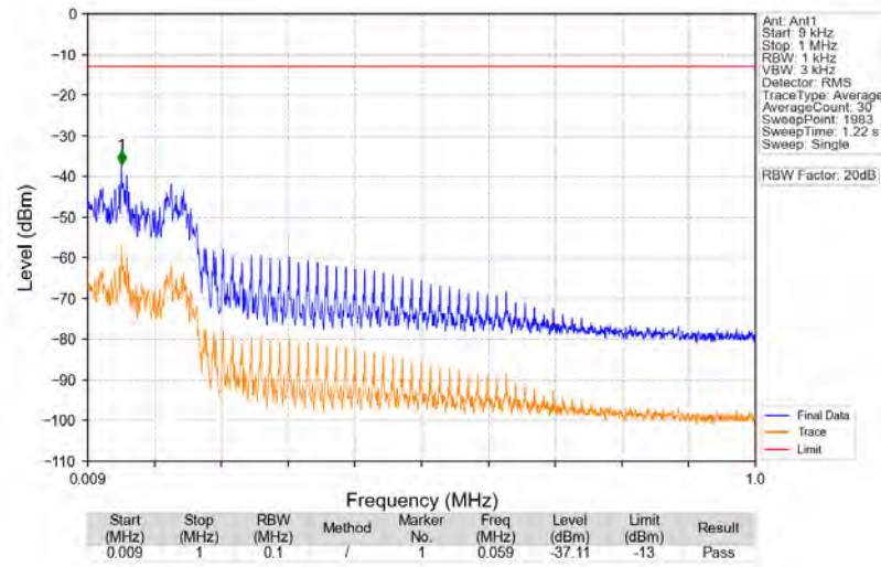
n5_15kHz_SISO_NTNV_10MHz_DFT-s-OFDM PI/2 BPSK 836.5MHz_Edge_1RB_Left
