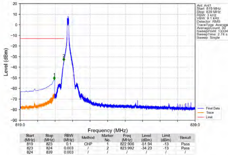
n5_15kHz_SISO_NTNV_15MHz_DFT-s-OFDM_QPSK_831.5MHz_Edge_1RB_Left
