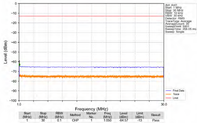
n5_15kHz_SISO_NTNV_20MHz_DFT-s-OFDM_QPSK_839MHz_Edge_1RB_Right
