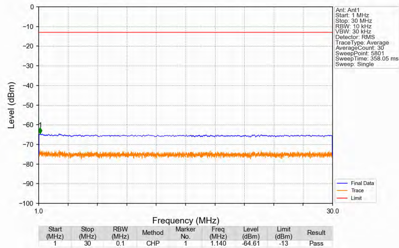
n5_15kHz_SISO_NTNV_20MHz_CP-OFDM_QPSK_834MHz_Edge_1RB_Left
