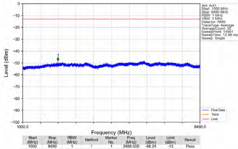
n5_15kHz_SISO_NTNV_15MHz_DFT-s-OFDM_QPSK_836.5MHz_Edge_1RB_Left
