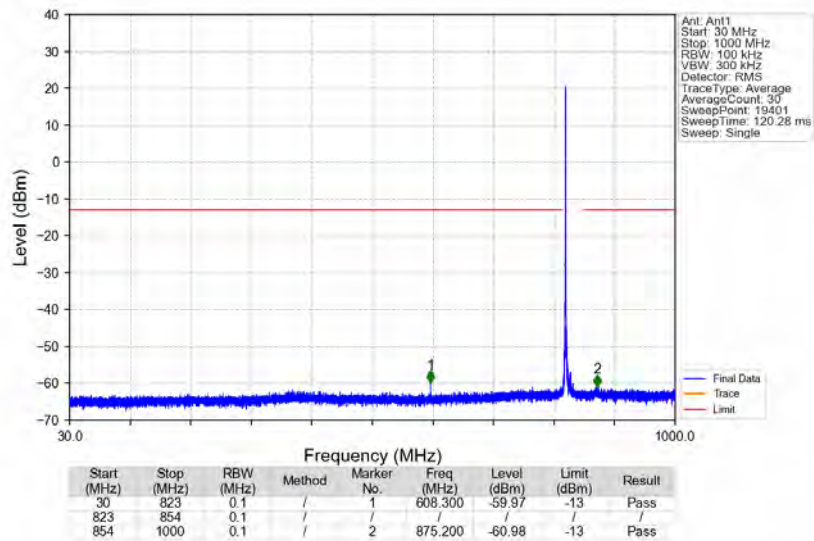
n5_15kHz_SISO_NTNV_10MHz_DFT-s-OFDM_QPSK_829MHz_Edge_1RB_Left
