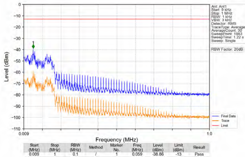
n5_15kHz_SISO_NTNV_15MHz_DFT-s-OFDM PI/2 BPSK_841.5MHz_Edge_1RB_Right
