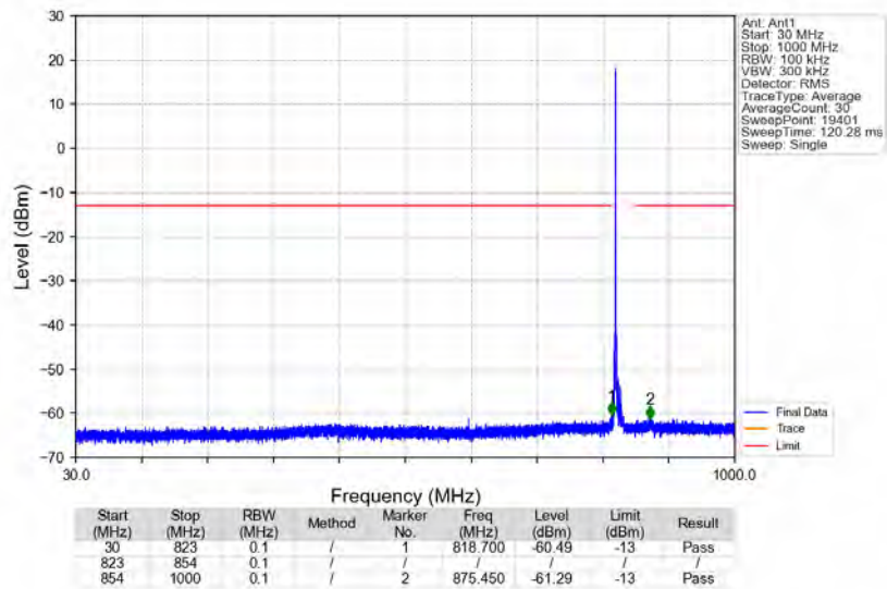
n5_15kHz_SISO_NTNV_10MHz_CP-OFDM_QPSK_829MHz_Edge_1RB_Left
