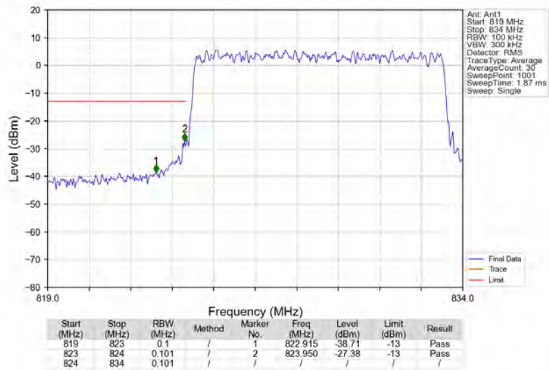
n5_15kHz_SISO_NTNV_10MHz_DFT-s-OFDM_QPSK_829MHz_Outer_Full
