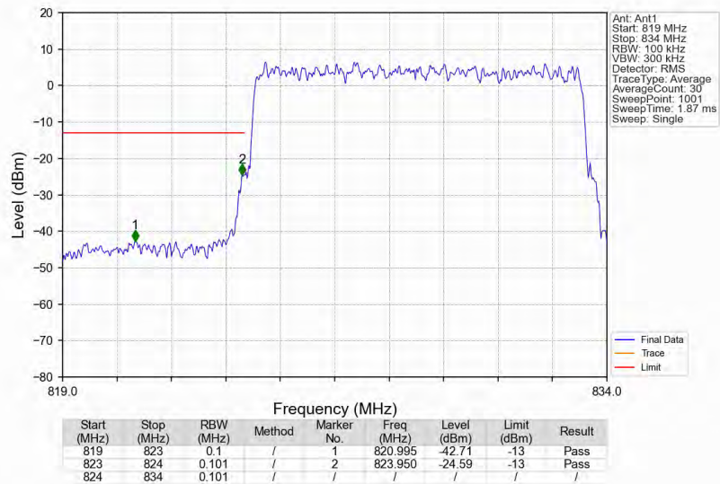
n5_15kHz_SISO_NTNV_10MHz_DFT-s-OFDM_PI/2_BPSK_829MHz_Outer_Full
