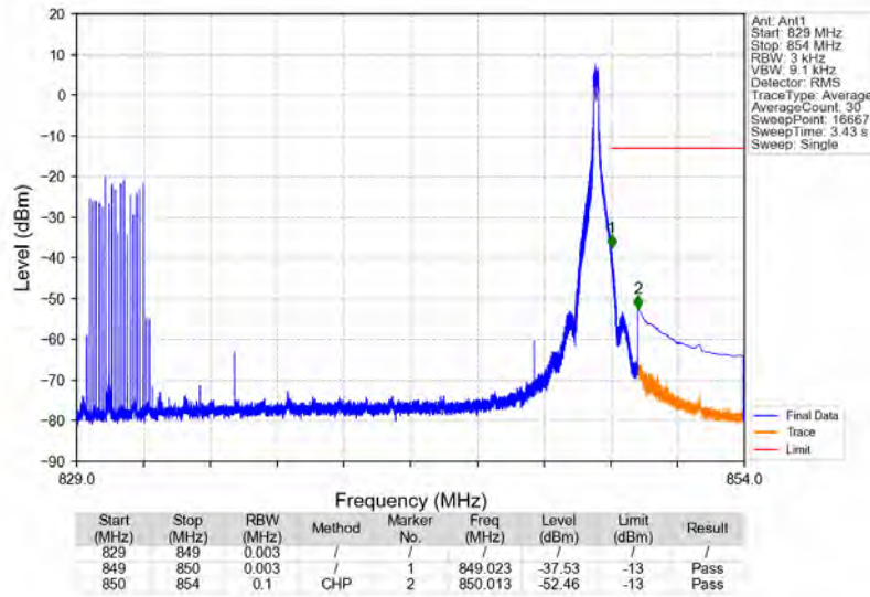
n5_15kHz_SISO_NTNV_20MHz_DFT-s-OFDM_QPSK_839MHz_Edge_1RB_Right
