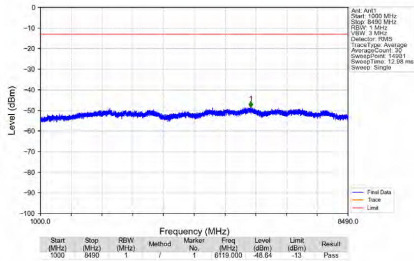
n5_15kHz_SISO_NTNV_10MHz_CP-OFDM_QPSK_844MHz_Edge_1RB_Right
