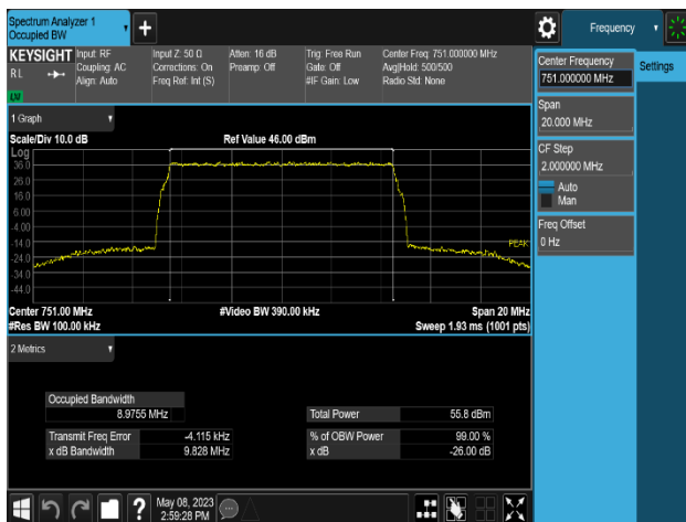
Plot 8-41. Occupied Bandwidth Plot (LTE B13_1C_10M_QPSK - Mid Channel_2T, Port 1)
