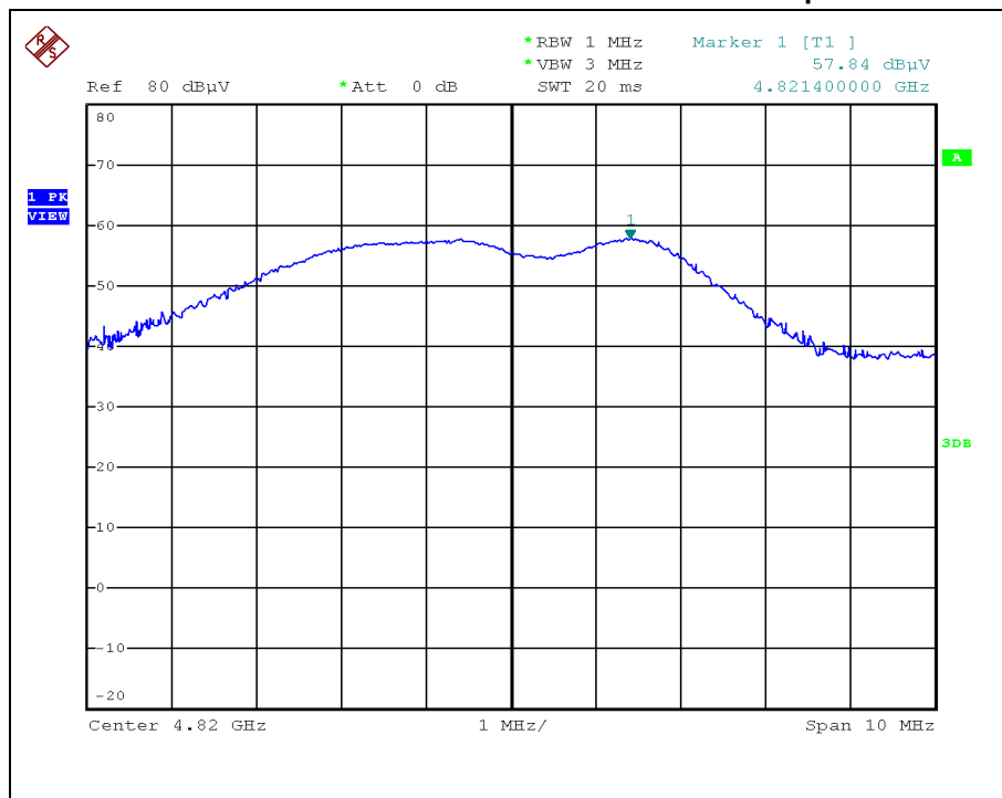
Spurious – Peak
