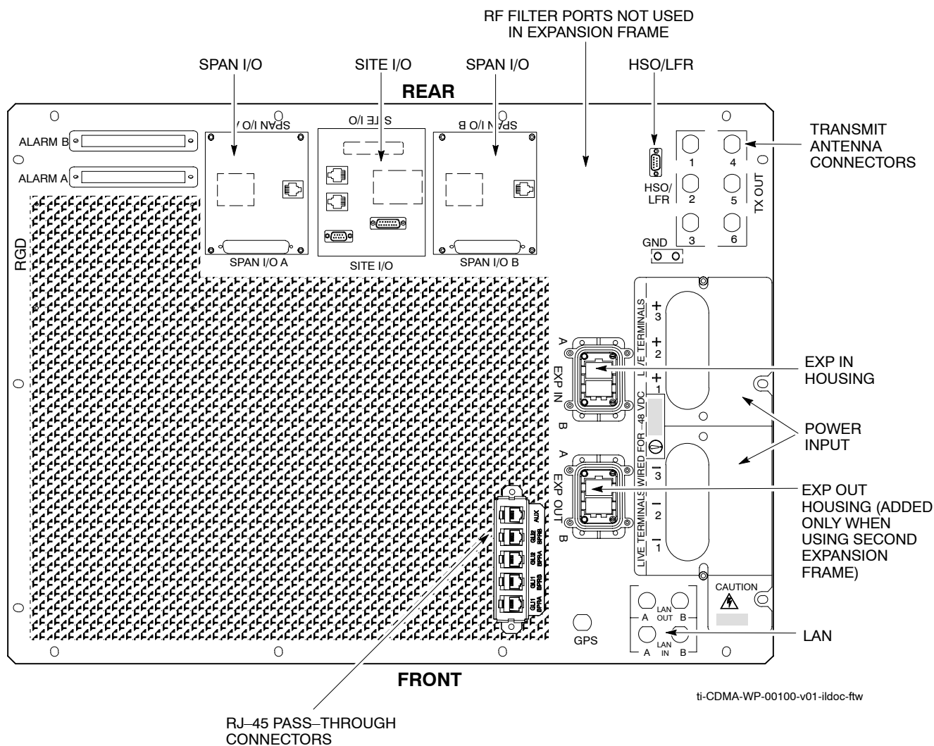
Figure 1-9: -48 V SC 4812T Expansion Frame I/O Interconnect Plate
