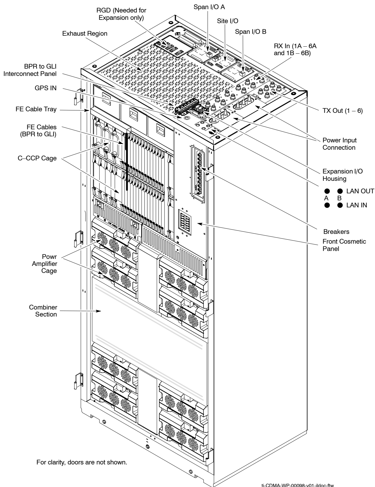
Figure 1-2: +27 V SC 4812T BTS Starter Frame
