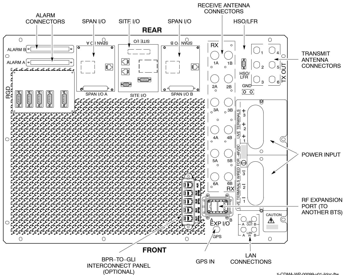
Figure 1-7: -48 V SC 4812T Starter Frame I/O Interconnect Plate
