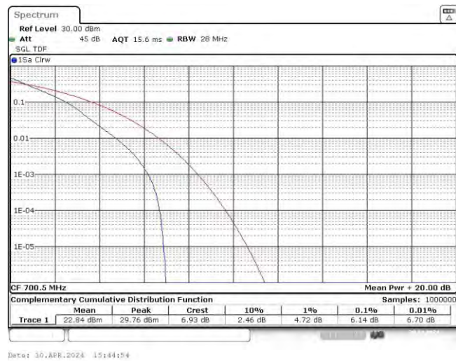
Band12-3MHz-QPSK-23095-15RB#0
