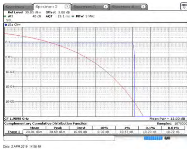
PCS_1900_GPRS_1909.8
