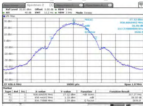
26dB BW_GSM_850_GPRS_836.6
