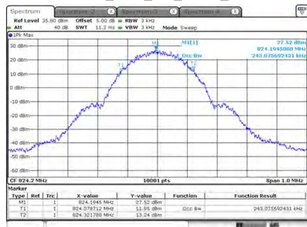
99% BW_GSM_850_GPRS_824.2
