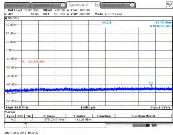
PCS_1900_GPRS_1880_under 1G
