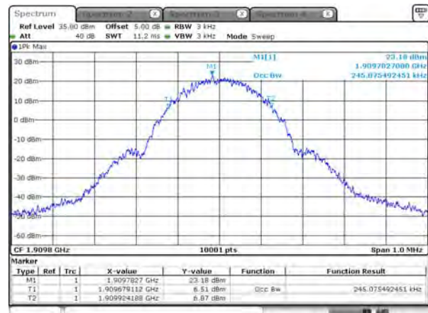
99% BW_PCS_1900_GPRS_1909.8
