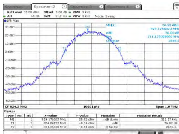
26dB BW_GSM_850_GPRS_824.2
