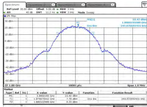
99% BW_PCS_1900_GPRS_1880
