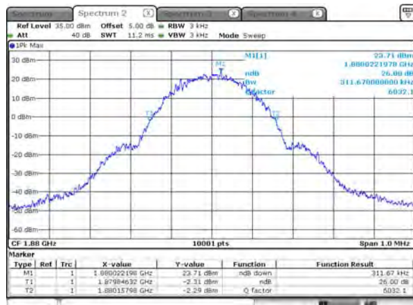
26dB BW_PCS_1900_GPRS_1880
