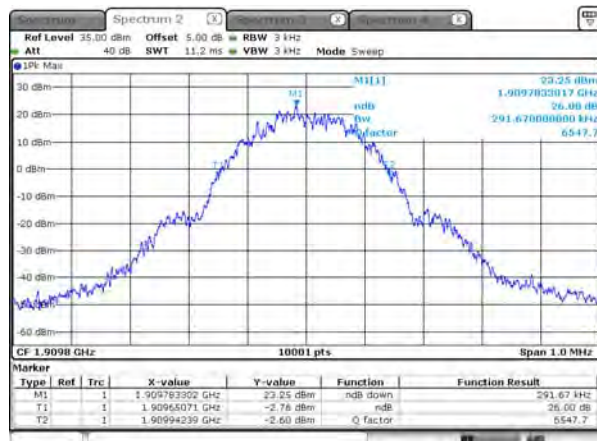
26dB BW_PCS_1900_GPRS_1909.8
