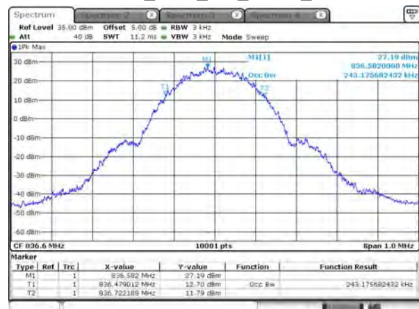
99% BW_GSM_850_GPRS_836.6
