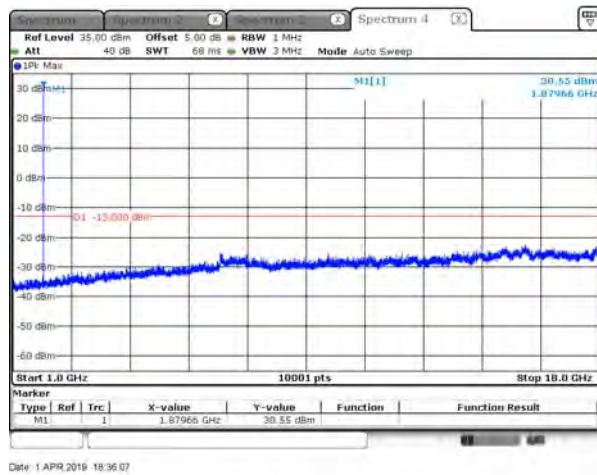
PCS_1900_GPRS_1880_above 1G
