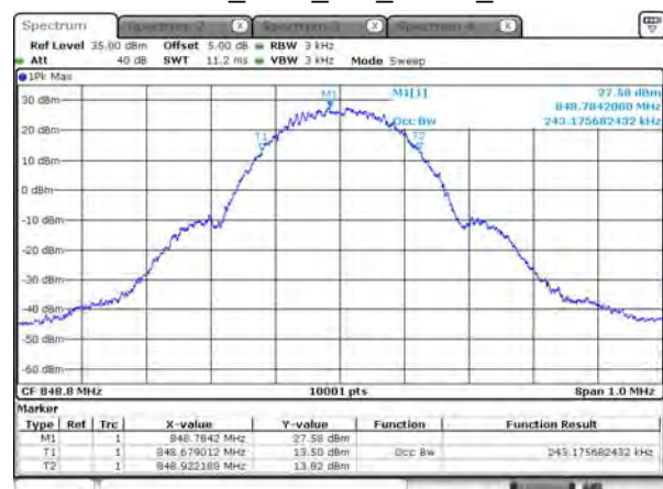
99% BW_GSM_850_GPRS_848.8
