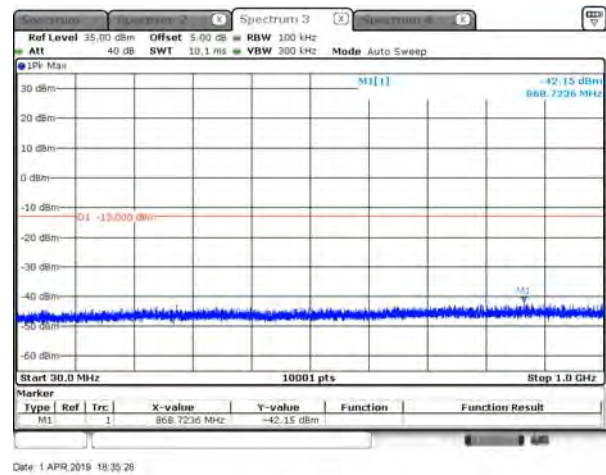
PCS_1900_GPRS_1880_under 1G
