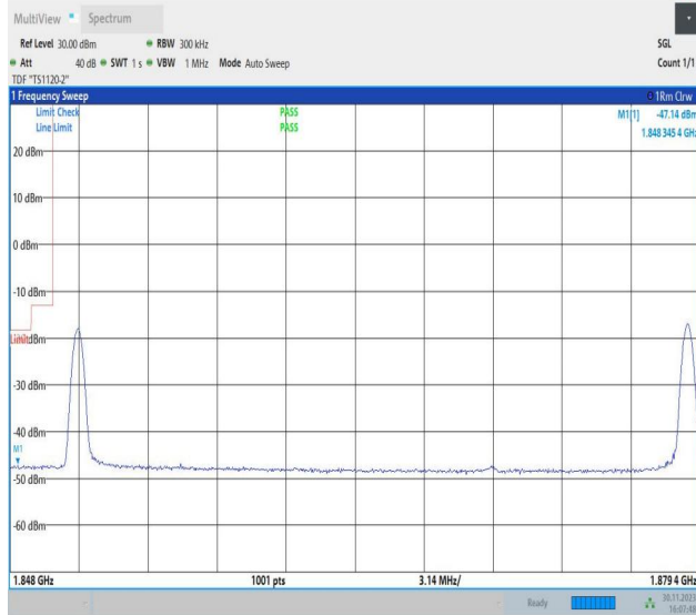
10MHz-20MHz_QPSK@QPSK-QPSK@QPSK_18655-18799_1RB#0@50RB#0-1RB#99@100RB#0
