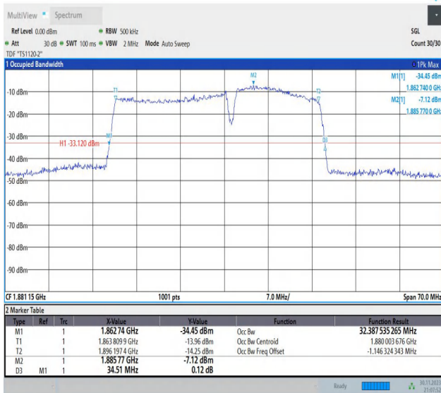
2-2-20MHz-15MHz-QPSK-QPSK-18826-18997-100RB#0-75R B#0-PASS
