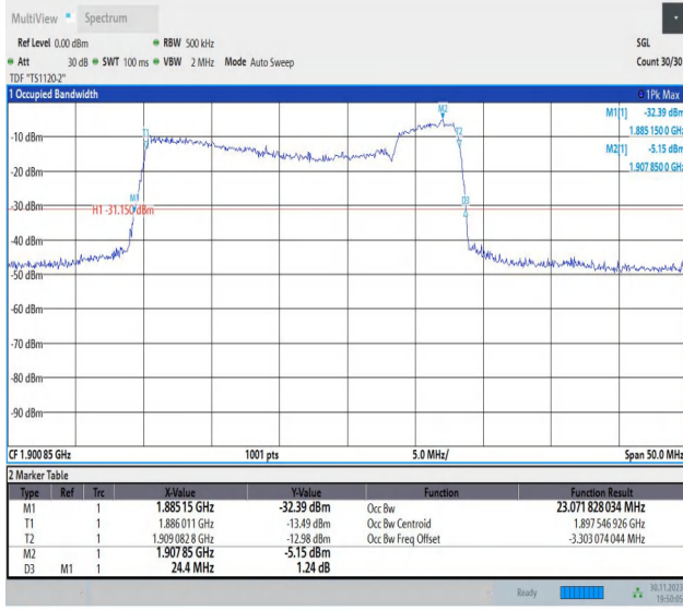
2-2-20MHz-5MHz-16QAM-16QAM-19050-19167-100RB#0-25 RB#0-PASS
