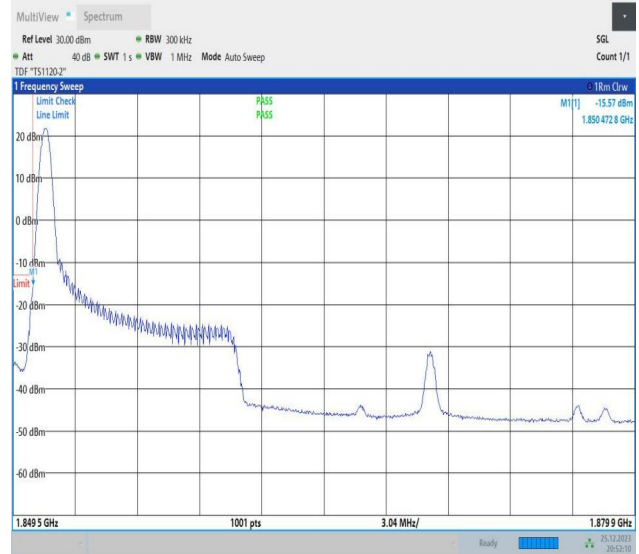
10MHz-20MHz_64QAM@64QAM-64QAM@64QAM_18655-18799_1RB#0@50RB#0-0RB#0@100RB#0
