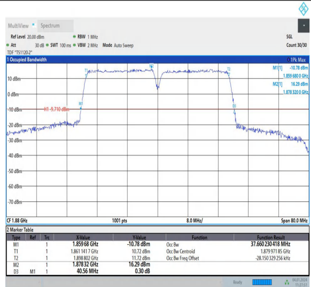
2-2-20MHz-15MHz-64QAM-64QAM-18951-19122-100RB#0-7 5RB#0-PASS
