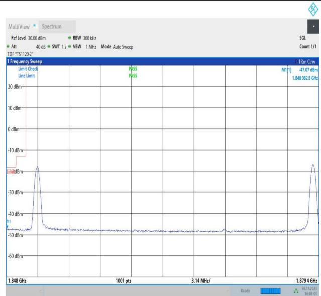
10MHz-20MHz_64QAM@64QAM-64QAM@64QAM_18655-18799_1RB#0@50RB#0-0RB#0@100RB#0
