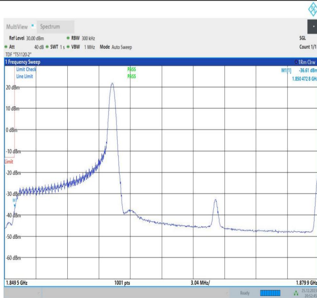
10MHz-20MHz_QPSK@QPSK-QPSK@QPSK_18655-18799_1RB#0@50RB#0-1RB#99@100RB#0
