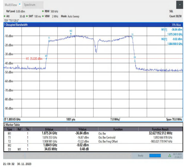
2-2-20MHz-15MHz-16QAM-16QAM-18951-19122-100RB#0-7 5RB#0-PASS
