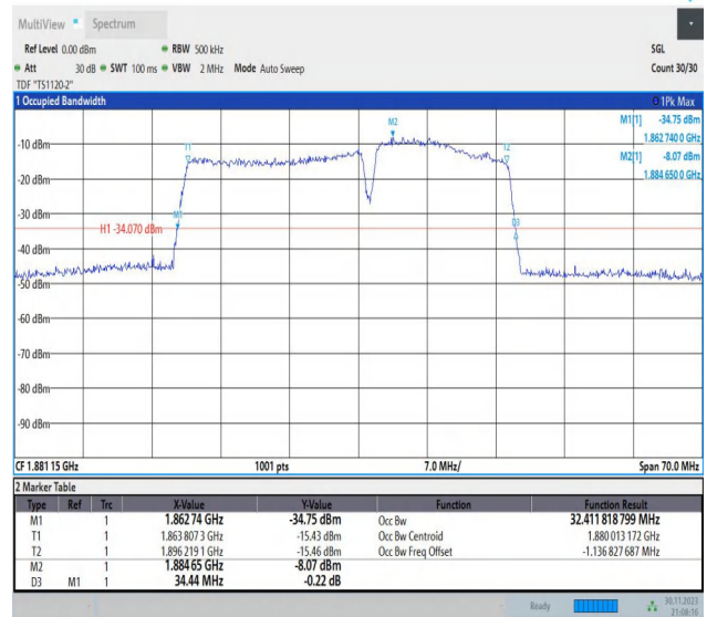
2-2-20MHz-15MHz-16QAM-16QAM-18826-18997-100RB#0-7 5RB#0-PASS
