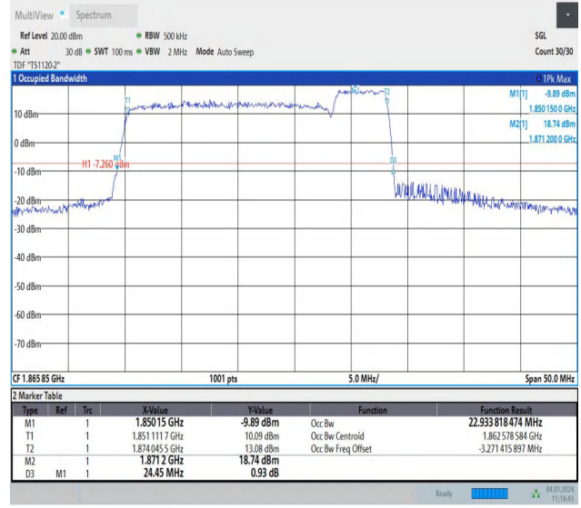
2-2-20MHz-5MHz-64QAM-64QAM-18700-18817-100RB#0-25 RB#0-PASS
