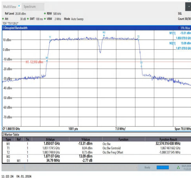
2-2-20MHz-15MHz-64QAM-64QAM-18700-18871-100RB#0-7 5RB#0-PASS
