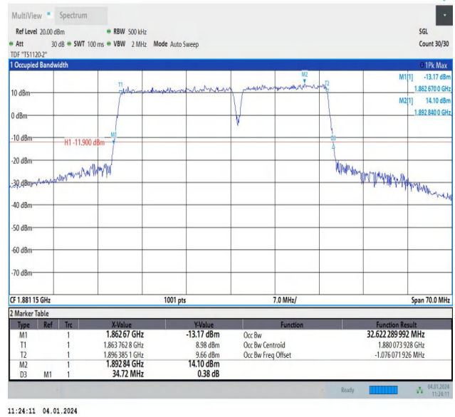
2-2-20MHz-15MHz-64QAM-64QAM-18826-18997-100RB#0-7 5RB#0-PASS
