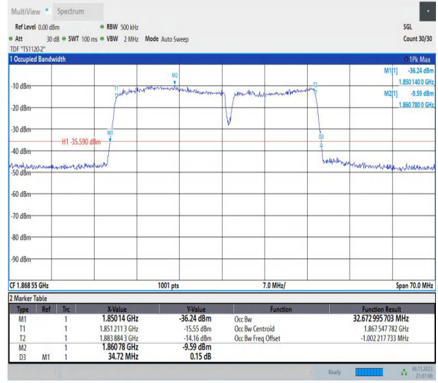
2-2-20MHz-15MHz-16QAM-16QAM-18700-18871-100RB#0-7 5RB#0-PASS
