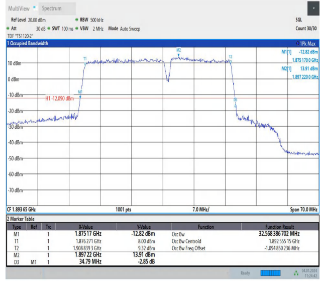
2-2-20MHz-15MHz-64QAM-64QAM-18951-19122-100RB#0-7 5RB#0-PASS
