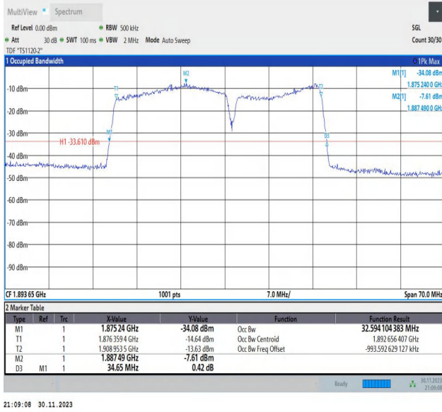
2-2-20MHz-15MHz-QPSK-QPSK-18951-19122-100RB#0-75R B#0-PASS
