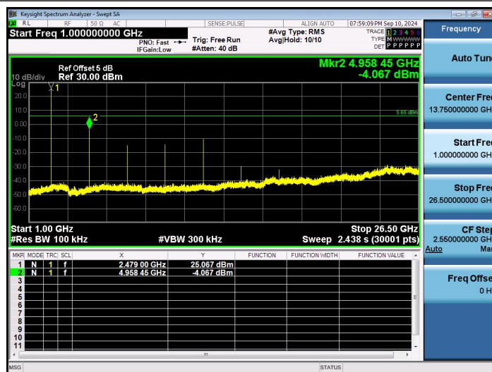
2.4G-Ant2-2479.4-1000~26500-PASS
