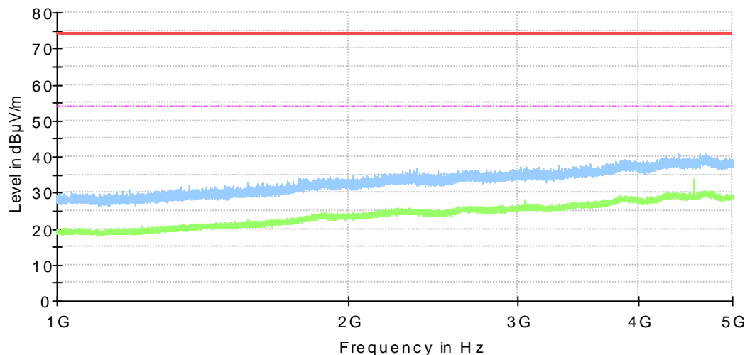
TEST SITE: Semi anechoic chamber LIMIT: Class B TEST DISTANCE: 3 m EUT OPERATING MODE: Receive
