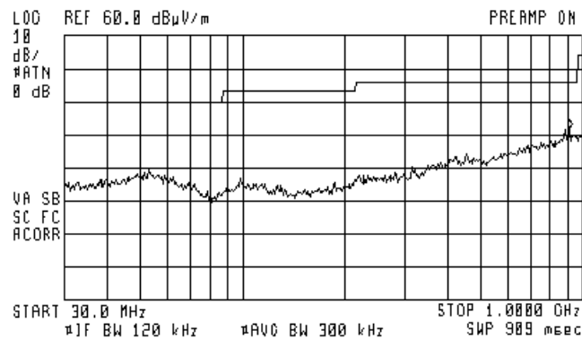
TEST SITE: Semi anechoic chamber LIMIT: Class B TEST DISTANCE: 3 m EUT OPERATING MODE: Receive
