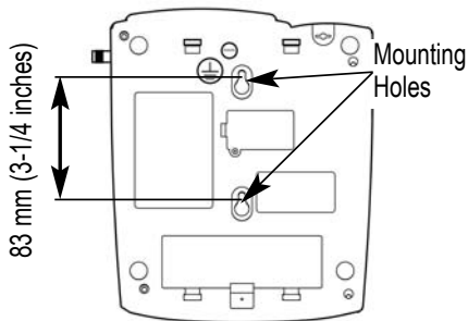
Figure 15 – SX5D mounting hooks.
