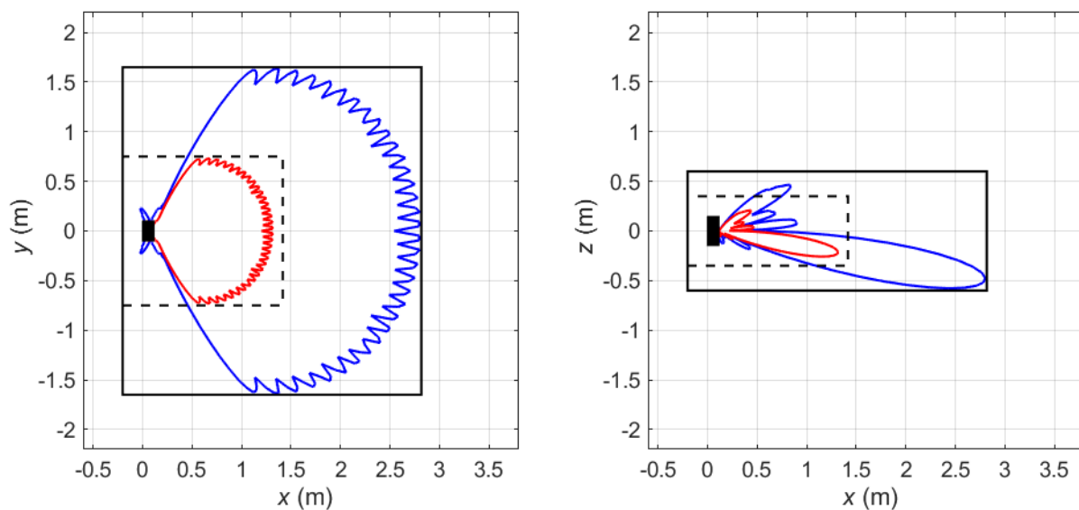
Figure 13 Compliance boundaries for general public (black solid line) and workers (black dashed line) exposure for markets where the FCC exposure limits apply for Macro11 (tilt 7.5°) sector shape (Configuration Mode 1). The blue solid lines correspond to compliance distance results for general public exposure obtained using the spherical models. The solid red lines indicate the corresponding compliance distance results for workers exposure. The EUT is shown from above (left) and from the side (right) with its backplane located at x = 0 m. Mode: B258 (26 GHz) (NR). Total EIRP of the radio: 60.2 dBm.
