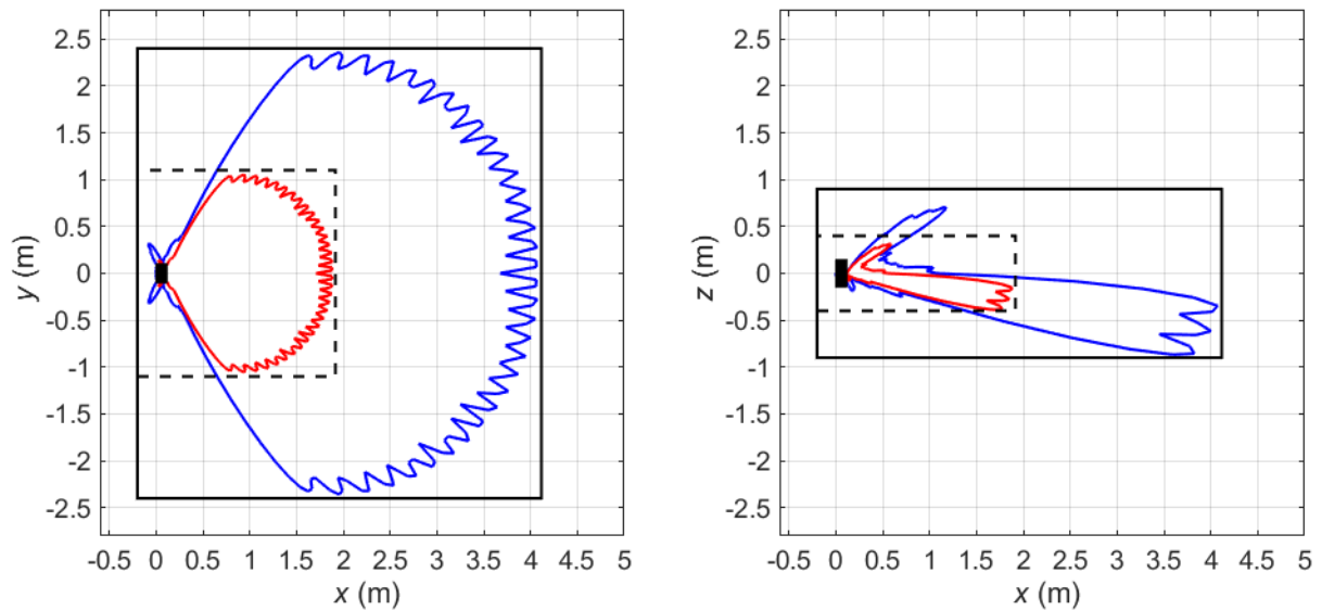
Figure 20 Compliance boundaries for general public (black solid line) and workers (black dashed line) exposure for markets where the FCC exposure limits apply for Macro13 (tilt 11.25°) sector shape (Configuration Mode 2). The blue solid lines correspond to compliance distance results for general public exposure obtained using the spherical models. The solid red lines indicate the corresponding compliance distance results for workers exposure. The EUT is shown from above (left) and from the side (right) with its backplane located at x = 0 m. Mode: B258 (26 GHz) (NR). Total EIRP of the radio: 63.2 dBm.
