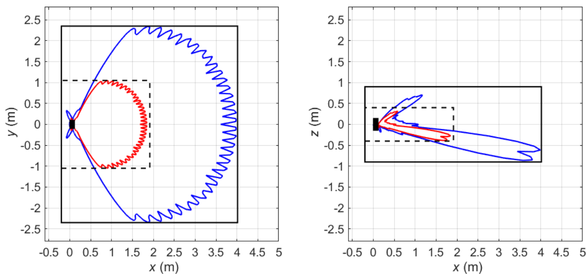
Figure 18 Compliance boundaries for general public (black solid line) and workers (black dashed line) exposure for markets where the FCC exposure limits apply for Macro7 (tilt 11.25°) sector shape (Configuration Mode 2). The blue solid lines correspond to compliance distance results for general public exposure obtained using the spherical models. The solid red lines indicate the corresponding compliance distance results for workers exposure. The EUT is shown from above (left) and from the side (right) with its backplane located at x = 0 m. Mode: B258 (26 GHz) (NR). Total EIRP of the radio: 63.2 dBm.
