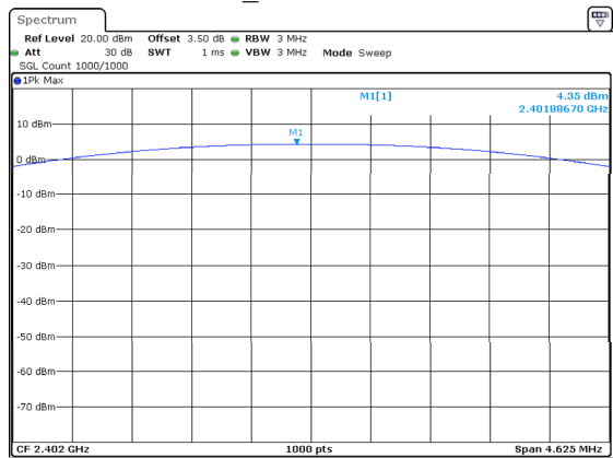
DH1_Low 4.35dBm
