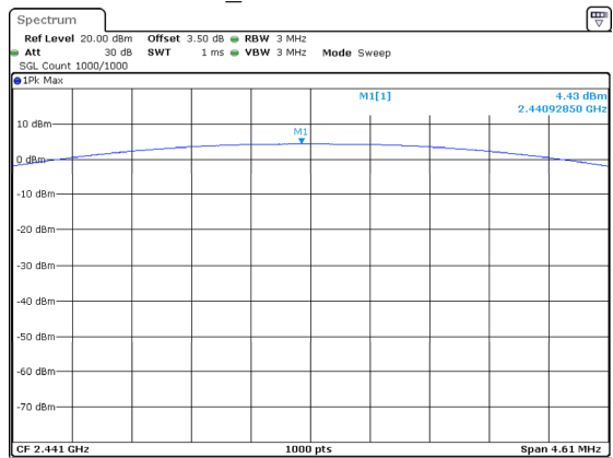
DH1_Middle 4.43dBm
