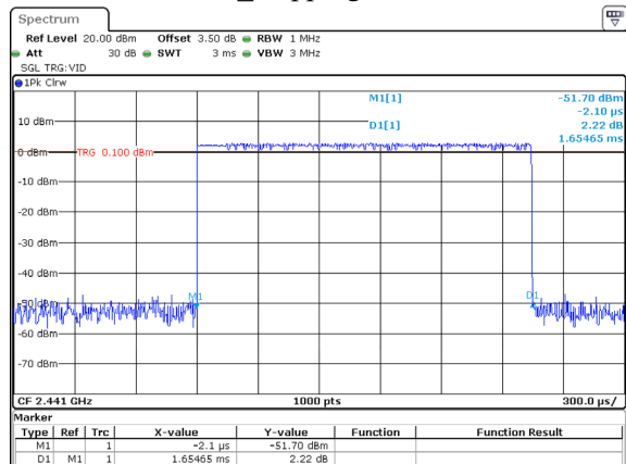
2DH3_Hopping 1.655ms
