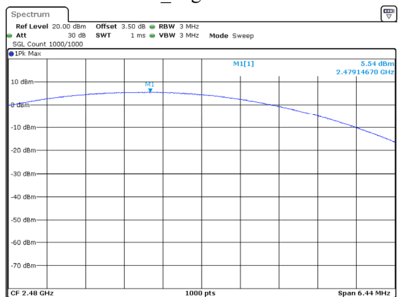
2DH1_High 5.54dBm
