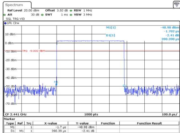
DH1_Hopping 0.390ms
