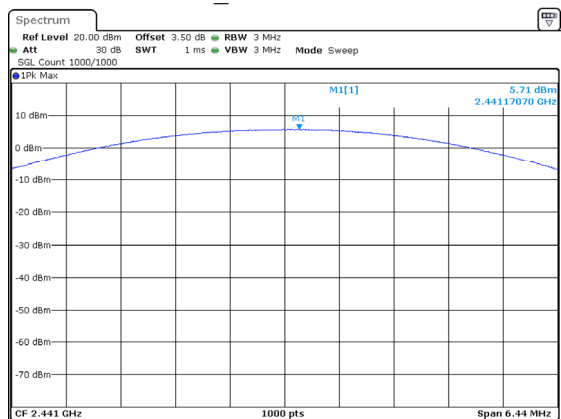
2DH1_Middle 5.71dBm
