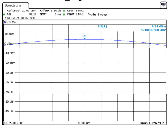
DH1_High 4.24dBm
