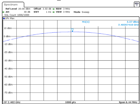
2DH1_Low 5.57dBm
