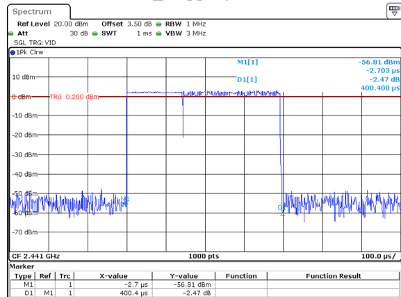
2DH1_Hopping 0.400ms
