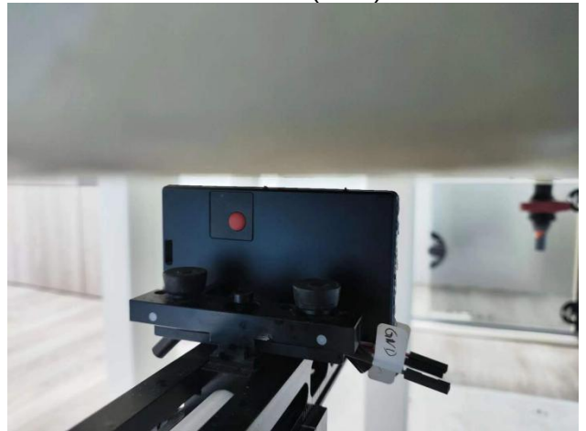
Right side(5mm)
