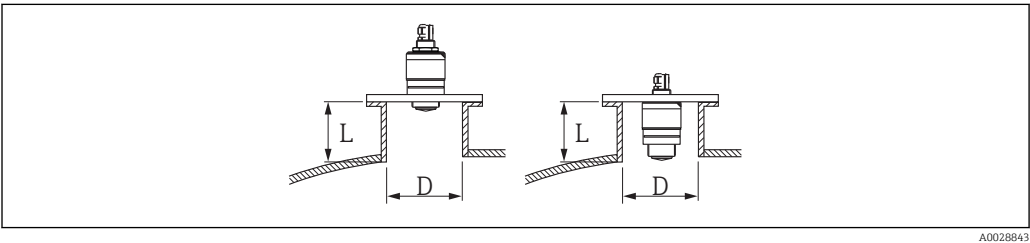
6 FMR10 nozzle installation
