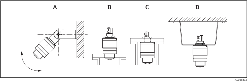
5 Wall, ceiling or nozzle installation A Wall or ceiling mount, adjustable B Mounted at front thread C Mounted at rear thread D Ceiling installation with counter nut (included in delivery)
