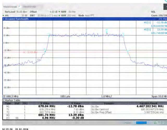
Band71-5MHz-16QAM-133297-25RB#0
