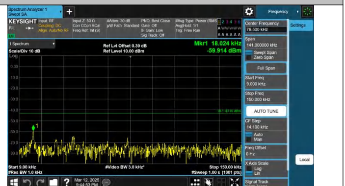
Band4-15MHz-QPSK-20175-1RB#74-0.009~0.15-PASS
