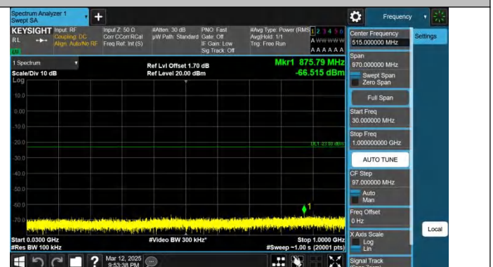
Band4-20MHz-QPSK-20175-1RB#99-30~1000-PASS
