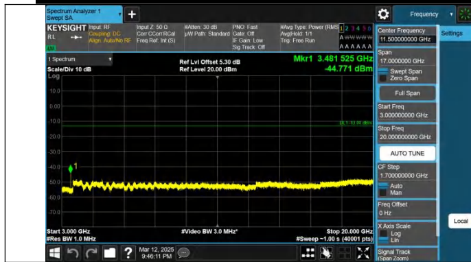
Band4-15MHz-QPSK-20325-1RB#0-3000~20000-PASS
