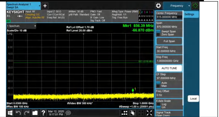
Band4-3MHz-QPSK-20385-1RB#14-30~1000-PASS
