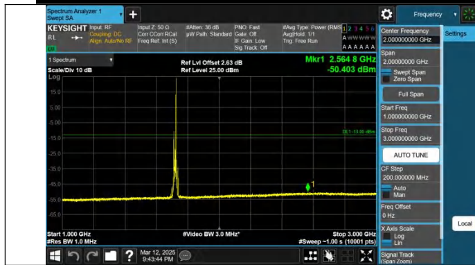
Band4-15MHz-QPSK-20025-1RB#74-1000~3000-PASS
