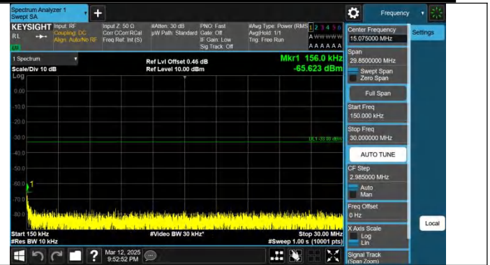
Band4-20MHz-QPSK-20175-1RB#0-0.15~30-PASS
