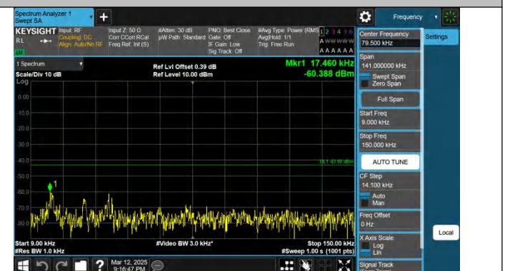
Band4-3MHz-QPSK-20385-1RB#14-0.009~0.15-PASS
