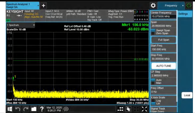
Band4-5MHz-QPSK-20375-1RB#0-0.15~30-PASS
