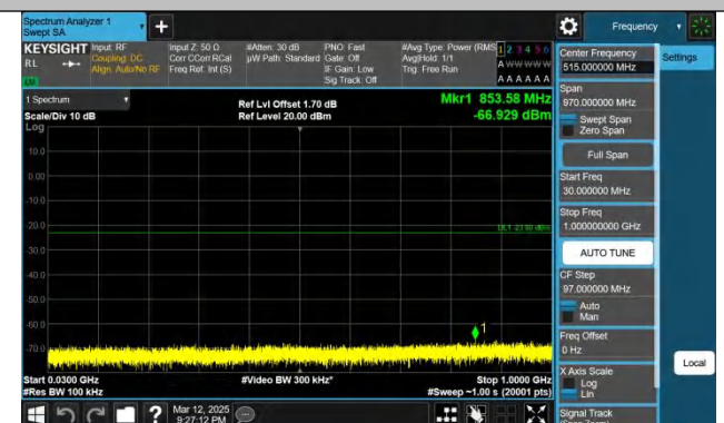
Band4-5MHz-QPSK-20375-1RB#24-30~1000-PASS
