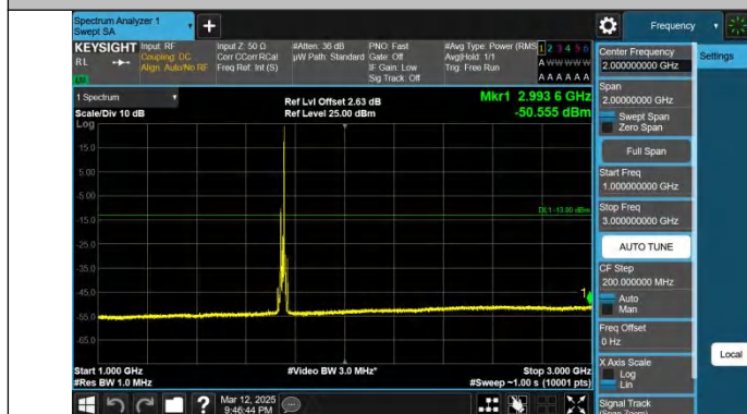
Band4-15MHz-QPSK-20325-1RB#74-1000~3000-PASS
