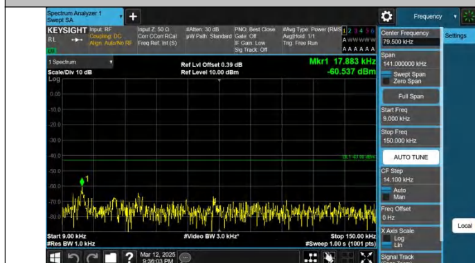
Band4-10MHz-QPSK-20350-1RB#0-0.009~0.15-PASS
