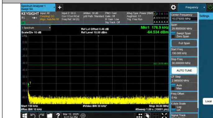
Band4-5MHz-QPSK-20375-1RB#24-0.15~30-PASS
