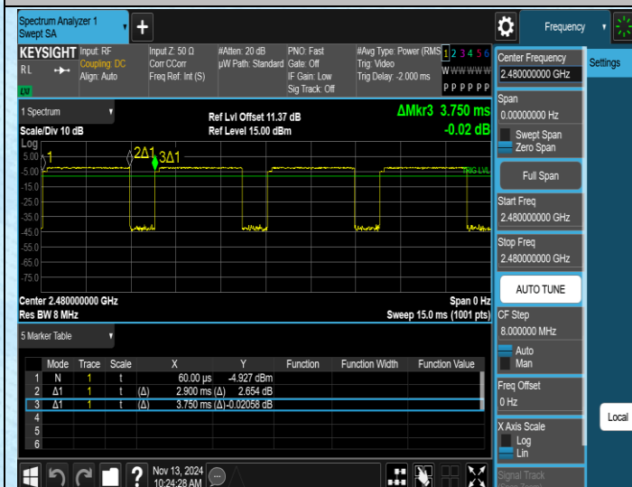
NTNV-3DH5-Ant1-2480
