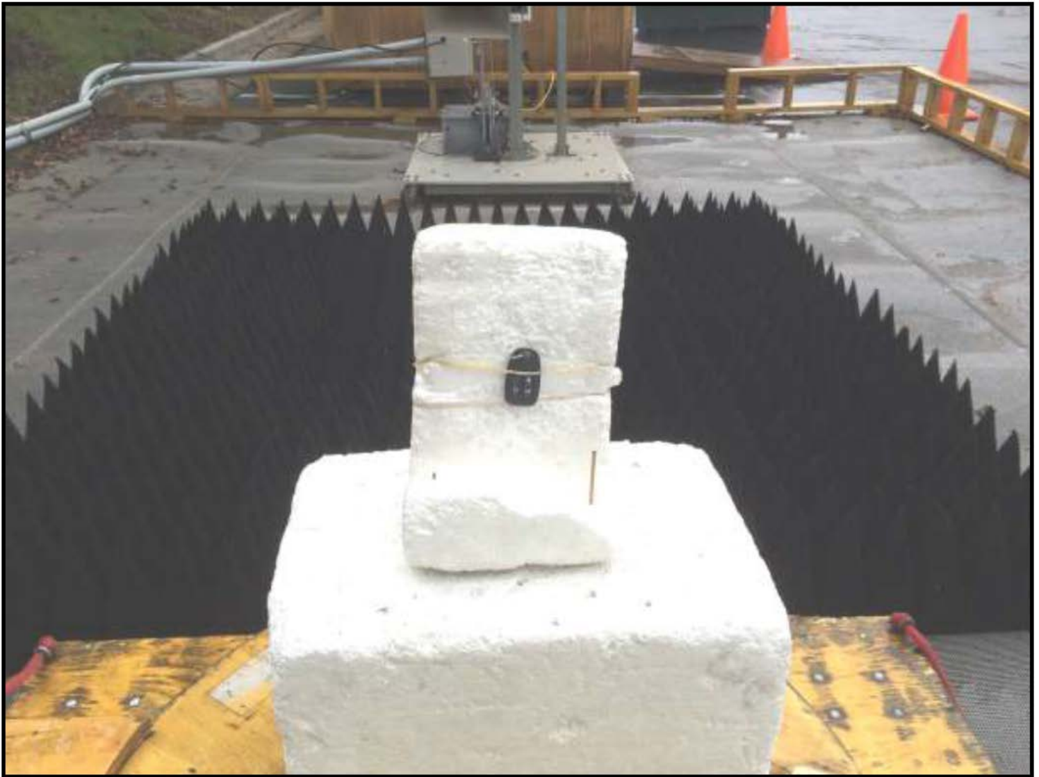
Photograph 1: Radiated Emissions
