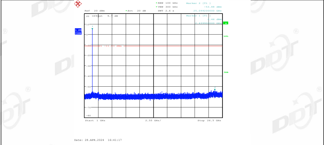
3DH5_Right side_2480_0~Reference
