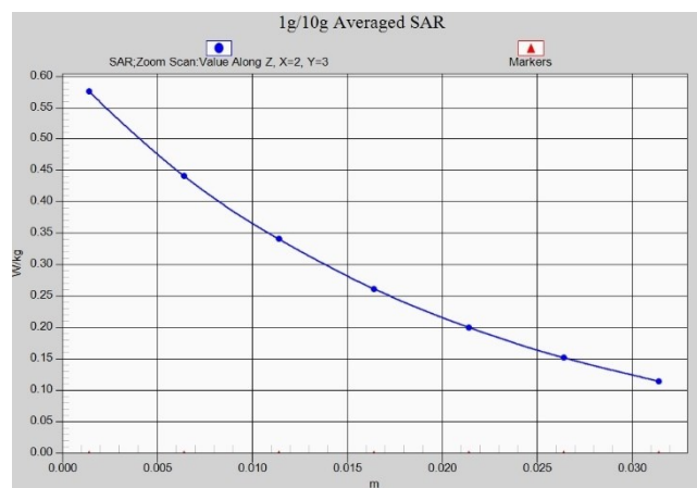
Fig. 1-21 Z-Scan at power reference point (LTE Band14)
