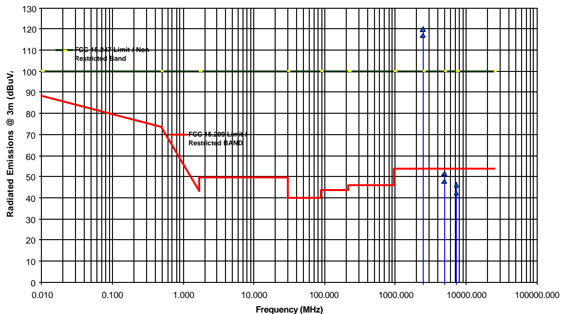
Transmitter Radiated Emissions Measurements at 3 Meter OETS Aerocomm LX2400-150 FHSS 148 mW Transmitter Tx Freq.:2440 MHz, Antenna: Maxrad MC2400 Antenna
