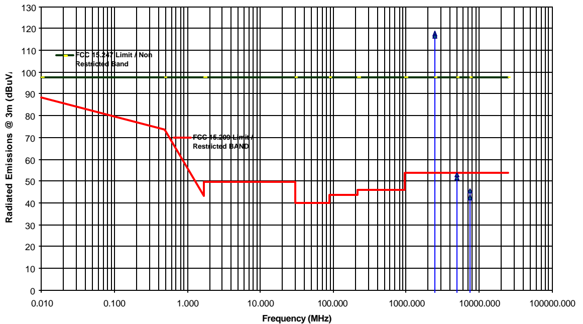
Transmitter Radiated Emissions Measurements at 3 Meter OFTS Aerocomm LX2400-150 FHSS 148 mW Transmitter Tx Freq.:2478 MHz, Antenna: Nearson S131CL-RMM-2450S
