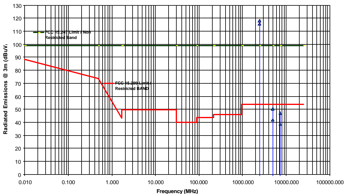
Transmitter Radiated Emissions Measurements at 3 Meter OFTS Aerocomm LX2400-150 FHSS 148 mW Transmitter Tx Freq.:2440 MHz, Antenna: Centurion WCP2400-MMCX
