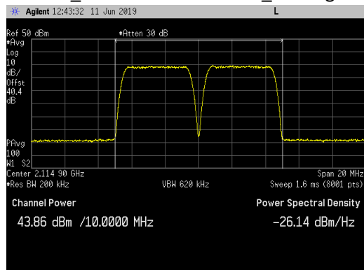
64QAM_ 2112.4 &amp; 2117.4MHz_ Average Power
