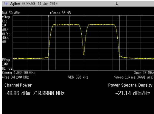
16QAM_ 1932.4 &amp; 1937.4MHz_ Average Power
