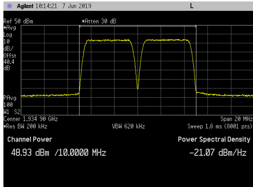
QPSK_ 1932.4 &amp; 1937.4MHz_ Average Power
