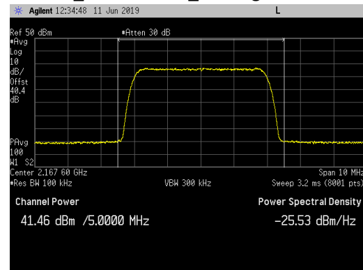
16QAM_ 2167.6MHz_ Average Power
