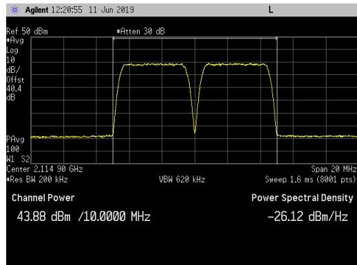
QPSK_ 2112.4 &amp; 2117.4MHz_ Average Power
