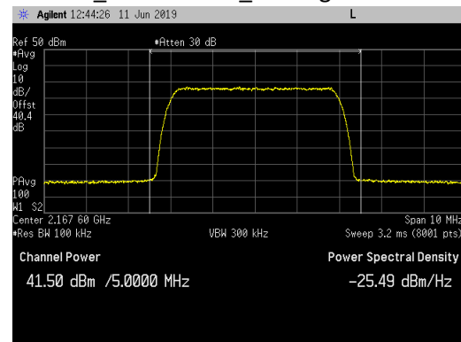
64QAM_ 2167.6MHz_ Average Power
