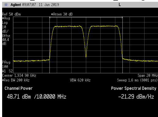
64QAM_ 1932.4 &amp; 1937.4MHz_ Average Power
