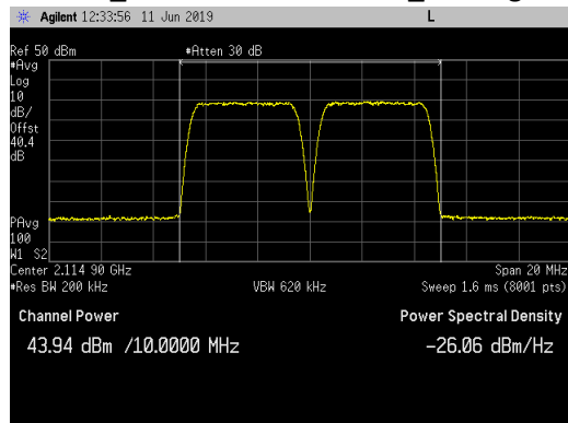
16QAM_ 2112.4 &amp; 2117.4MHz_ Average Power
