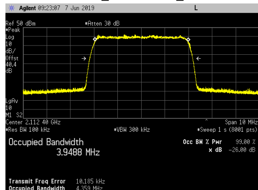
Bottom Channel_2112.4MHz_QPSK Modulation
