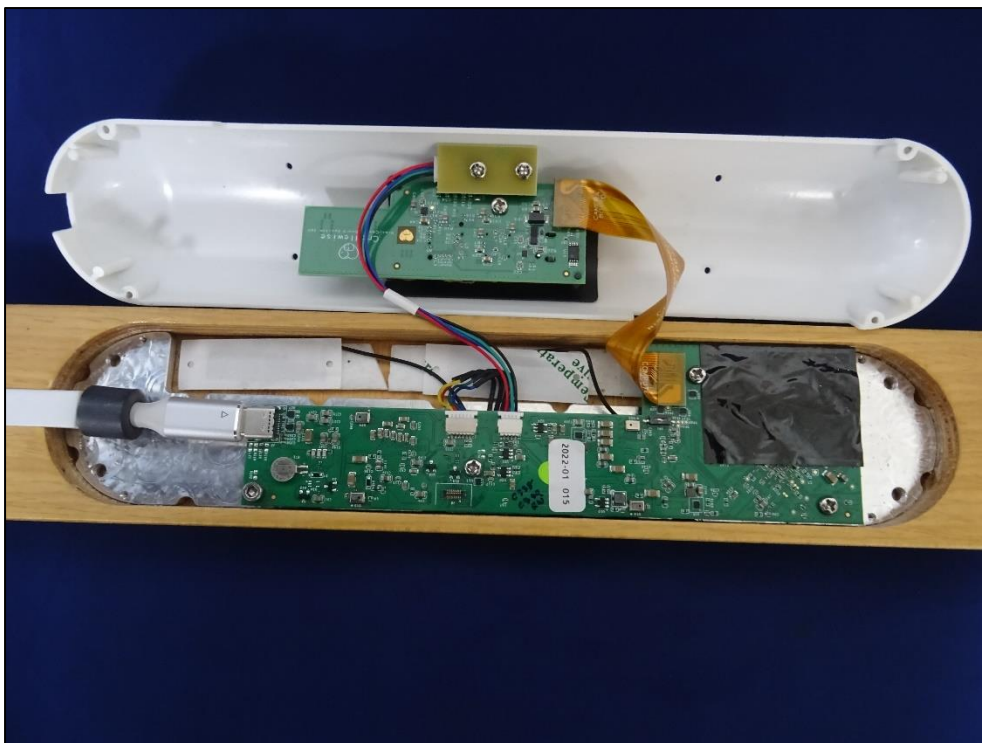
Photo 14: Monitor arc with monitor cover open
