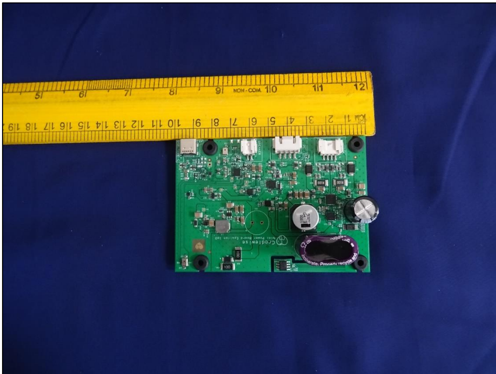
Photo 21: Power board dimensional View
