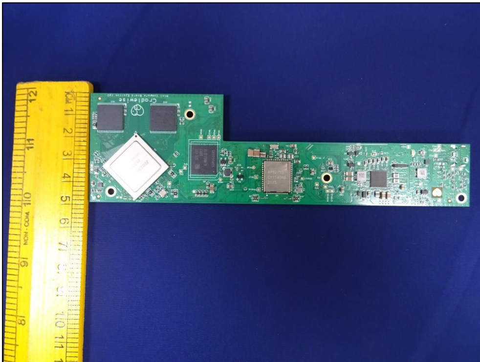
Photo 23: Compute board with dimension view
