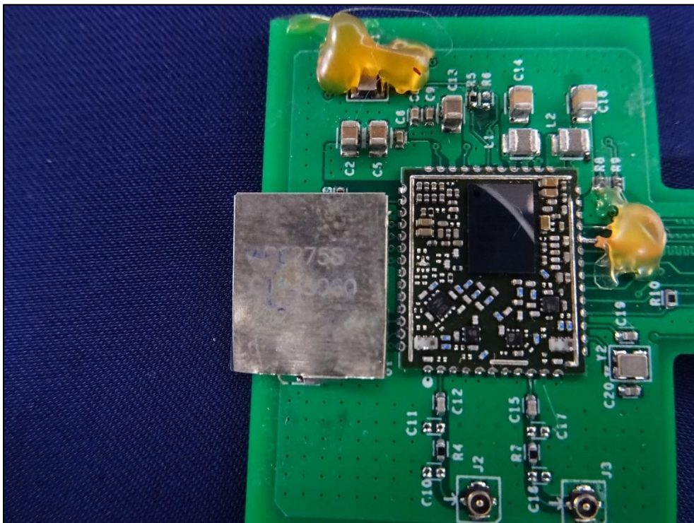
Photo 26: Wireless module with shield open
