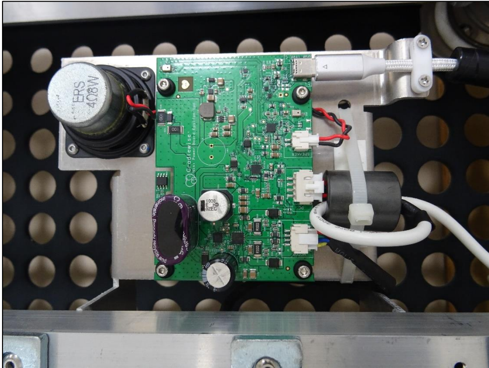
Photo 11: Power board and speaker used in the cradle
