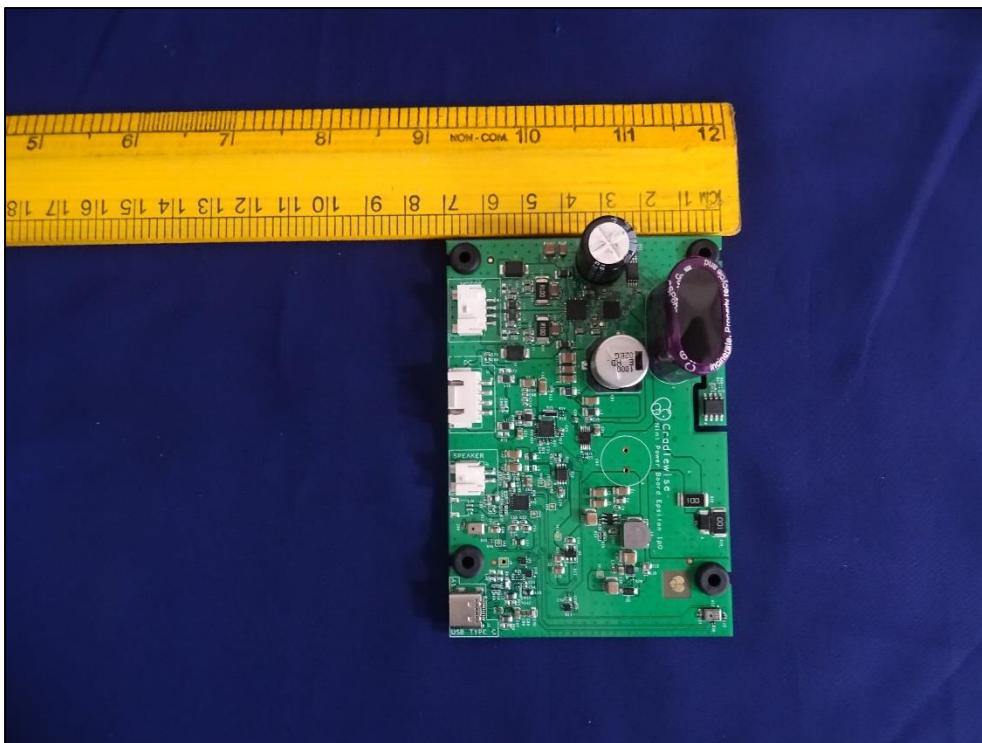
Photo 22: Power board dimensional View
