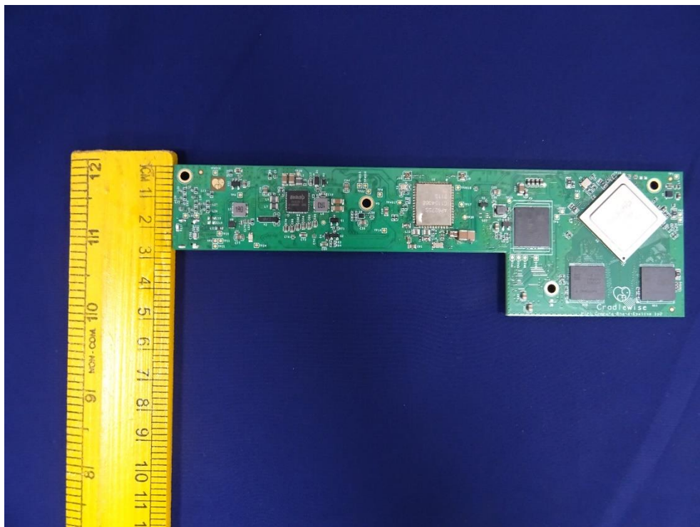
Photo 24: Compute board with dimension view
