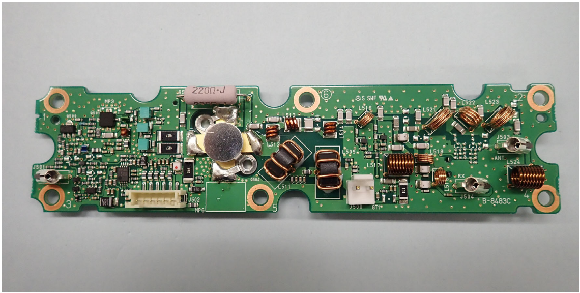
PA-E (TOP)
