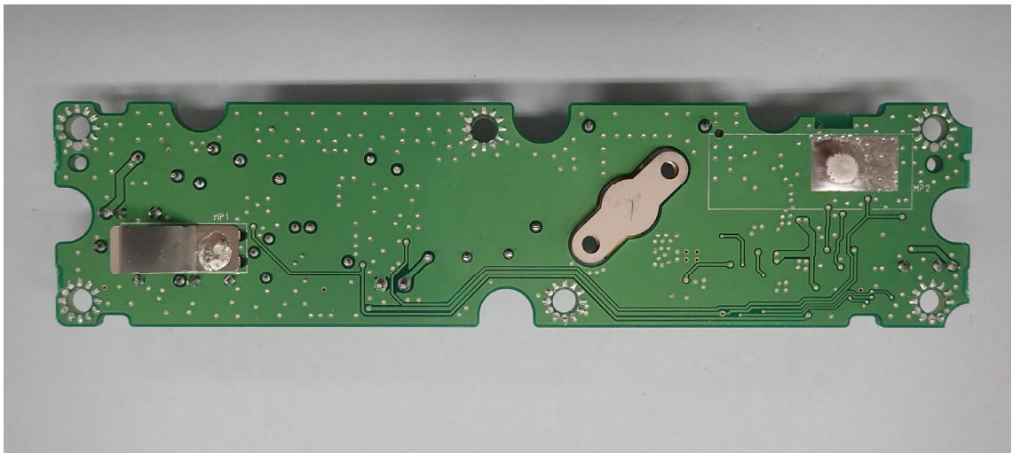
PA-E (BOTTOM)
