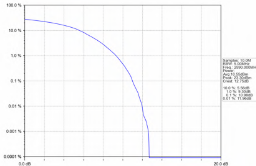
n38_30kHz_SISO_NTNV_40MHz_DFT-s-OFDM QPSK_2590MHz_Outer_Full
