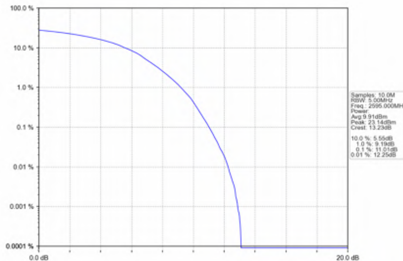
n38_30kHz_SISO_NTNV_20MHz_DFT-s-OFDM_256_QAM_2595MHz_Outer_Full
