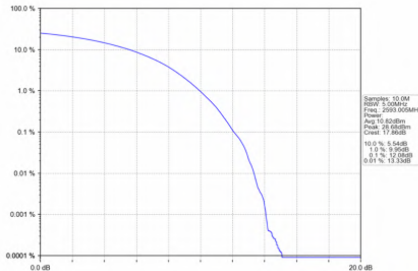
n41_15kHz_SISO_NTNV_30MHz_CP-OFDM 64 QAM_2593.005MHz_Outer_Full
