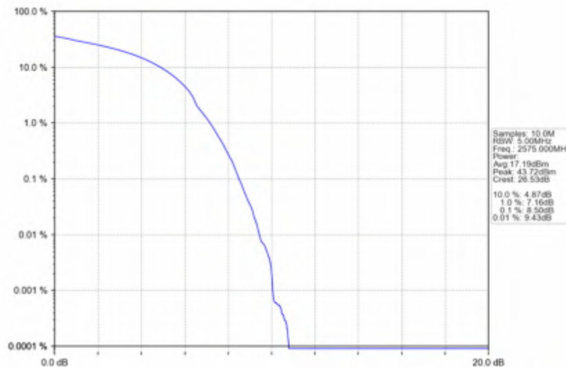
n38_30kHz_SISO_NTNV_10MHz_DFT-s-OFDM_64_QAM_2575MHz_Outer_Full
