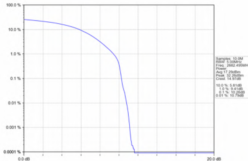
n41_15kHz_SISO_NTNV_15MHz_DFT-s-OFDM_QPSK_2682.495MHz_Outer_Full
