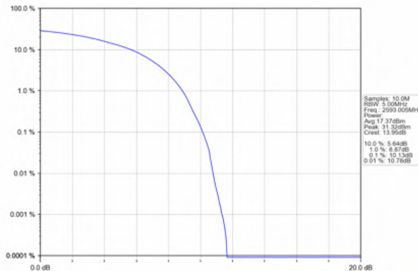
n41_15kHz_SISO_NTNV_10MHz_DFT-s-OFDM 64 QAM_2593.005MHz_Outer_Full
