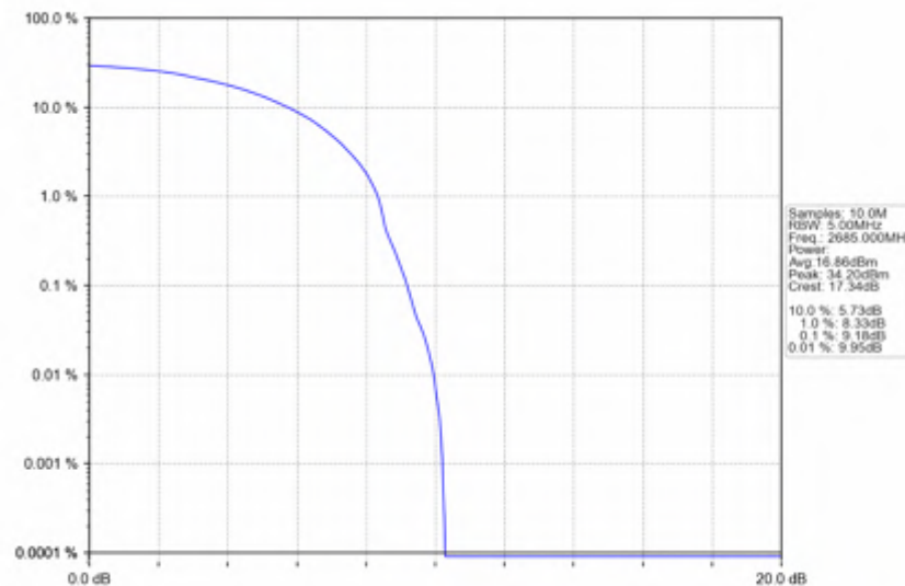
n41_30kHz_SISO_NTNV_10MHz_DFT-s-OFDM QPSK_2685MHz_Outer_Full
