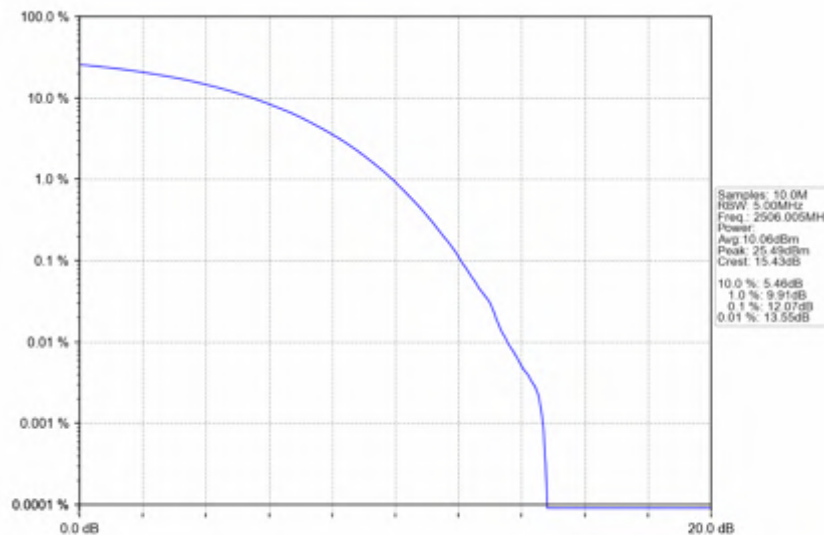
n41_15kHz_SISO_NTNV_20MHz_CP-OFDM_256_QAM_2506.005MHz_Outer_Full
