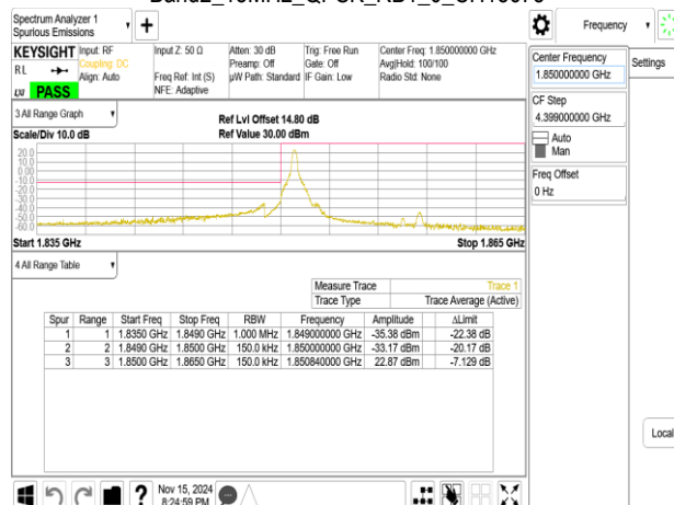
Band2_15MHz_QPSK_RB75_0_CH18675
