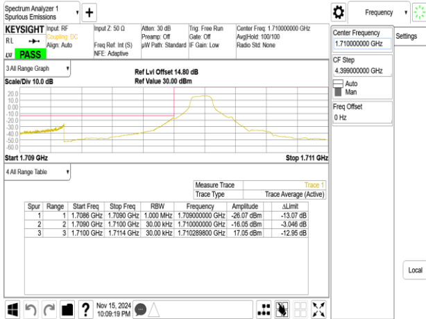
Band4_1.4MHz_QPSK_RB6_0_CH19957
