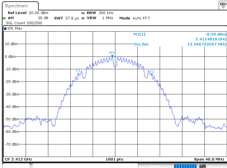
OBW NVNT 802.11b 2412MHz Ant 1
