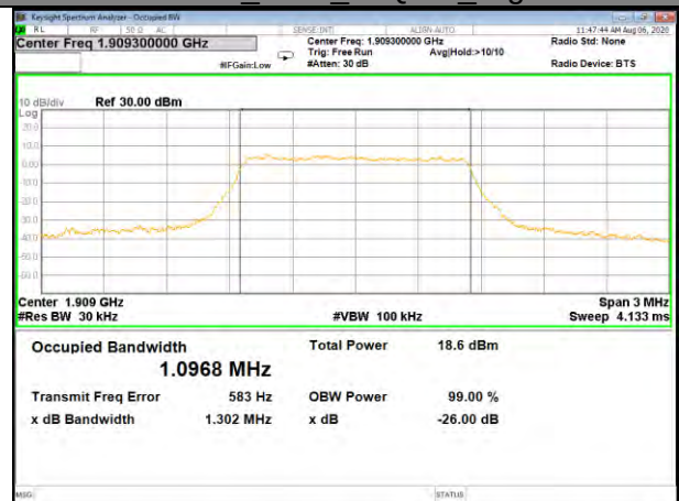
Band2_1.4M_16QAM_High
