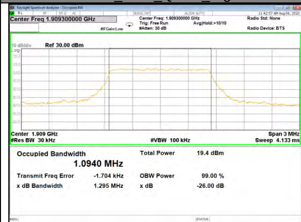
Band2_1.4M_QPSK_High
