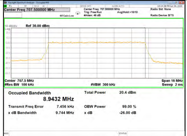
Band12_10M_QPSK_Middle
