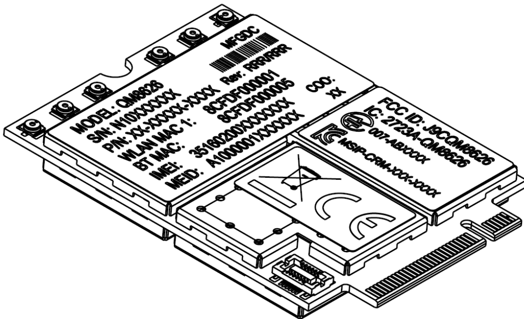
Figure 1-2 QM8626 FCC/IC label placement
