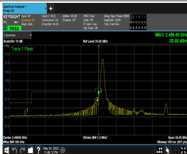
Band41-20MHz-QPSK-39750-1RB#99
