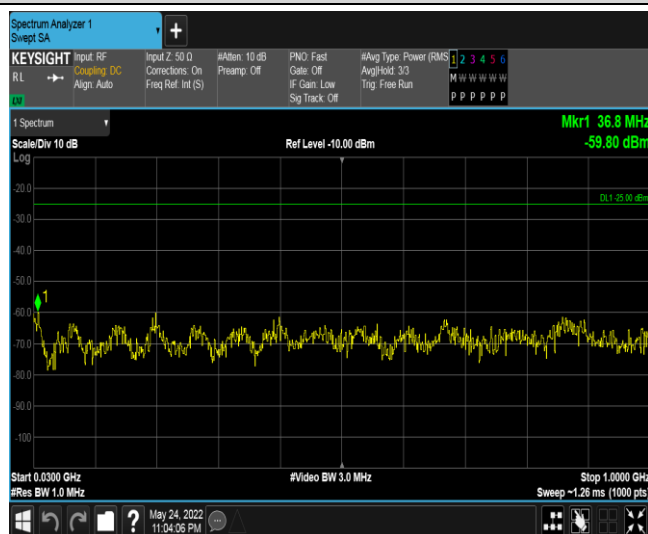
Band41-15MHz-QPSK-40620-1RB#0-Range1:30~1000MHz
