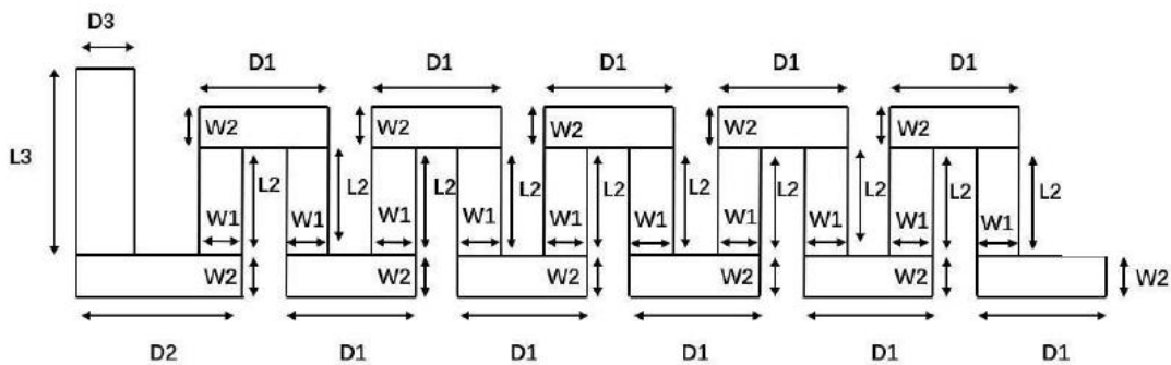
Antenna Dimensions
