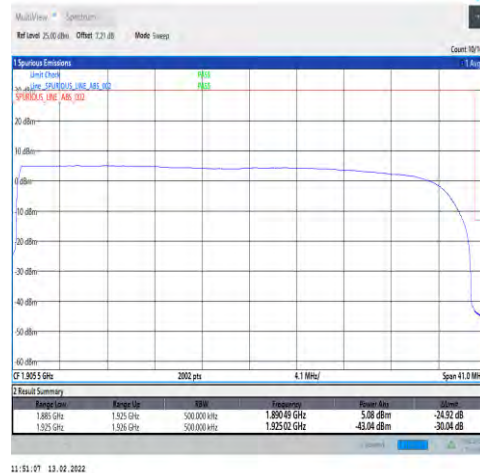
1-N25-15-40-H-6-CP-QPSK-Outer_Full-216@0-Ant1-seegraph-PASS-see graph
