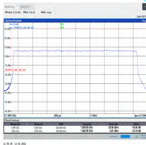
1-N25-15-20-L-3-DFT-PI2BPSK-Outer_Full-100@0-Ant1-seegraph-PASS-see graph
