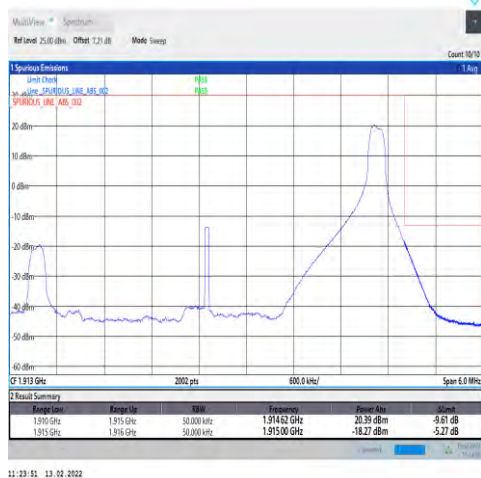
1-N25-15-5-H-2-DFT-PI2BPSK-Edge_1RB_Right-1@24-Ant1-seegraph-PASS-see graph
