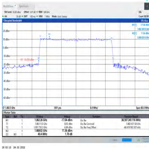
1-N25-PC3-15-40-M-8-CP-64QAM-Outer_Full-216@0-Ant1-38.597-40.400-≤40-PASS
