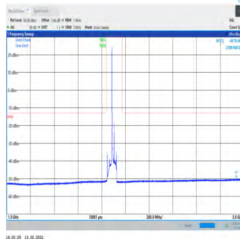
1-N25-15-40-H-1-DFT-PI2BPSK-Inner_1RB_ Left-1@1-1000-3000-Ant1--49.78--13-PASS
