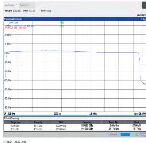
1-N25-PC3-15-25-H-6-CP-QPSK-Outer_Full-133@0-Ant1-seegraph-PASS-see graph
