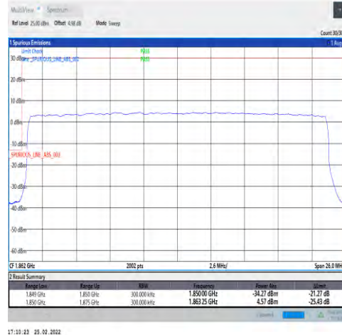
1-N25-PC3-15-25-L-3-DFT-PI2BPSK-Outer_Full-128@0-Ant1-seegraph-PASS-see graph
