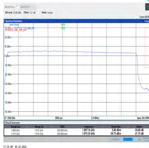
1-N25-PC3-15-25-H-3-DFT-PI2BPSK-Outer_Full-128@0-Ant1-seegraph-PASS-see graph
