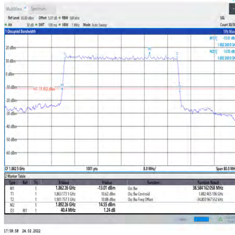
1-N25-PC3-15-40-M-2-DFT-PI2BPSK-Out_F Full-216@0-Ant1-38.584-40.400-≤40-PASS
