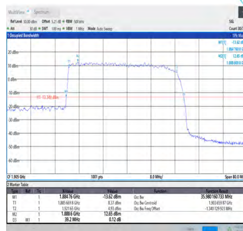
1-N25-PC3-15-40-H-4-DFT-64QAM-Outer_Full-216@0-Ant1-35.98-39.200-≤40-PASS
