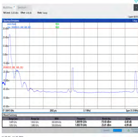
1-N25-15-30-L-4-CP-QPSK-Edge_1RB_Left-1@0-Ant1-seegraph-PASS-see graph
