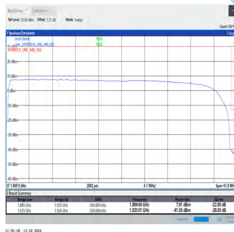
1-N25-15-40-H-3-DFT-PI2BPSK-Outer_Full-216@0-Ant1-seegraph-PASS-see graph
