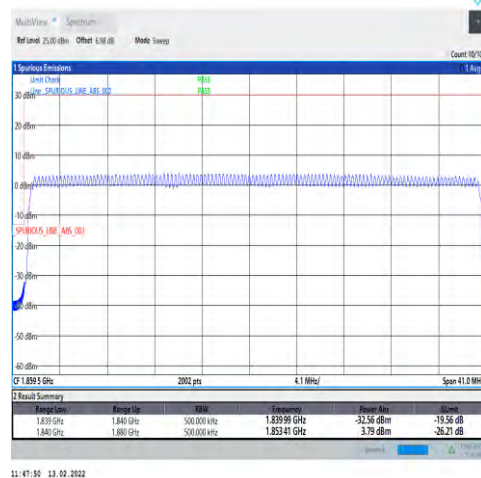
1-N25-15-40-L-3-DFT-PI2BPSK-Outer_Full-216@0-Ant1-seegraph-PASS-see graph
