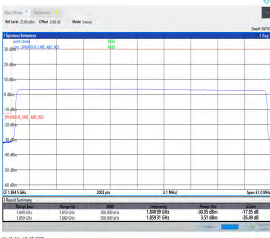
1-N25-15-30-L-6-CP-QPSK-Outer_Full-160@0-Ant1-seegraph-PASS-see graph
