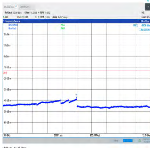
1-N25-15-40-M-1-DFT-PI2BPSK-Inner_1RB_ Left-1@1-3000-12000-Ant1--38.29--13-PASS
