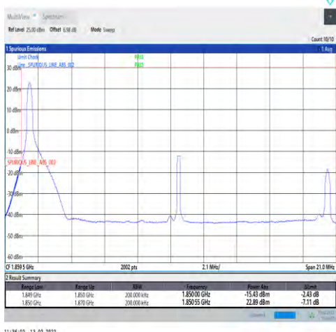
1-N25-15-20-L-4-CP-QPSK-Edge_1RB_Left-1@0-Ant1-seegraph-PASS-see graph
