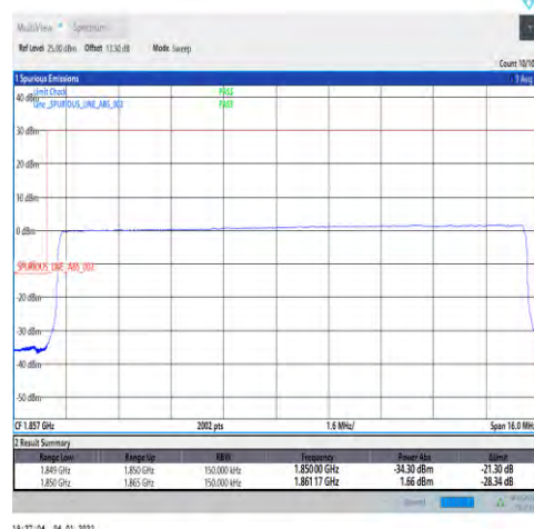
1-N25-15-15-L-6-CP-QPSK-Outer_Full-79@0-Ant1-seegraph-PASS-see graph
