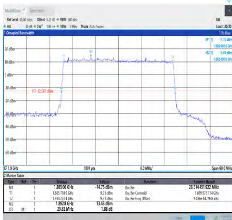
1-N25-PC3-15-30-H-2-DFT-PI2BPSK-Outer_Full-160@0-Ant1-28.514-29.820-≤30-PASS
