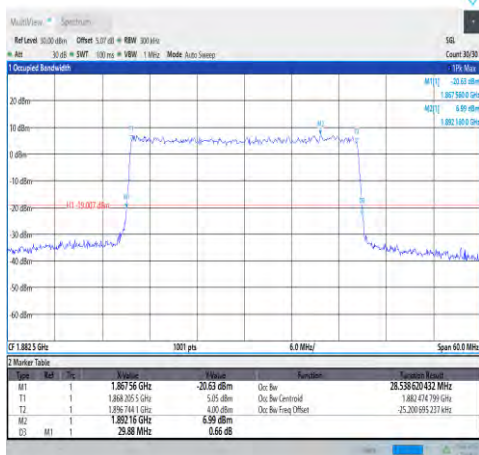
1-N25-PC3-15-30-M-9-CP-256QAM-Outer_Full-160@0-Ant1-28.539-29.880-≤30-PASS
