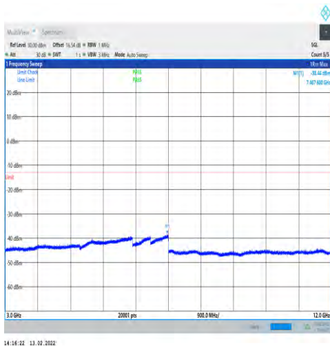
1-N25-15-40-L-1-DFT-PI2BPSK-Inner_1RB_ Left-1@1-3000-12000-Ant1--38.44--13-PASS
