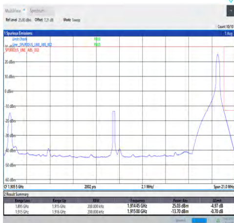
1-N25-15-20-H-2-DFT-PI2BPSK-Edge_1RB_Right-1@105-Ant1-seegraph-PASS-see graph
