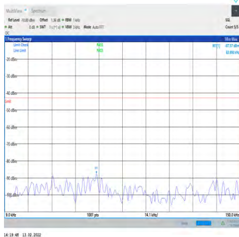
1-N25-15-40-H-1-DFT-PI2BPSK-Inner_1RB_ Left-1@1-0.009-0.15-Ant1--87.57--43-PASS
