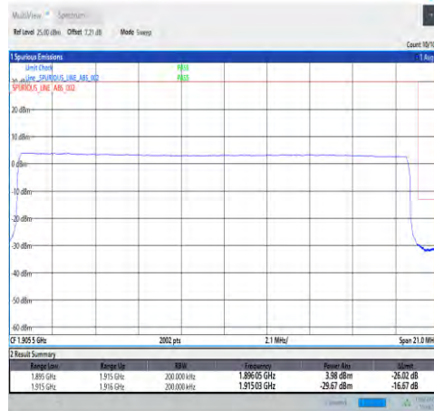
1-N25-15-20-H-6-CP-QPSK-Outer_Full-106@0-Ant1-seegraph-PASS-see graph
