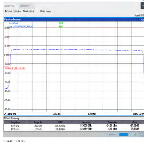
1-N25-15-30-L-3-DFT-PI2BPSK-Outer_Full-160@0-Ant1-seegraph-PASS-see graph
