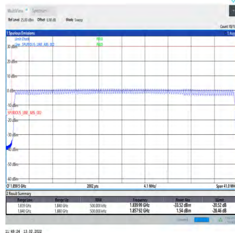
1-N25-15-40-L-6-CP-QPSK-Outer_Full-216@0-Ant1-seegraph-PASS-see graph
