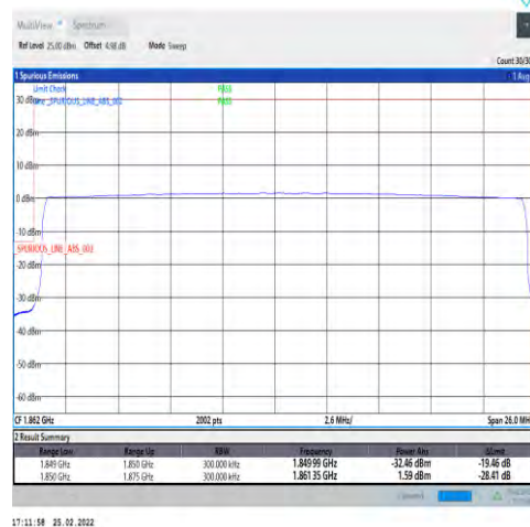
1-N25-PC3-15-25-L-6-CP-QPSK-Outer_Full-133@0-Ant1-seegraph-PASS-see graph
