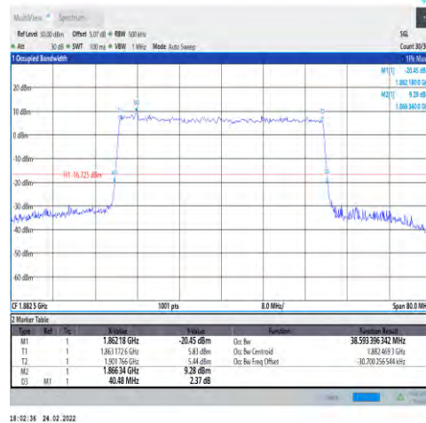
1-N25-PC3-15-40-M-9-CP-256QAM-Outer_Full-216@0-Ant1-38.593-40.480-≤40-PASS
