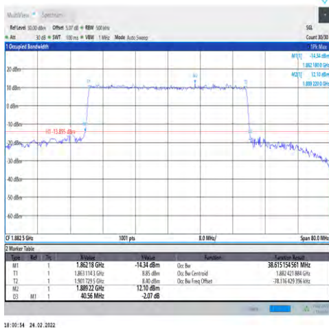
1-N25-PC3-15-40-M-6-CP-QPSK-Outer_Full-216@0-Ant1-38.615-40.560-≤40-PASS
