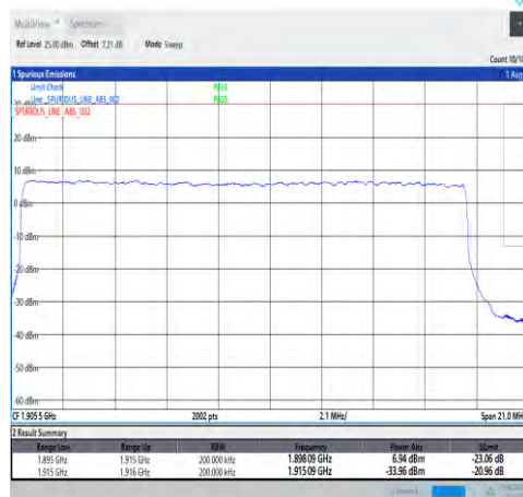
1-N25-15-20-H-3-DFT-PI2BPSK-Outer_Full-100@0-Ant1-seegraph-PASS-see graph
