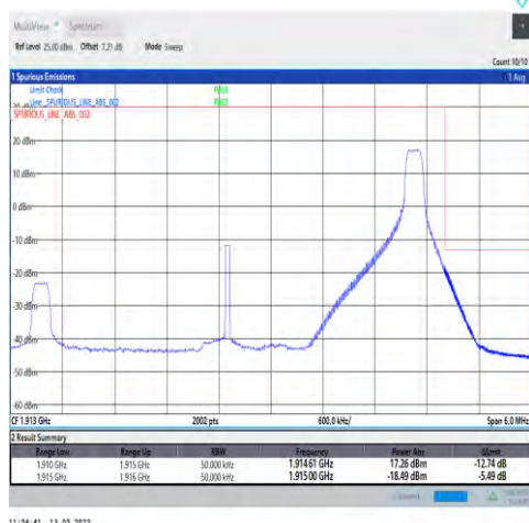
1-N25-15-5-H-5-CP-QPSK-Edge_1RB_Right-1@24-Ant1-seegraph-PASS-see graph
