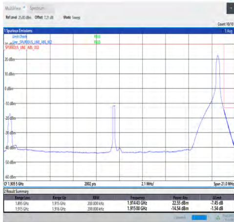
1-N25-15-20-H-5-CP-QPSK-Edge_1RB_Right-1@105-Ant1-seegraph-PASS-see graph
