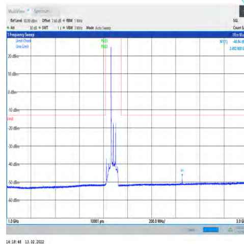
1-N25-15-40-M-1-DFT-PI2BPSK-Inner_1RB_ Left-1@1-1000-3000-Ant1--46.94--13-PASS
