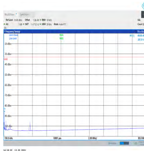
1-N25-15-40-M-1-DFT-PI2BPSK-Inner_1RB_ Left-1@1-0.15-30-Ant1--86.85--33-PASS
