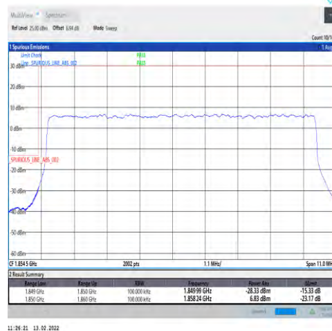
1-N25-15-10-L-3-DFT-PI2BPSK-Outer_Full-50@0-Ant1-seegraph-PASS-see graph
