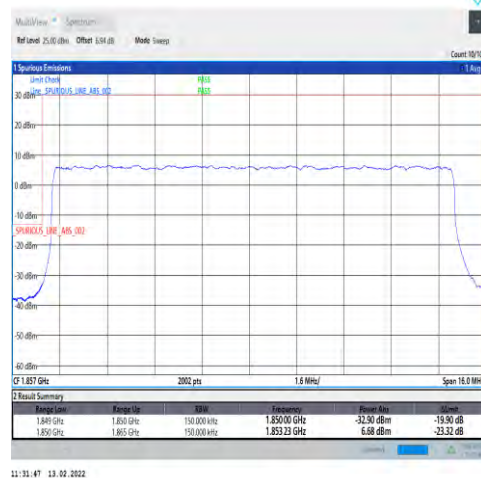
1-N25-15-15-L-3-DFT-PI2BPSK-Outer_Full-75@0-Ant1-seegraph-PASS-see graph
