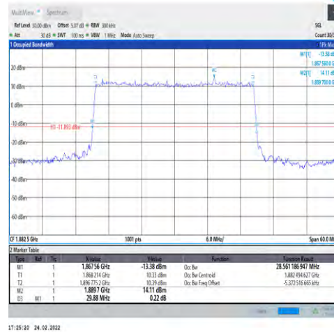
1-N25-PC3-15-30-M-2-DFT-PI2BPSK-Outer_Full-160@0-Ant1-28.561-29.880-≤30-PASS
