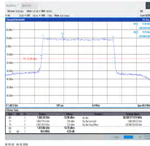
1-N25-PC3-15-40-M-5-DFT-256QAM-Out_F Full-216@0-Ant1-38.589-40.400-≤40-PASS
