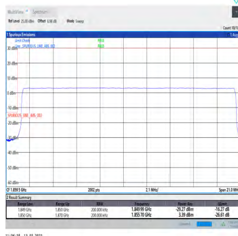
1-N25-15-20-L-6-CP-QPSK-Outer_Full-106@0-Ant1-seegraph-PASS-see graph
