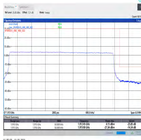
1-N25-15-5-H-6-CP-QPSK-Outer_Full-25@0-Ant1-seegraph-PASS-see graph
