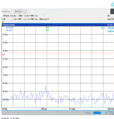
1-N25-15-40-M-1-DFT-PI2BPSK-Inner_1RB_ Left-1@1-0.009-0.15-Ant1--87.94--43-PASS
