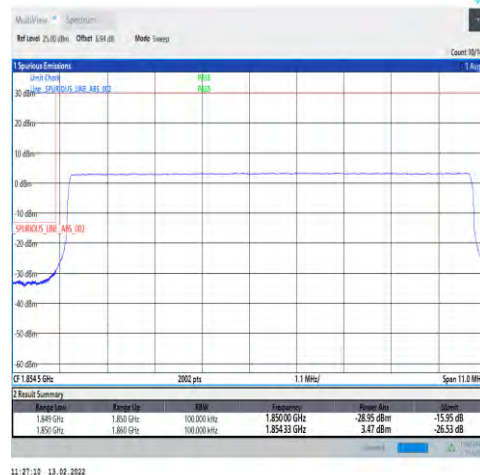
1-N25-15-10-L-6-CP-QPSK-Outer_Full-52@0-Ant1-seegraph-PASS-see graph
