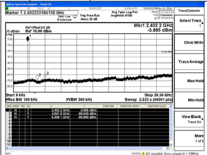
2DH1-Low channel
