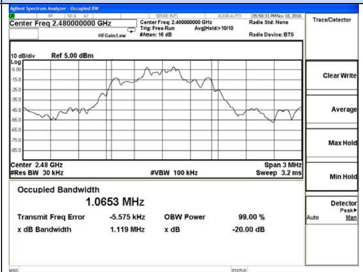
20dB Bandwidth \pi/4 -DQPSK-High channel
