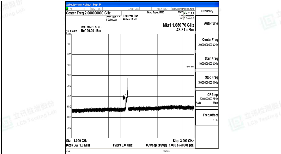
Band25_15MHz_16QAM_26615_1RB#0_1000~3000_1000~3000
