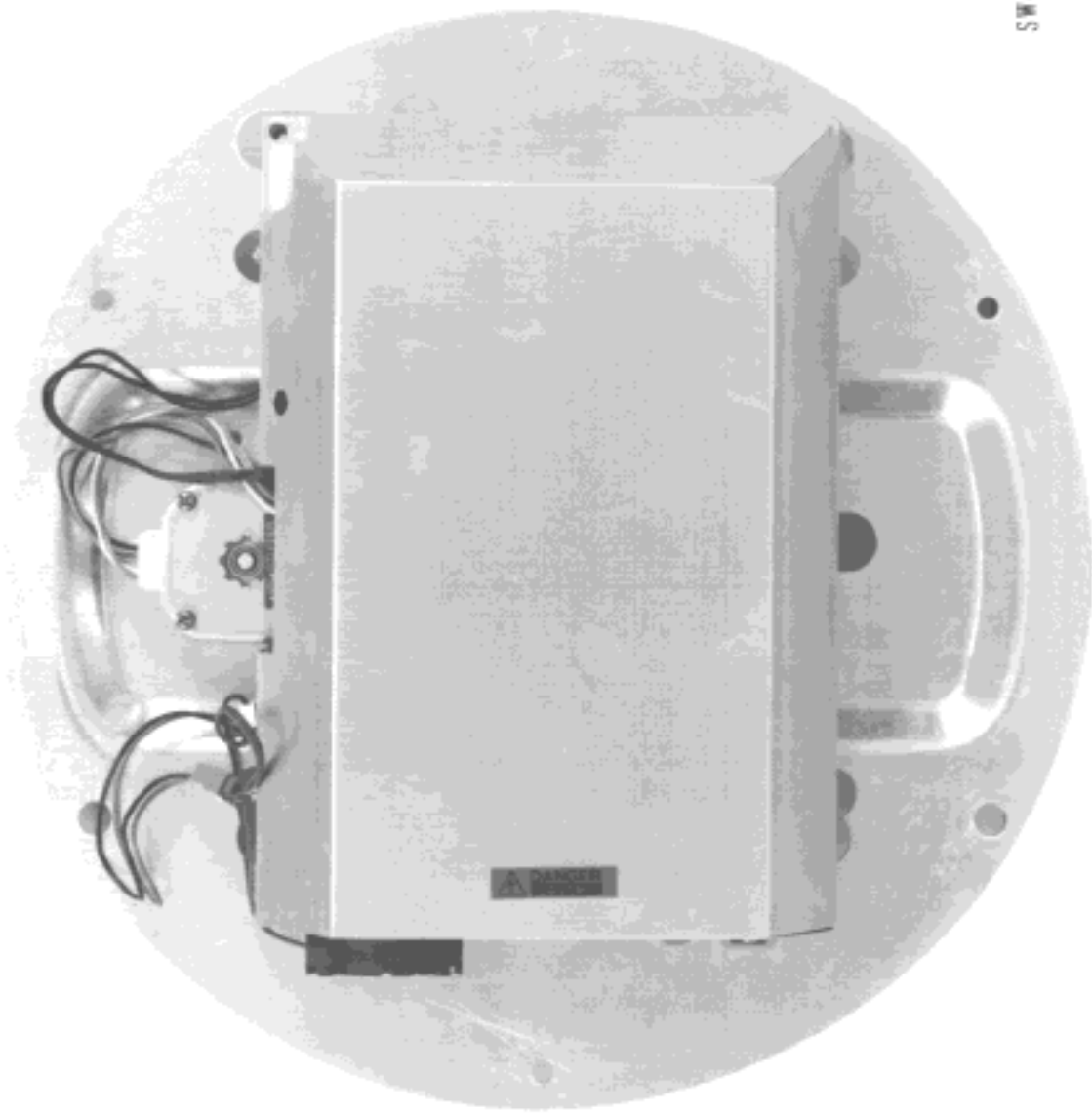
PHOTO.5 T/R UNIT WITH SHIELD COVER OF SCANNER UNIT
