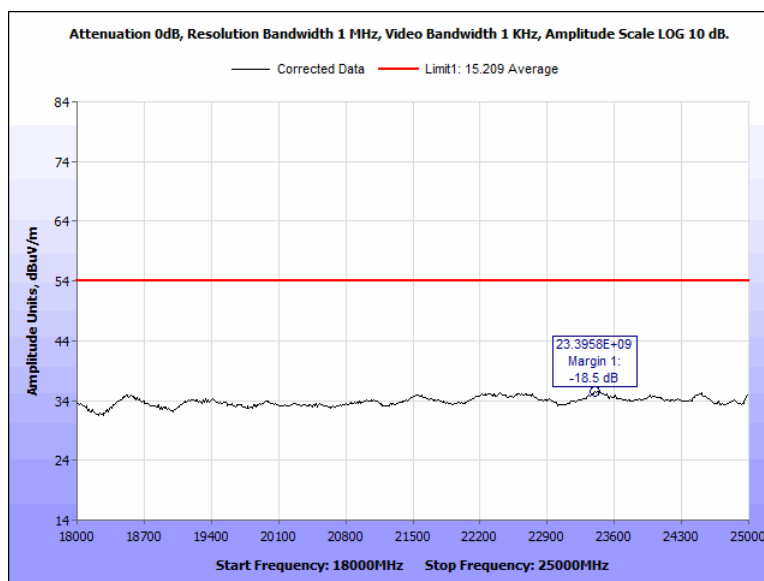
Figure 61: Radiated Spurious Emissions, Pigtail, 2402 MHz, 18 GHz - 25 GHz, Average, Vertical
