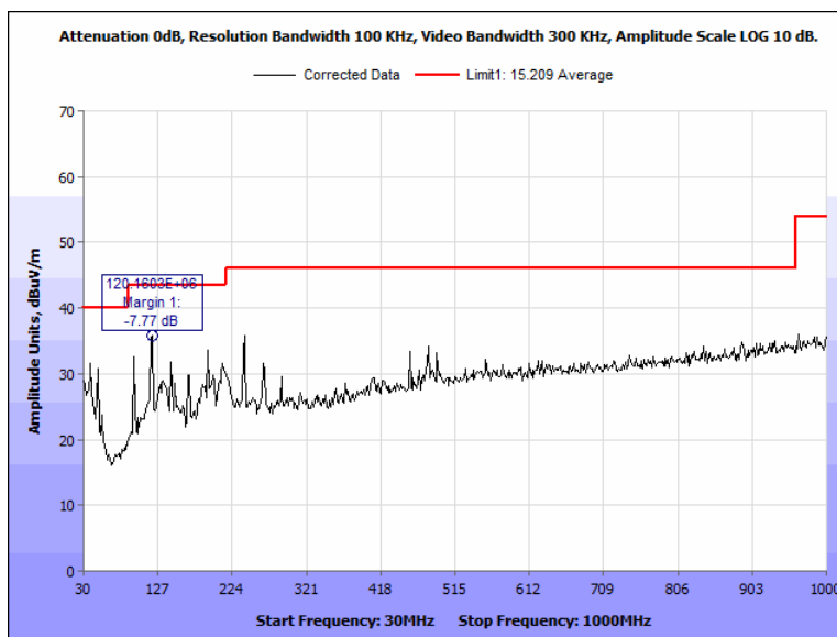
Figure 80: Radiated Spurious Emissions, Terminal, 2402 MHz, 30 MHz - 1000 MHz, Horizontal
