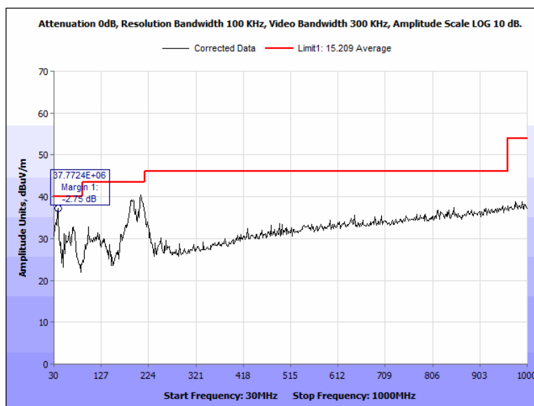
Figure 53: Radiated Spurious Emissions, Pigtail, 2402 MHz, 30 MHz - 1000 MHz, Vertical
