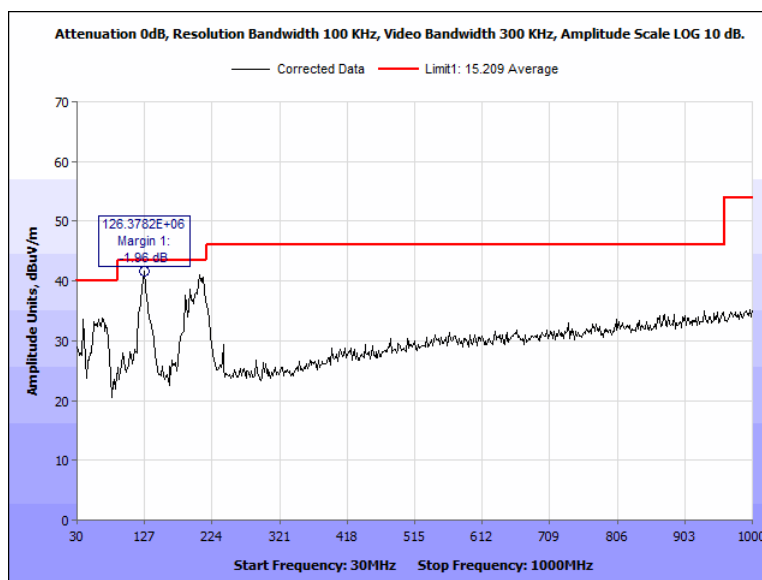
Figure 93: Radiated Spurious Emissions, Terminal, 2442 MHz, 30 MHz - 1000 MHz, Vertical
