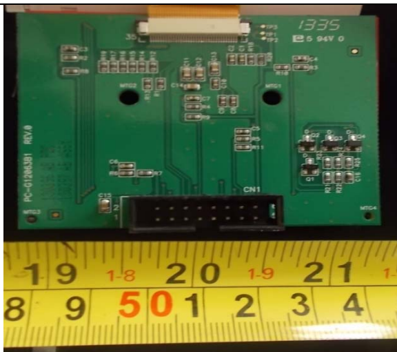
Main PCBA Board - Top View
