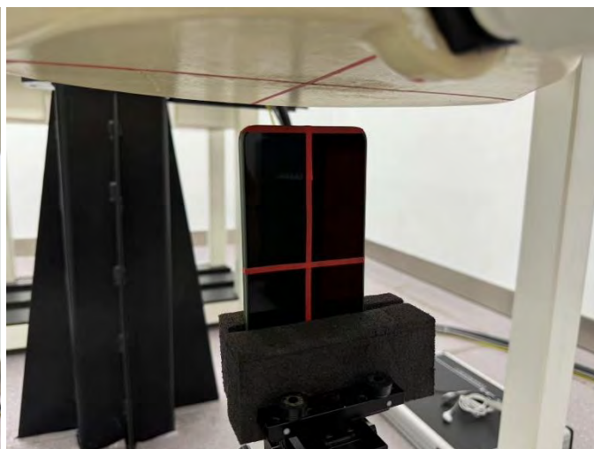
Top Side of EUT with 2.0 cm Gap (Body-Worn Mode)
