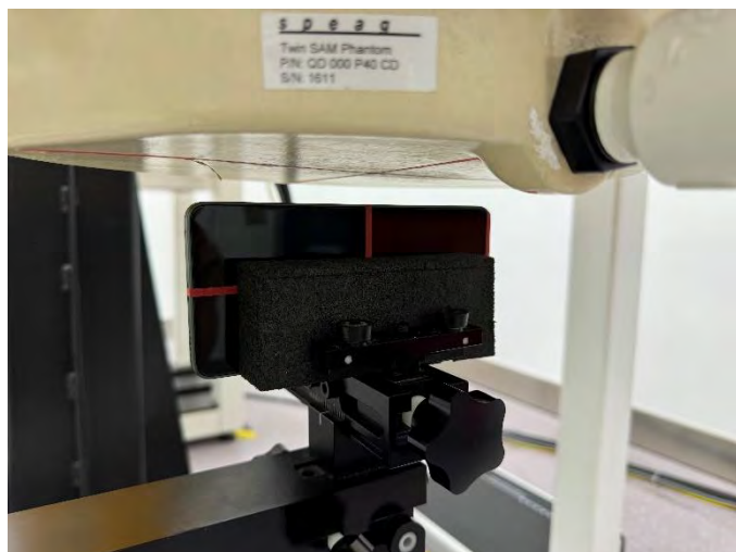
Left Side of EUT with 1.5 cm Gap (Body-Worn Mode)
