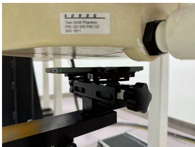
Front Face of EUT with 2.0 cm Gap (Body-Worn Mode)
