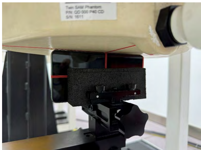
Left Side of EUT with 0 cm Gap (Limbs Mode)
