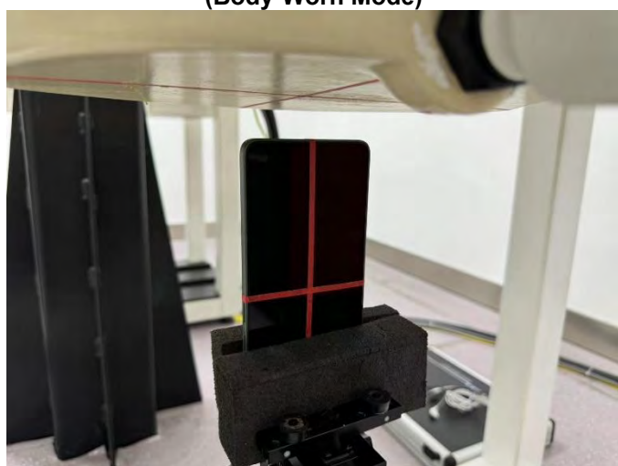
Bottom Side of EUT with 2.0 cm Gap (Body-Worn Mode)
