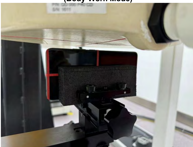
Right Side of EUT with 1 cm Gap (Body-Worn Mode)
