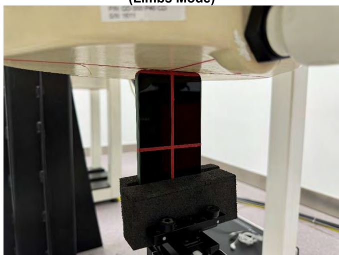
Top Side of EUT with 0 cm Gap (Limbs Mode)
