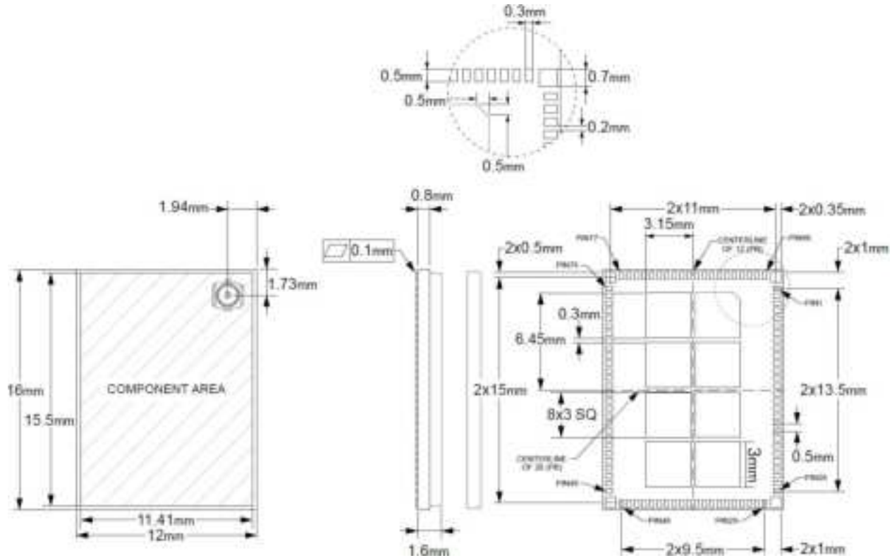
Figure 10: EMQ100-5U Dimension
