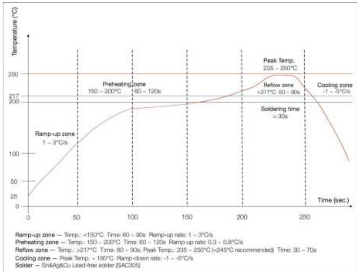
Figure 16: Soldering Guideline
