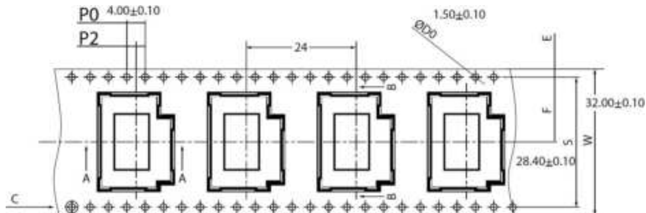
Figure 16: Module Packaging
