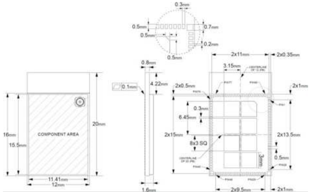
Figure 12: EMQ100-5B Dimension
