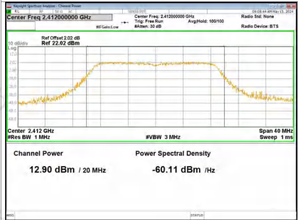
Peak Power NVNT n20 2412MHz Ant2
