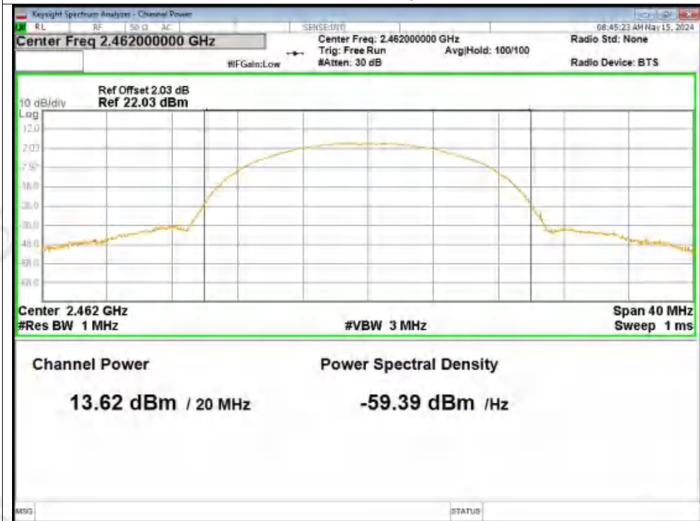
Peak Power NVNT b 2462MHz Ant2
