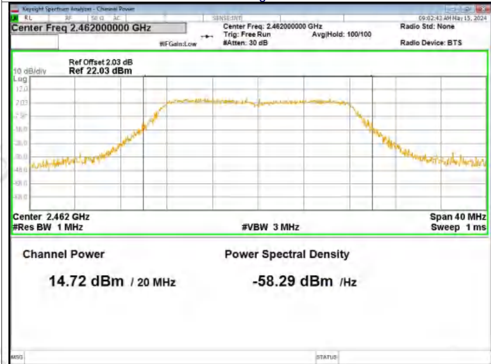
Peak Power NVNT g 2462MHz Ant2
