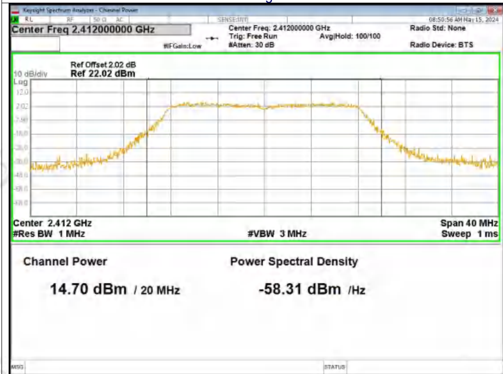
Peak Power NVNT g 2412MHz Ant2
