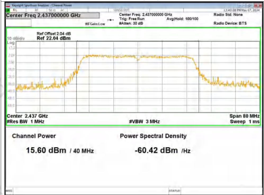
Peak Power NVNT n40 2437MHz Ant1
