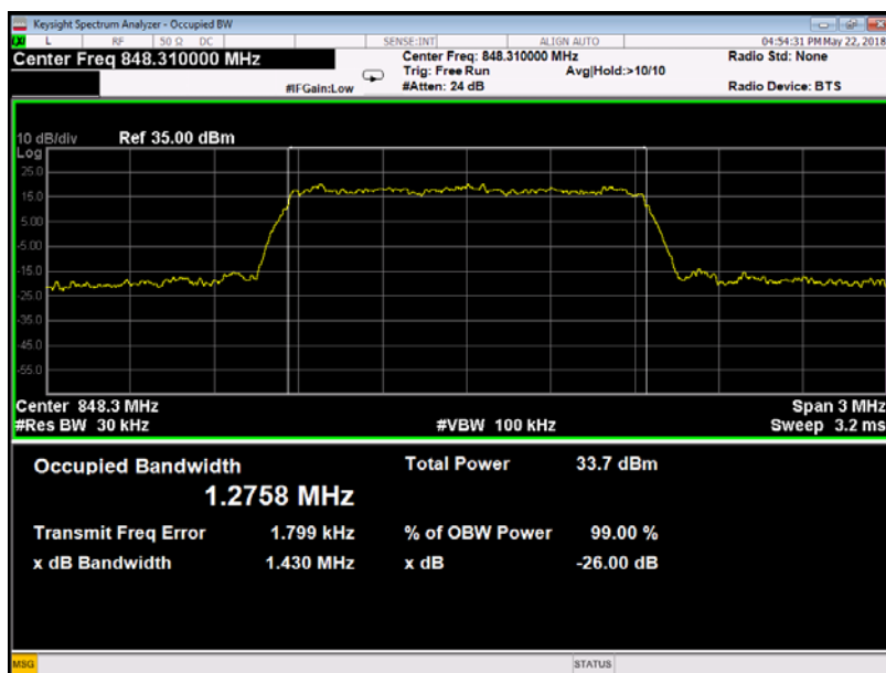
99% &amp; 26dB Occupied Bandwidth Plot on Channel 777
