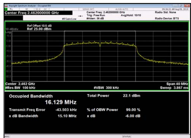
6dB Bandwidth-802.11g,2462MHz,Ant1
