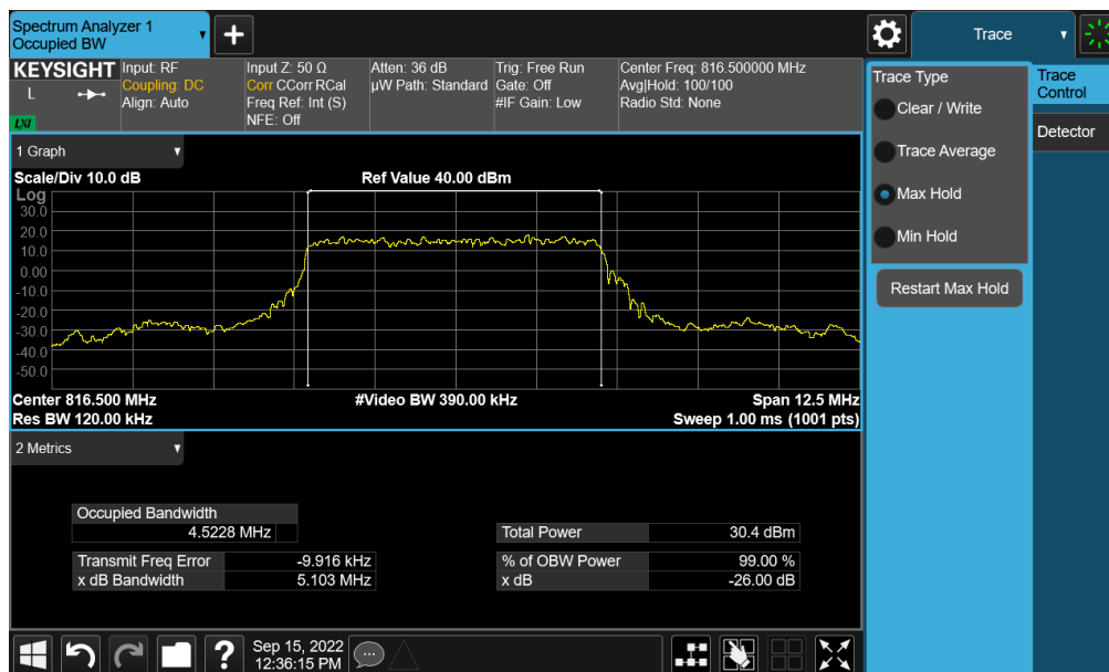
Plot 7-24. Occupied Bandwidth Plot (NR Band n26- 5MHz \pi/2 BPSK - Full RB)
