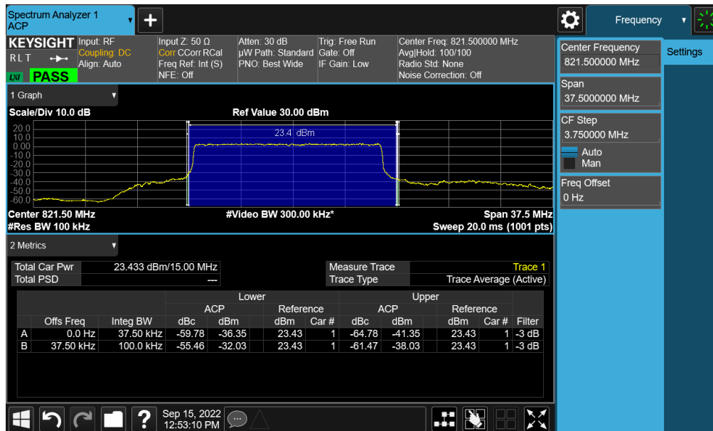
Plot 7-53. Channel Edge Plot (NR Band n26 - 15MHz DFT-s \pi/2 BPSK - Mid Channel)
