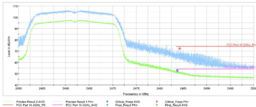
Fig. 7.6 Transmitter Spurious Emission - Radiated (Power): 802.11n-HT20, ch11, 2.45 GHz - 2.50GHz
