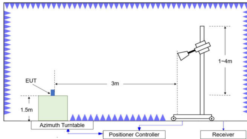
Figure A.2.3. Test Site Diagram (1GHz-40GHz)
