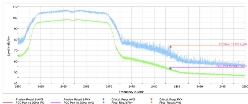
Fig. 7.4 Transmitter Spurious Emission - Radiated (Power): 802.11g, ch11, 2.45 GHz - 2.50GHz
