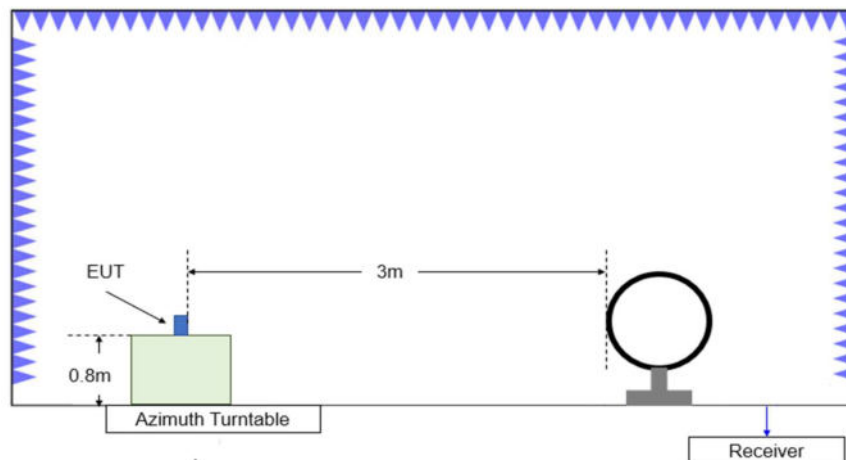
Figure A.2.1. Test Site Diagram (9kHz-30MHz)
