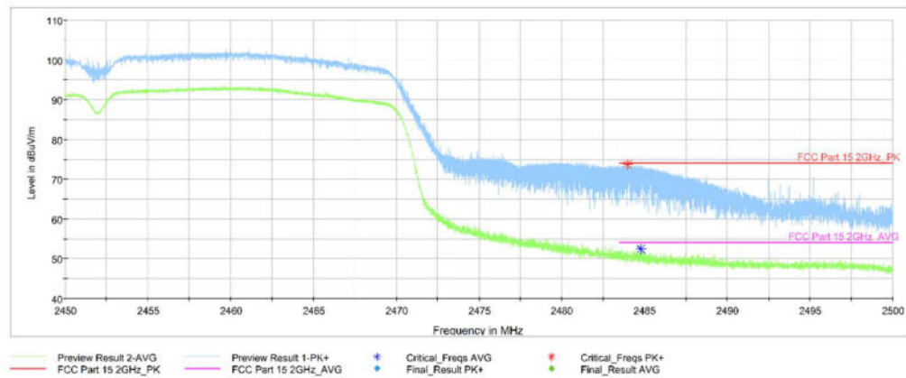
Fig. 7.8 Transmitter Spurious Emission - Radiated (Power): 802.11n-HT40, ch9, 2.45 GHz - 2.50GHz
