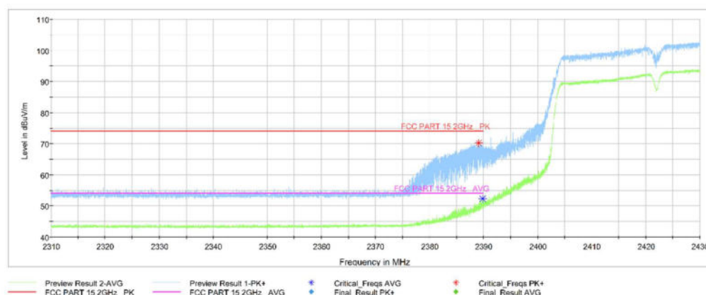
Fig. 7.7 Transmitter Spurious Emission - Radiated (Power): 802.11n-HT40, ch3, 2.31 GHz - 2.43GHz
