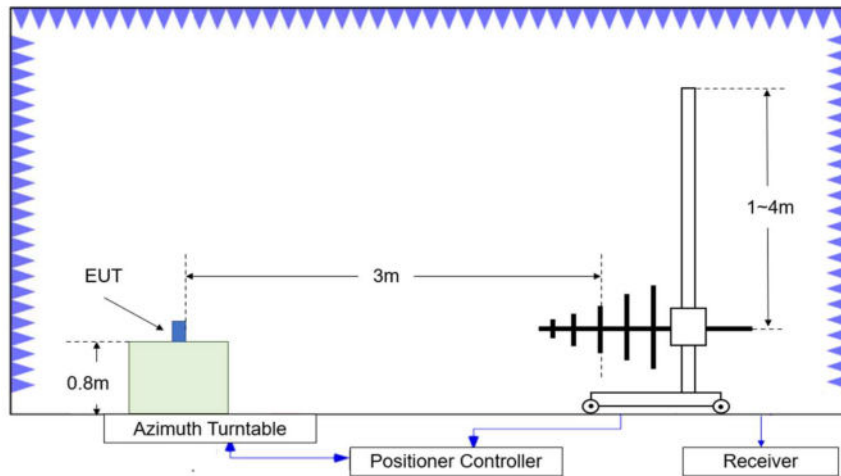
Figure A.2.2. Test Site Diagram (30MHz-1GHz)
