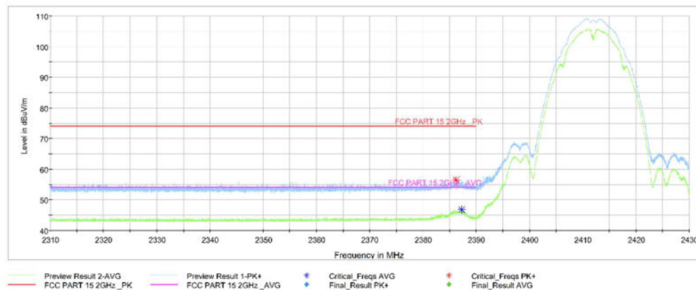
Fig. 7.1 Transmitter Spurious Emission - Radiated (Power): 802.11b, ch1, 2.31 GHz – 2.43GHz
