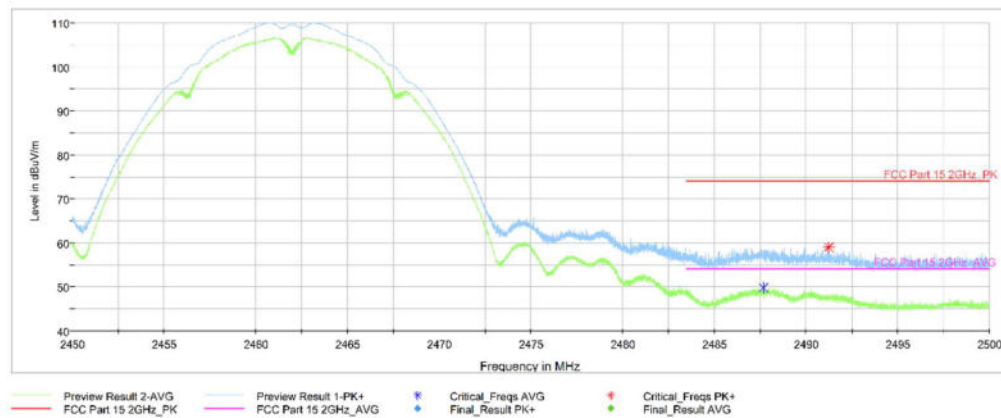
Fig. 7.2 Transmitter Spurious Emission - Radiated (Power): 802.11b, ch11, 2.45 GHz - 2.50GHz
