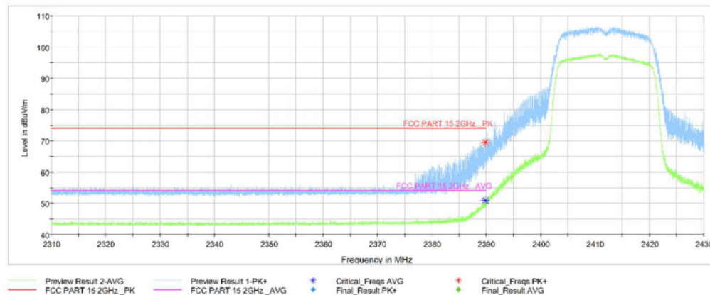
Fig. 7.5 Transmitter Spurious Emission - Radiated (Power): 802.11n-HT20, ch1, 2.31 GHz - 2.43GHz
