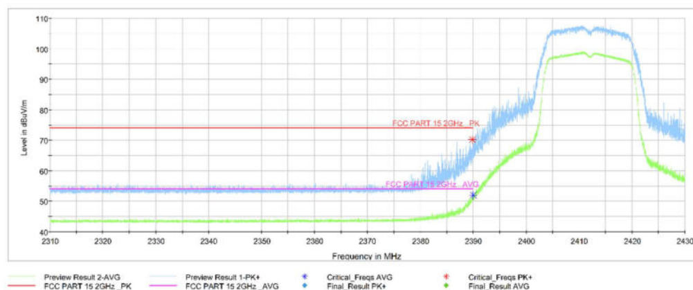
Fig. 7.3 Transmitter Spurious Emission - Radiated (Power): 802.11g, ch1, 2.31 GHz - 2.43GHz
