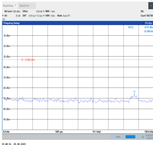
Band42_20MHz_QPSK_42990_1RB#0_0.009~0.15_0.009~0.15
