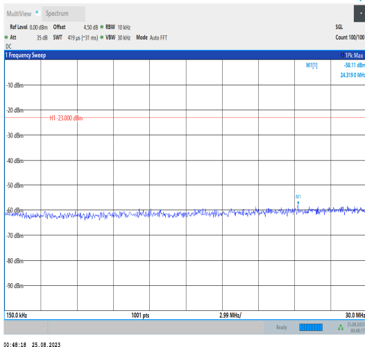
Band42_20MHz_QPSK_42590_1RB#0_0.15~30_0.15~30
