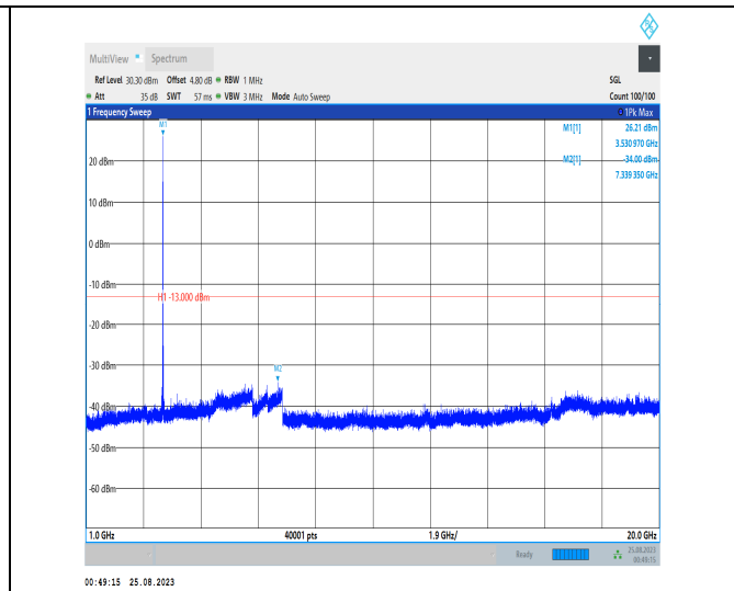
Band42_20MHz_QPSK_42990_1RB#0_1000~20000_1000~20000
