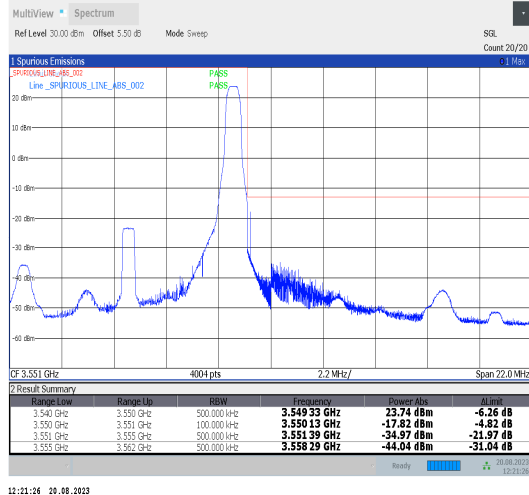
Band42_10MHz_QPSK_43040_1RB#49
