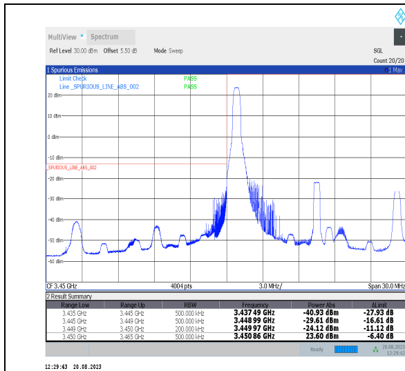
Band42_15MHz_QPSK_42165_1RB#0
