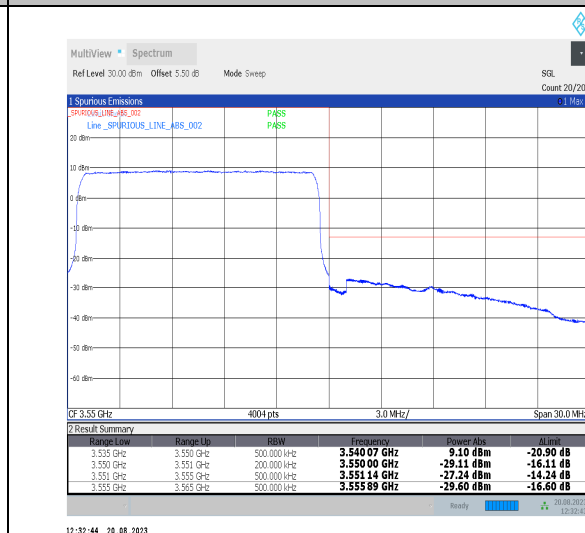
Band42_15MHz_QPSK_43015_75RB#0
