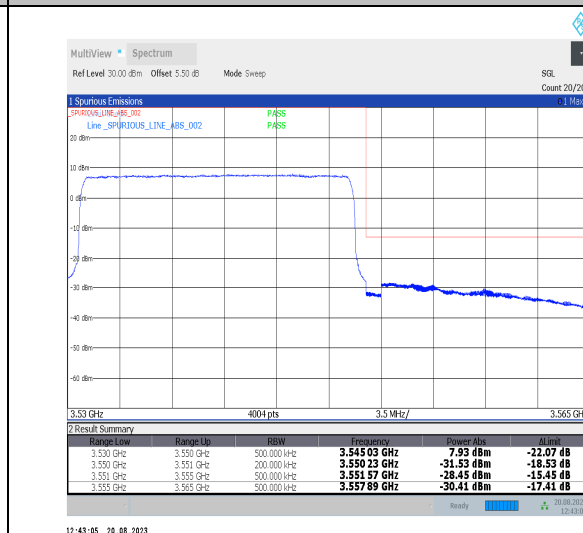
Band42_20MHz_QPSK_42990_100RB#0
