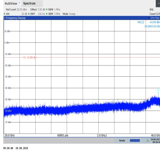
Band42_20MHz_QPSK_42590_1RB#0_20000~40000_20000~40000
