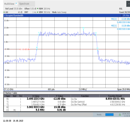
Band42-10MHz-16QAM-42590-50RB#0-PASS
