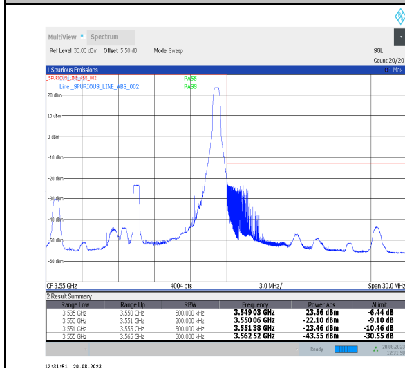
Band42_15MHz_QPSK_43015_1RB#74
