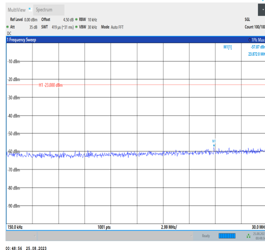
Band42_20MHz_QPSK_42990_1RB#0_0.15~30_0.15~30
