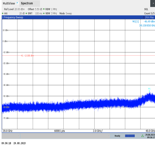
Band42_20MHz_QPSK_42190_1RB#0_20000~40000_20000~40000
