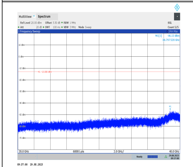
Band42_20MHz_QPSK_42990_1RB#0_20000~40000_20000~40000
