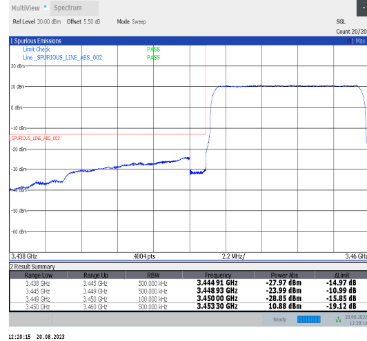
Band42_10MHz_QPSK_42140_50RB#0
