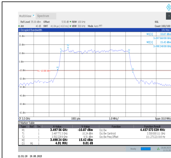
Band42-5MHz-QPSK-42590-25RB#0-PASS
