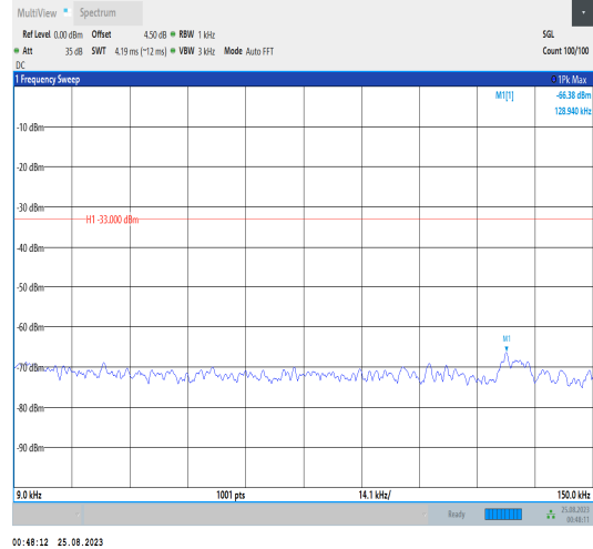
Band42_20MHz_QPSK_42590_1RB#0_0.009~0.15_0.09~0.15
