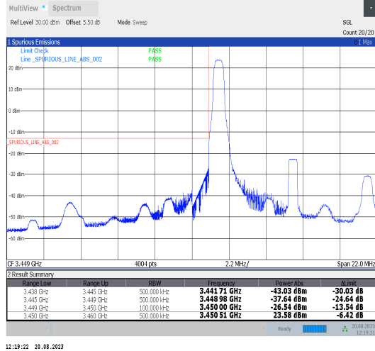
Band42_10MHz_QPSK_42140_1RB#0
