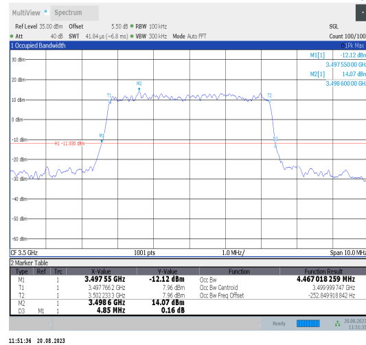
Band42-5MHz-16QAM-42590-25RB#0-PASS
