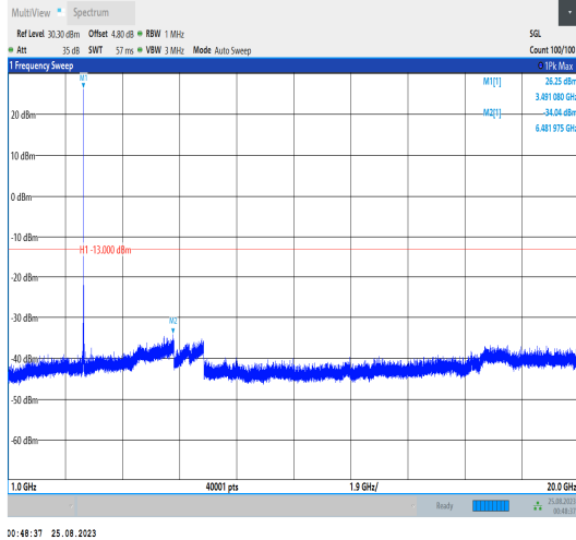
Band42_20MHz_QPSK_42590_1RB#0_1000~20000_1000~20000
