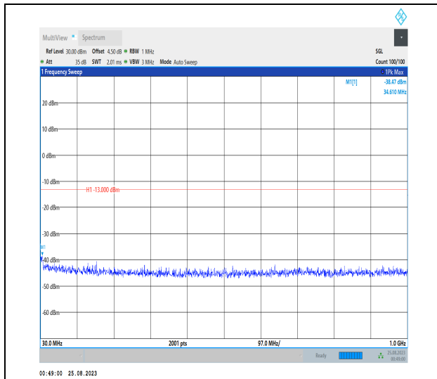
Band42_20MHz_QPSK_42990_1RB#0_30~1000_30~1000
