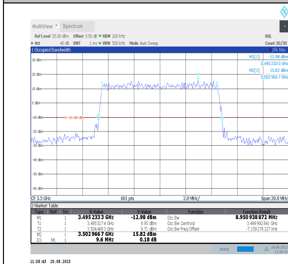
Band42-10MHz-QPSK-42590-50RB#0-PASS
