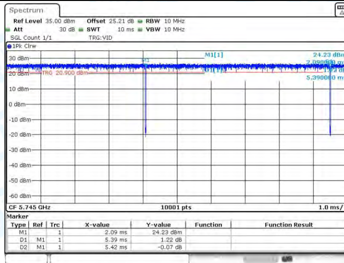
11A_Ant3_5745
