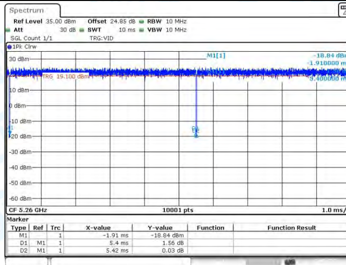
11A_Ant4_5260
