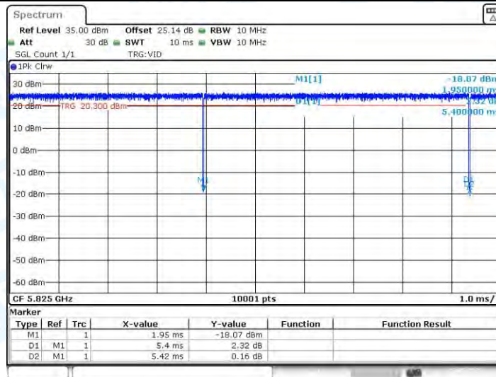
11A_Ant4_5825
