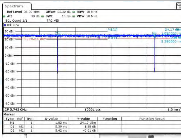
11A_Ant4_5745
