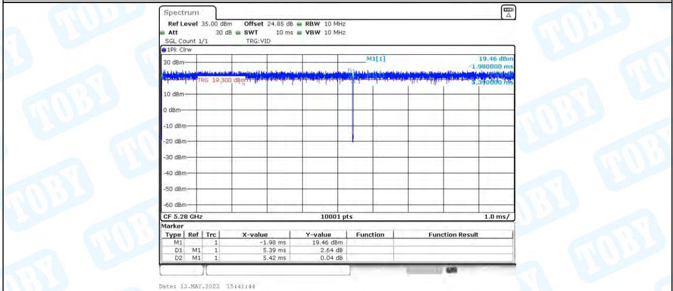
11A_Ant4_5280
