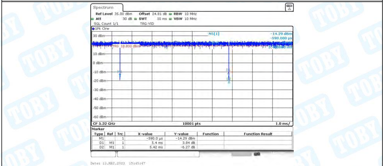
11A_Ant4_5320
