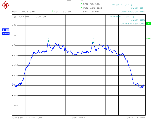
3DH1_High 1.001MHz
