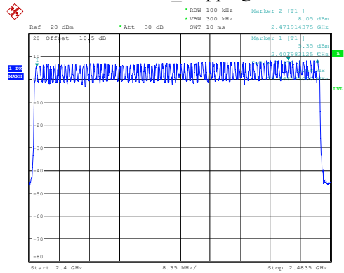
3DH1_Hopping 79
