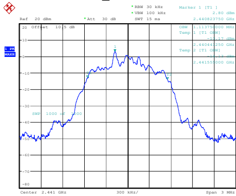
3DH1_Middle 1.114MHz
