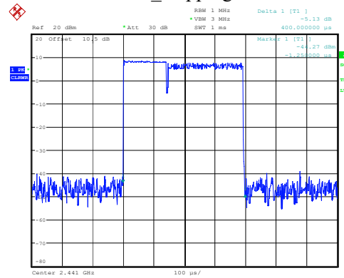
2DH1_Hopping 0.400ms
