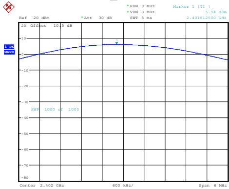
2DH1_Low 5.94dBm
