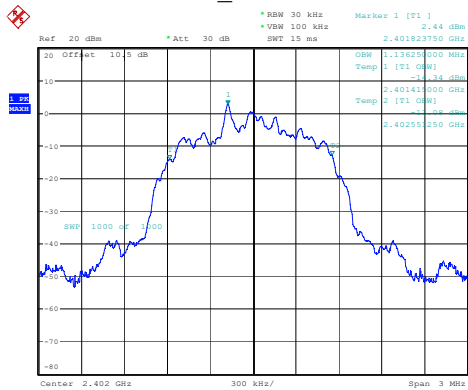
2DH1_Low 1.136MHz
