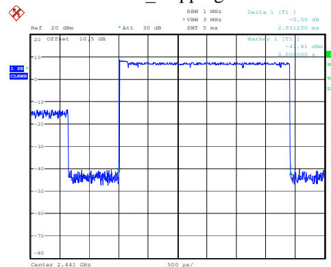
2DH5_Hopping 2.931ms
