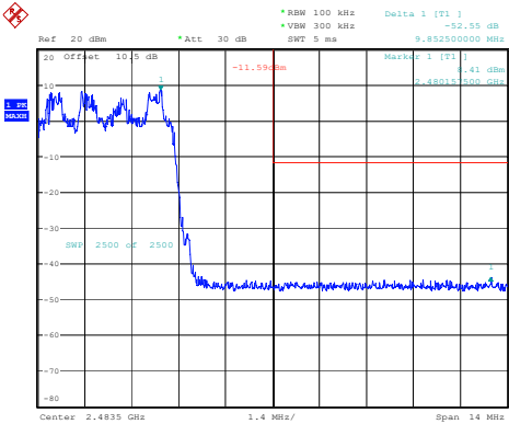
2DH1_Hopping_Upper
