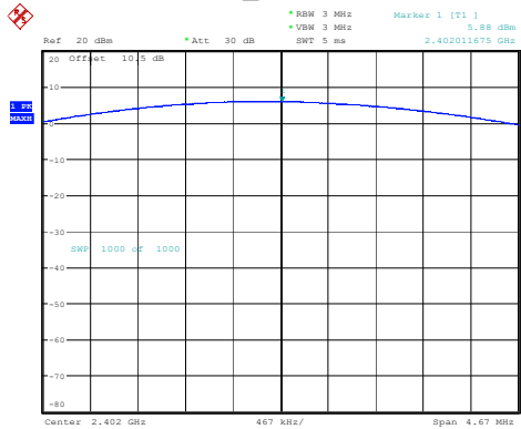
DH1_Low 5.88dBm
