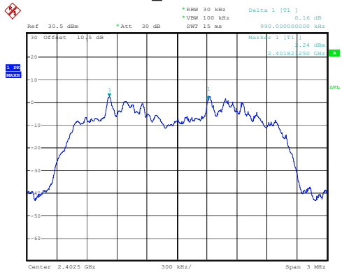
3DH1_Low 0.990MHz
