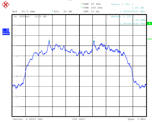
2DH1_Low 1.005MHz
