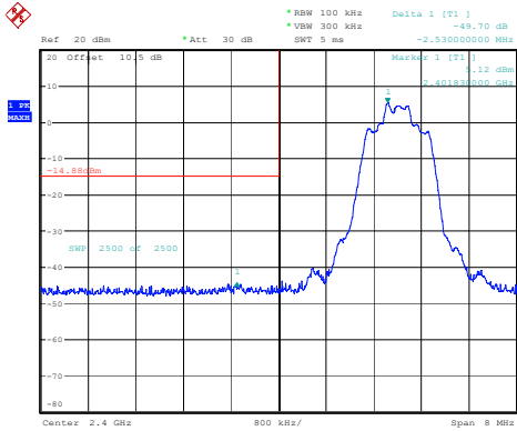
3DH1_Low
