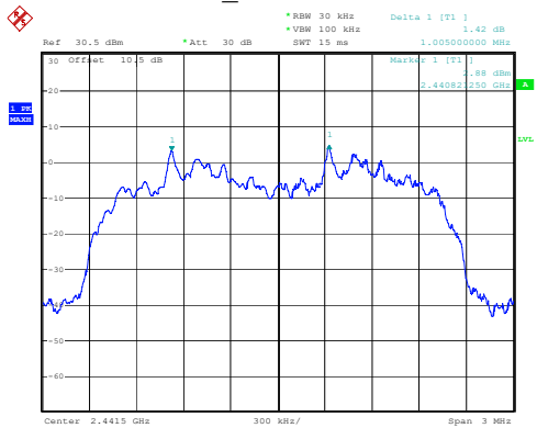
2DH1_Middle 1.005MHz
