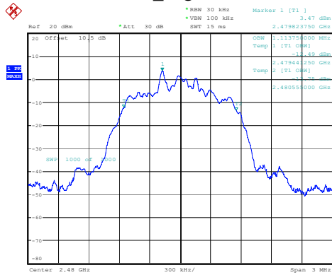
3DH1_High 1.114MHz
