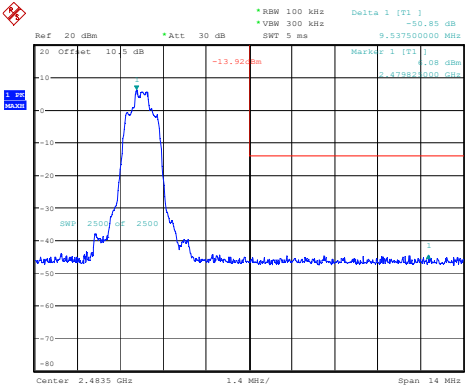
3DH1_High
