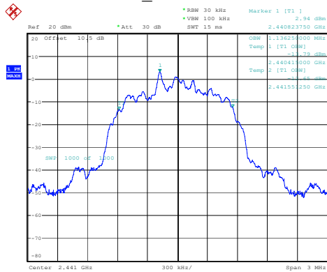
2DH1_Middle 1.136MHz
