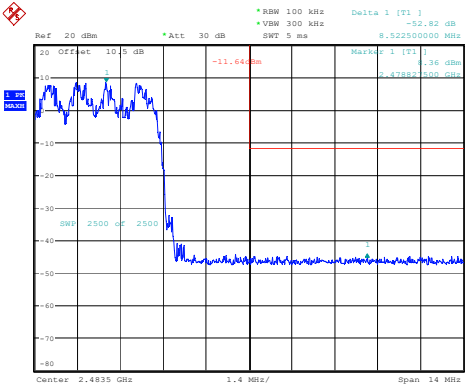
3DH1_Hopping_Upper
