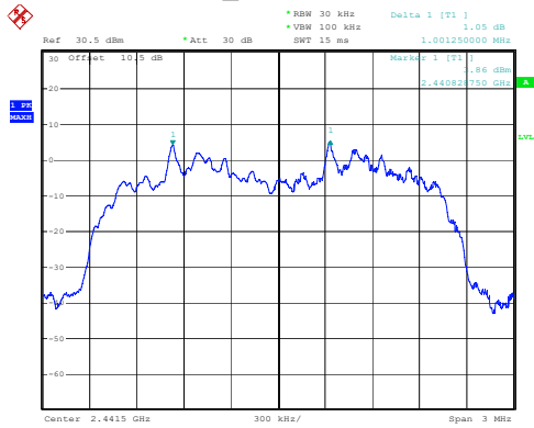
2DH1_Middle 1.001MHz
