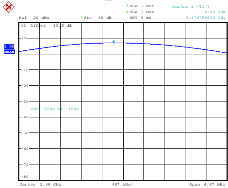
DH1_High 6.86dBm
