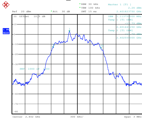
3DH1_Low 1.114MHz
