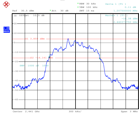
2DH1_Middle 1.208MHz
