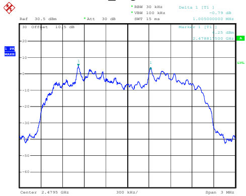
2DH1_High 1.005MHz
