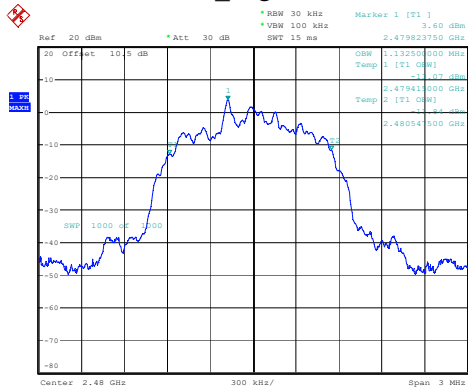
2DH1_High 1.133MHz
