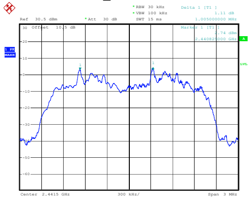
3DH1_Middle 1.005MHz
