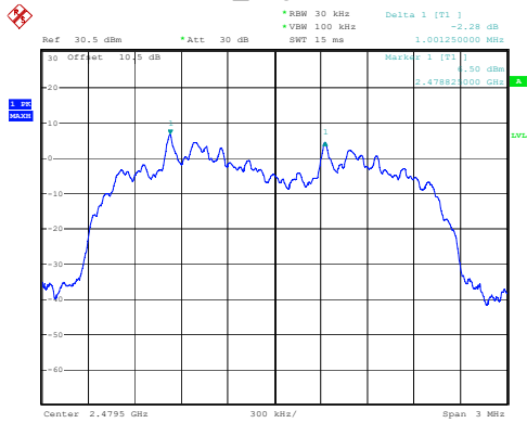
2DH1_High 1.001MHz
