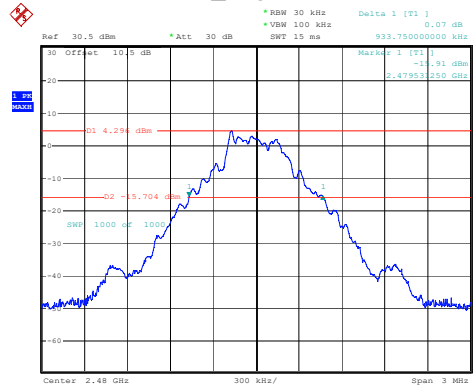
DH1_High 0.934MHz
