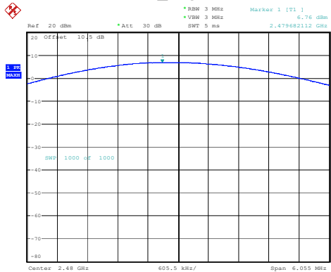
2DH1_High 6.76dBm
