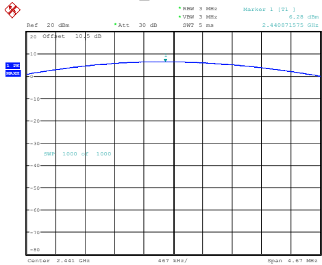
DH1_Middle 6.28dBm
