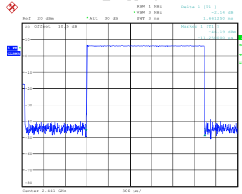
DH3_Hopping 1.661ms
