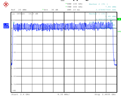
2DH1_Hopping 79
