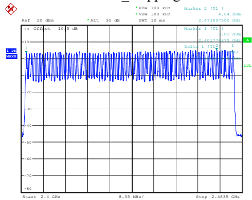
DH1_Hopping 79
