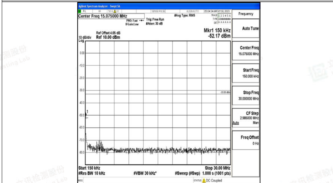
Band2_20MHz_QPSK_18700_1RB#0_0.15~30_0.15~30
